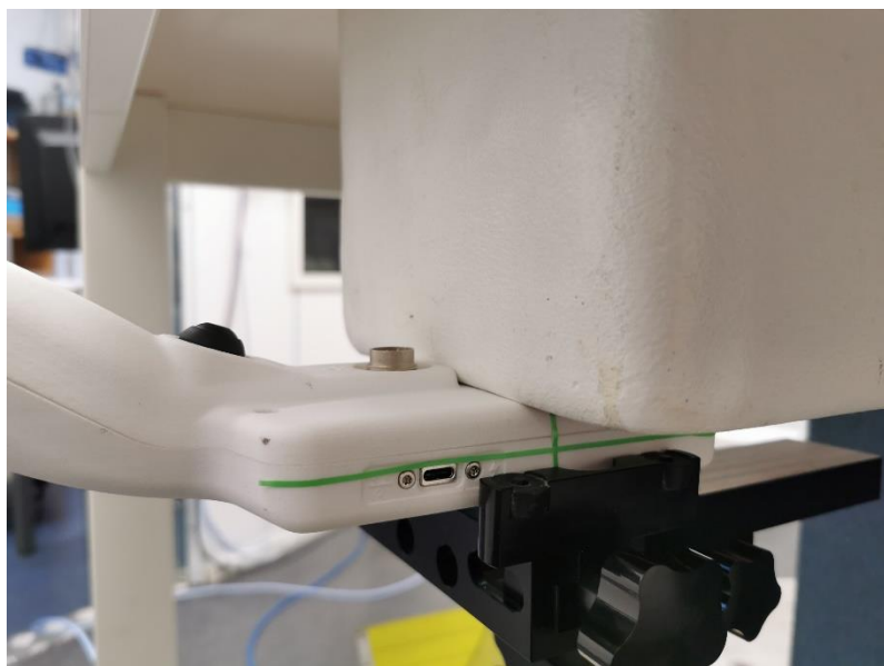
Figure 4. Back side of the DUT, 0mm separation distance
