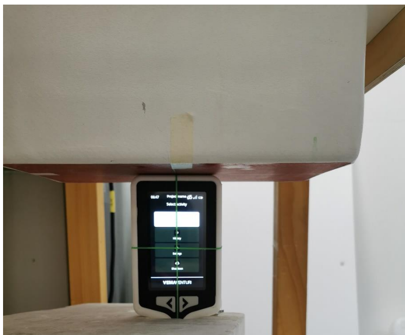
Figure 7. Top side of the DUT, 0mm separation distance
