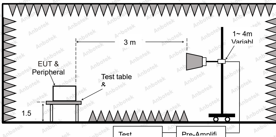
Figure 3. Above 1 GHz
