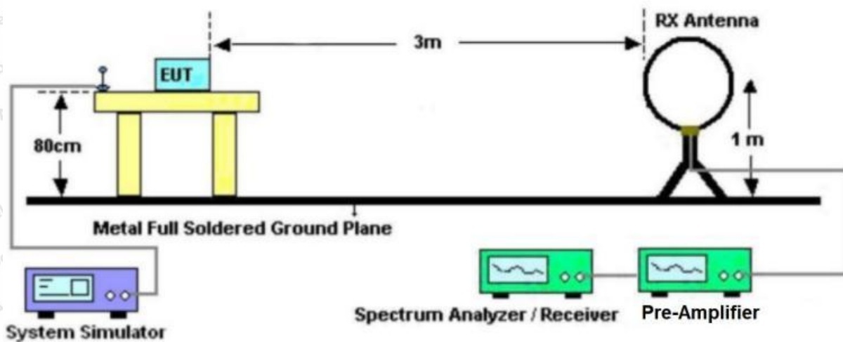
Figure 1. Below 30MHz
