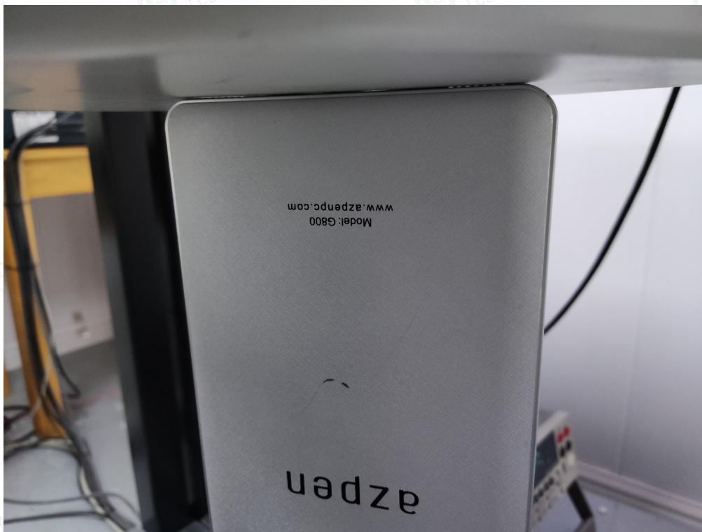
0mm body Vertical-Bottom Side Setup Photo
