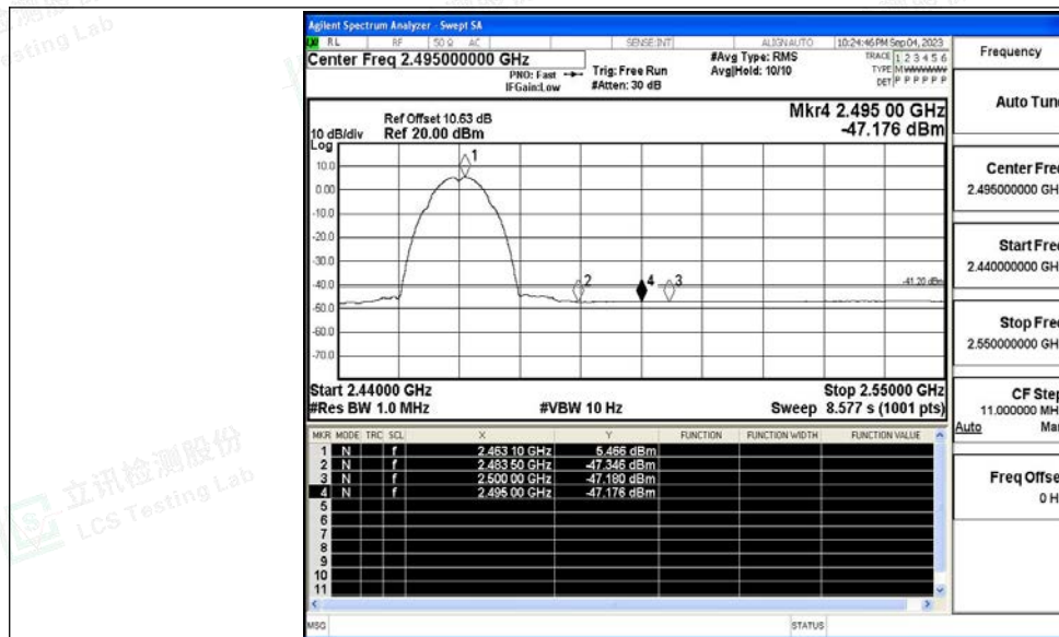
11B_Ant1_High_2462_Peak
