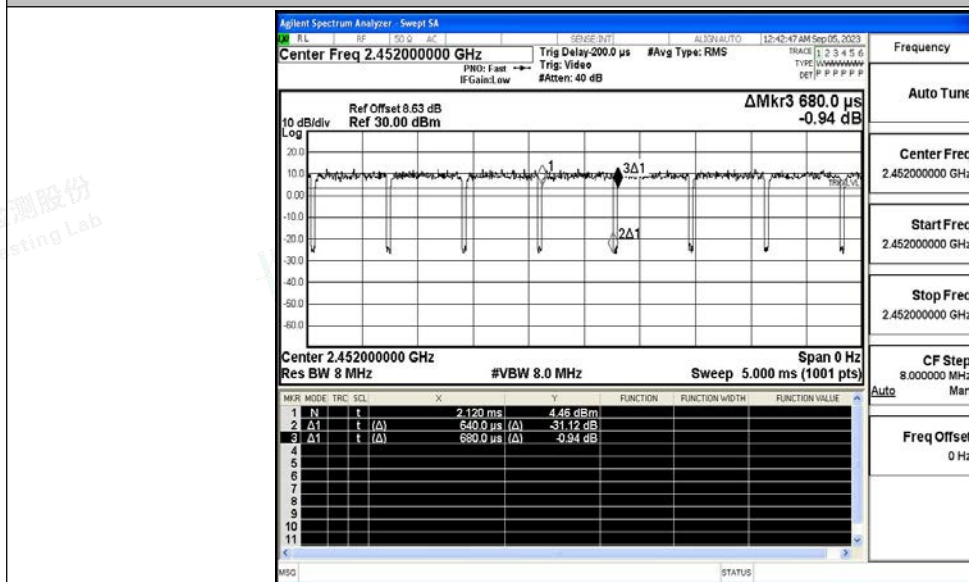
11N40SISO_Ant1_2452
