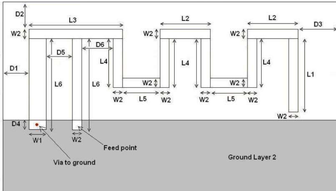
Figure 3: Antenna Dimensions
