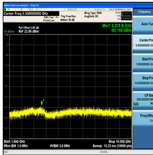
Band12-1.4MHz-16QAM-23017-6RB#0-Range2:1000~10000MHz
