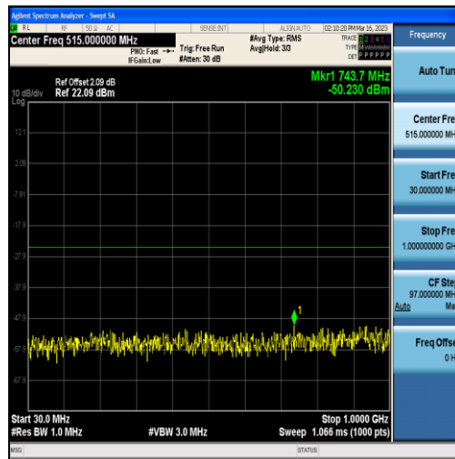
Band7-15MHz-16QAM-20825-75RB#0-Range1:30~1000MHz
