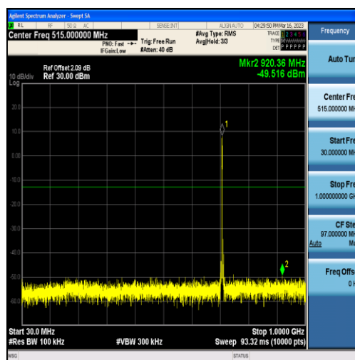
Band12-3MHz-16QAM-23165-15RB#0-Range1:30~1000MHz
