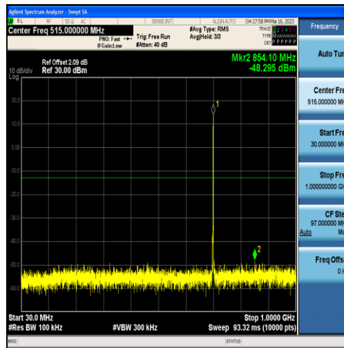
Band12-1.4MHz-16QAM-23095-6RB#0-Range1:30~1000MHz
