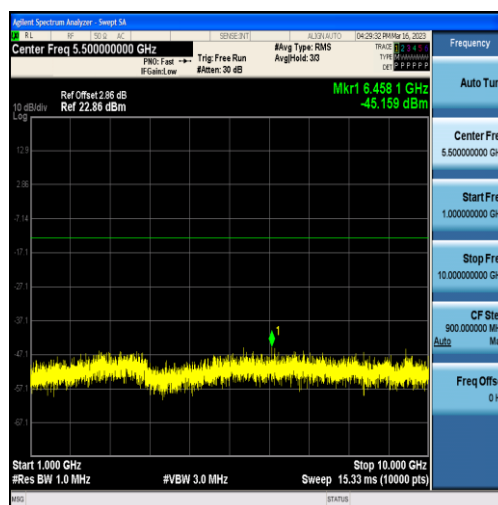
Band12-3MHz-16QAM-23095-15RB#0-Range2:1000~10000MHz
