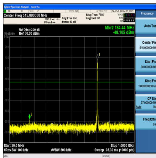
Band12-5MHz-16QAM-23155-25RB#0-Range1:30~1000MHz
