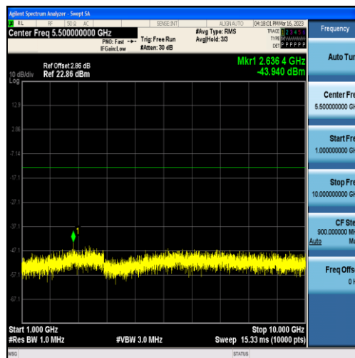
Band12-1.4MHz-16QAM-23095-6RB#0-Range2:1000~10000MHz
