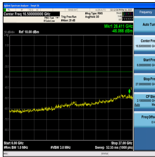
Band7-15MHz-16QAM-21100-75RB#0-Range3:6000~27000MHz
