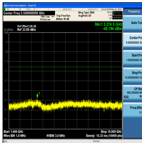
Band12-5MHz-16QAM-23095-25RB#0-Range2:1000~10000MHz
