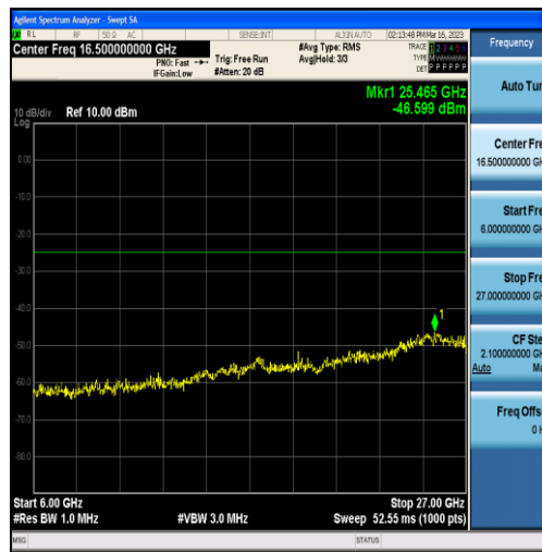
Band7-15MHz-16QAM-21375-75RB#0-Range3:6000~27000MHz
