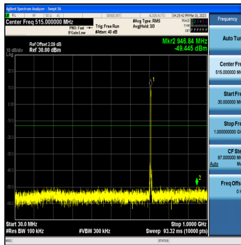
Band12-3MHz-QPSK-23165-15RB#0-Range1:30~1000MHz
