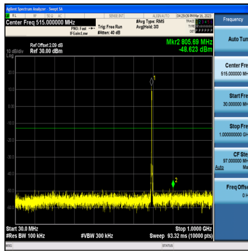
Band12-3MHz-16QAM-23025-15RB#0-Range1:30~1000MHz
