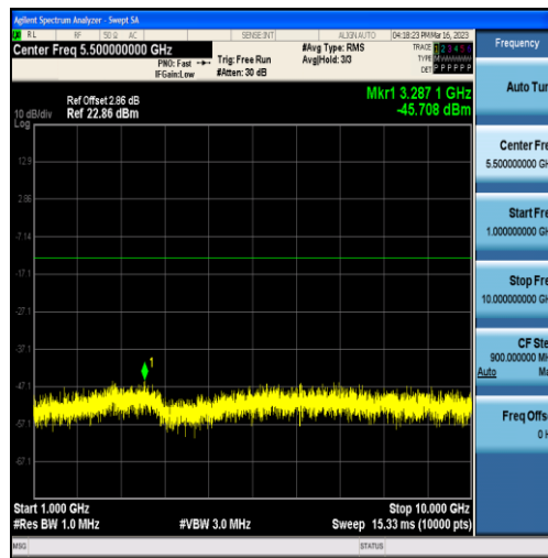
Band12-1.4MHz-16QAM-23173-6RB#0-Range2:1000~10000MHz
