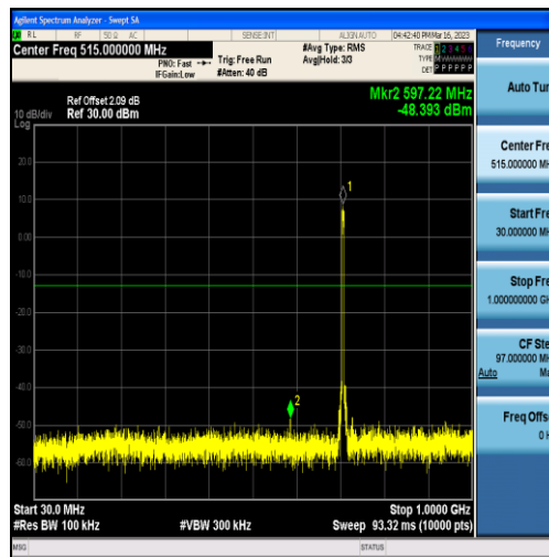
Band12-5MHz-QPSK-23155-25RB#0-Range1:30~1000MHz
