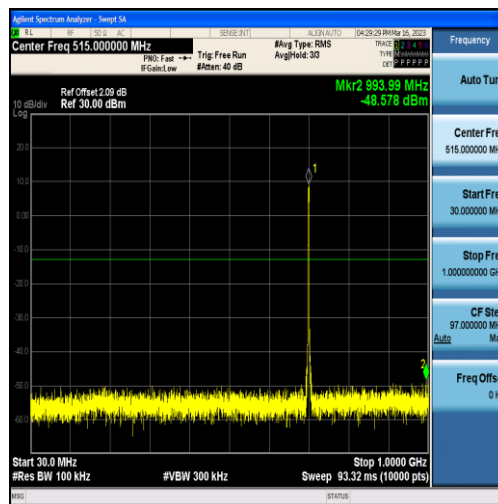
Band12-3MHz-16QAM-23095-15RB#0-Range1:30~1000MHz
