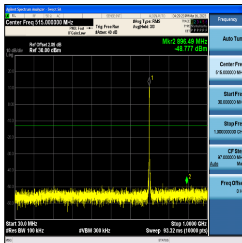
Band12-3MHz-QPSK-23095-15RB#0-Range1:30~1000MHz
