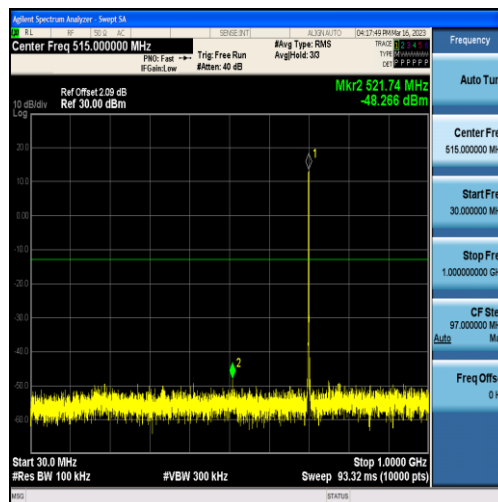
Band12-1.4MHz-QPSK-23095-6RB#0-Range1:30~1000MHz
