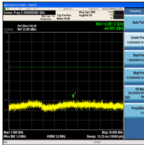
Band12-3MHz-16QAM-23025-15RB#0-Range2:1000~10000MHz
