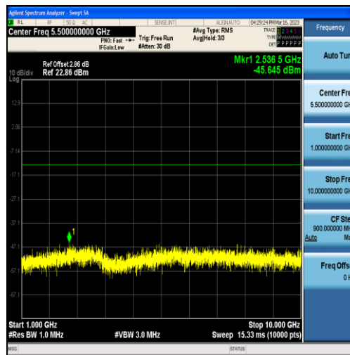
Band12-3MHz-QPSK-23095-15RB#0-Range2:1000~10000MHz
