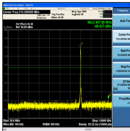
Band12-5MHz-QPSK-23095-25RB#0-Range1:30~1000MHz
