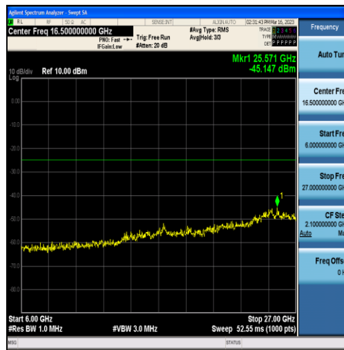
Band7-20MHz-16QAM-21100-100RB#0-Range3:6000~27000MHz
