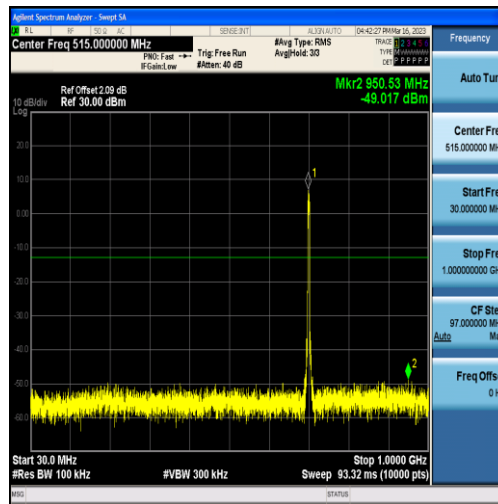
Band12-5MHz-16QAM-23095-25RB#0-Range1:30~1000MHz
