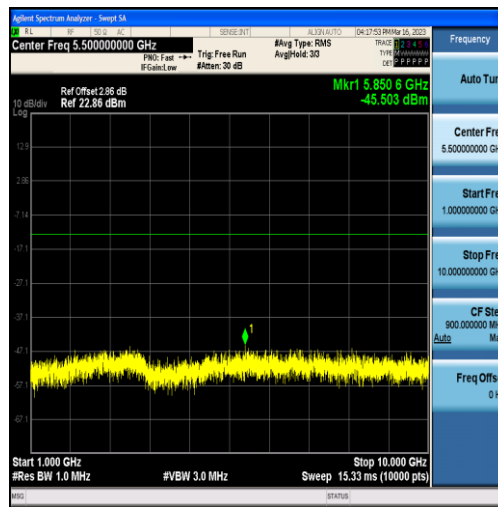
Band12-1.4MHz-QPSK-23095-6RB#0-Range2:1000~10000MHz
