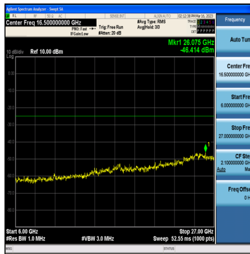
Band7-15MHz-QPSK-21375-75RB#0-Range3:6000~27000MHz
