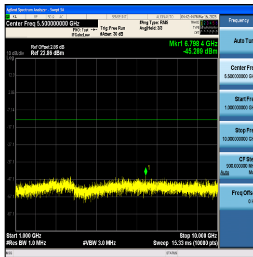
Band12-5MHz-QPSK-23155-25RB#0-Range2:1000~10000MHz
