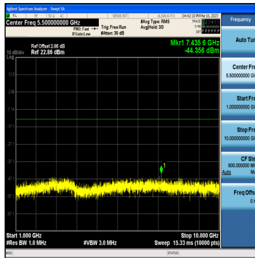
Band12-5MHz-16QAM-23035-25RB#0-Range2:1000~10000MHz
