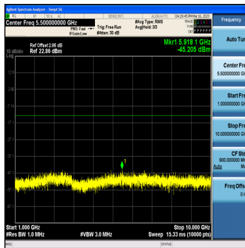
Band12-3MHz-QPSK-23165-15RB#0-Range2:1000~10000MHz
