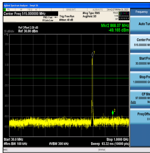
Band12-5MHz-16QAM-23035-25RB#0-Range1:30~1000MHz
