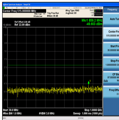
Band7-20MHz-QPSK-21100-100RB#0-Range1:30~1000MHz
