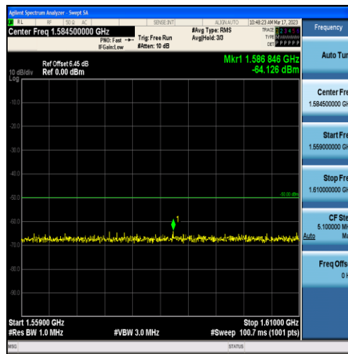
Band13-5MHz-QPSK-23205-25RB#0-Range3:1559~1610MHz
