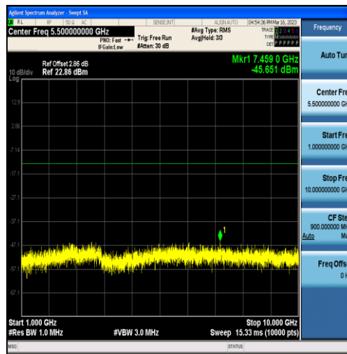
Band12-10MHz-16QAM-23130-50RB#0-Range2:1000~10000MHz
