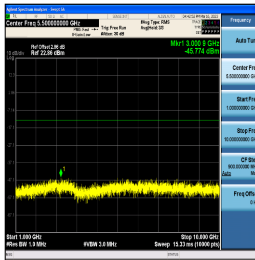
Band12-5MHz-16QAM-23155-25RB#0-Range2:1000~10000MHz
