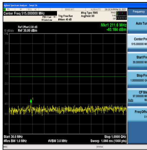
Band25-1.4MHz-QPSK-26683-6RB#0-Range1:30~1000MHz
