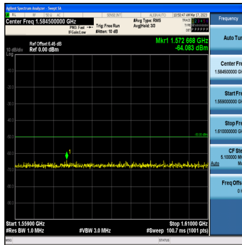
Band13-10MHz-16QAM-23230-50RB#0-Range3:1559~1610MHz
