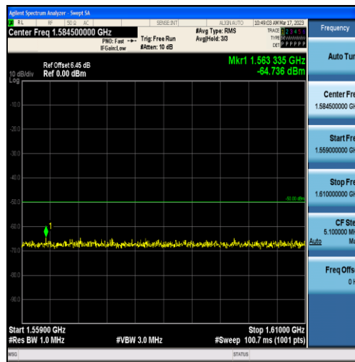
Band13-5MHz-16QAM-23230-25RB#0-Range3:1559~1610MHz
