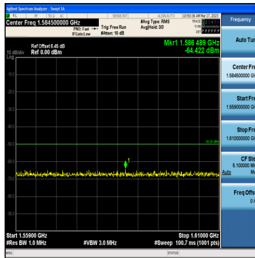
Band13-10MHz-QPSK-23230-50RB#0-Range3:1559~1610MHz
