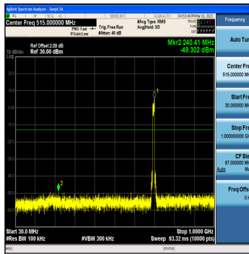
Band12-10MHz-16QAM-23060-50RB#0-Range1:30~1000MHz
