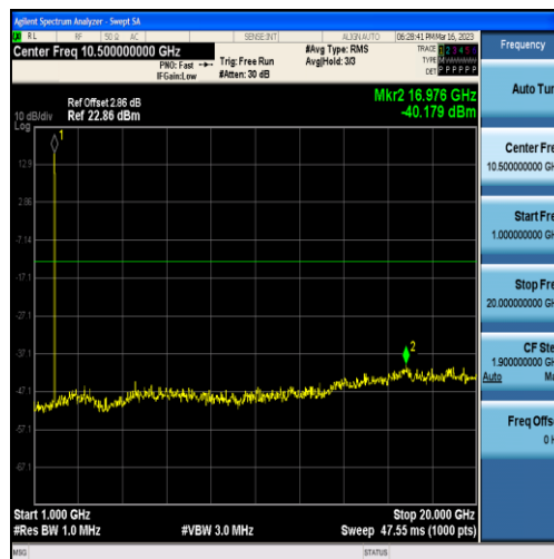
Band25-3MHz-16QAM-26365-15RB#0-Range2:1000~20000MHz
