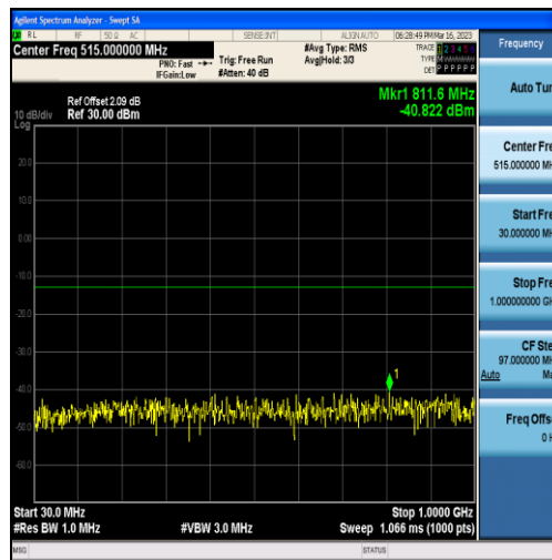
Band25-3MHz-QPSK-26675-15RB#0-Range1:30~1000MHz
