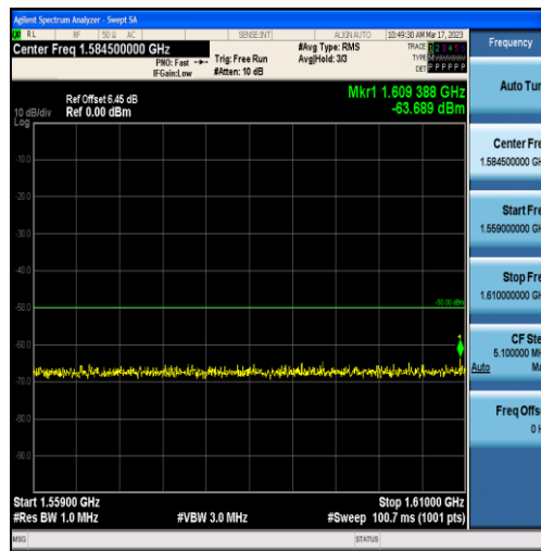
Band13-5MHz-16QAM-23255-25RB#0-Range3:1559~1610MHz
