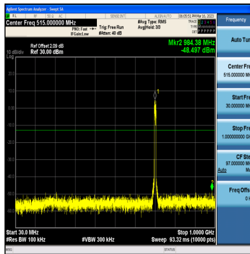
Band17-10MHz-16QAM-23780-50RB#0-Range1:30~1000MHz
