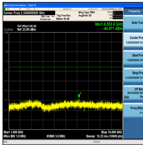
Band12-10MHz-QPSK-23095-50RB#0-Range2:1000~10000MHz
