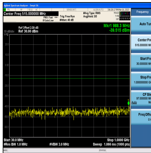
Band25-3MHz-16QAM-26055-15RB#0-Range1:30~1000MHz
