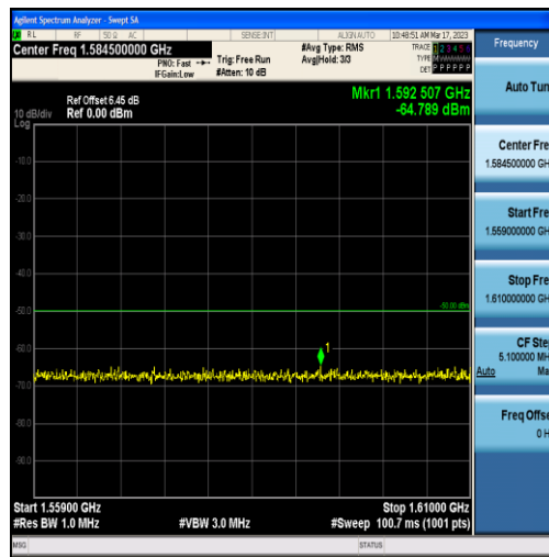
Band13-5MHz-QPSK-23230-25RB#0-Range3:1559~1610MHz
