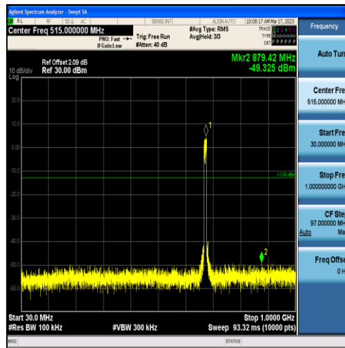
Band71-10MHz-16QAM-133297-50RB#0-Range1:30~1000MHz
