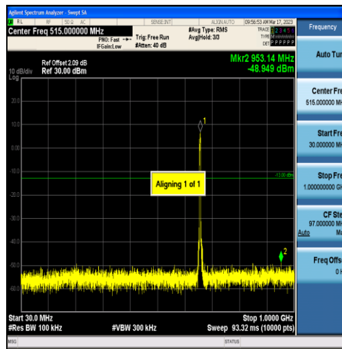
Band71-5MHz-16QAM-133147-25RB#0-Range1:30~1000MHz
