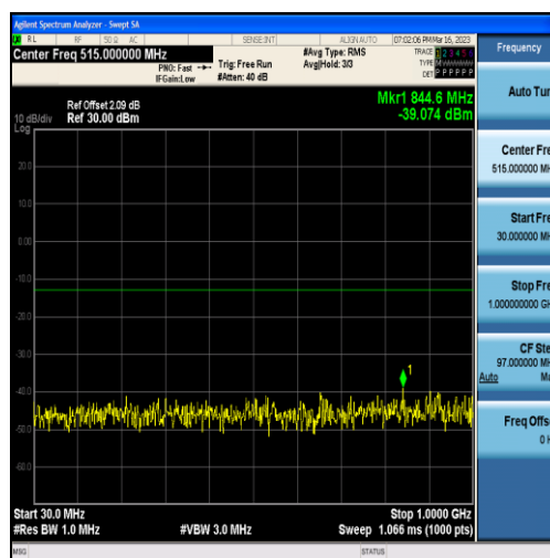
Band25-10MHz-16QAM-26640-50RB#0-Range1:30~1000MHz
