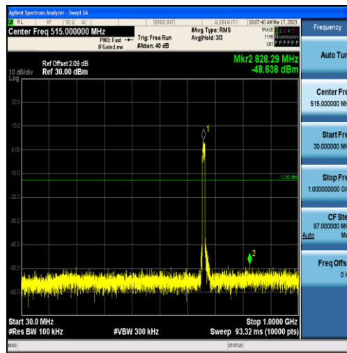
Band71-10MHz-16QAM-133172-50RB#0-Range1:30~1000MHz
