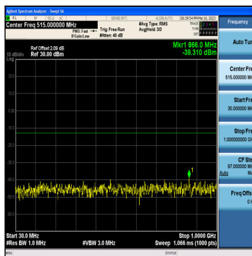
Band25-5MHz-16QAM-26665-25RB#0-Range1:30~1000MHz
