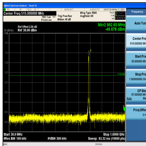
Band71-5MHz-16QAM-133447-25RB#0-Range1:30~1000MHz
