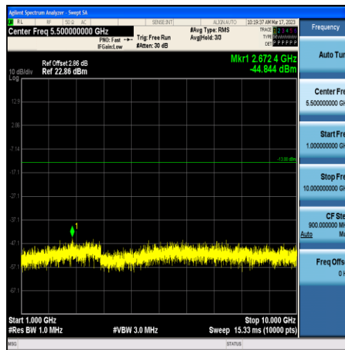
Band71-15MHz-QPSK-133297-75RB#0-Range2:1000~10000MHz
