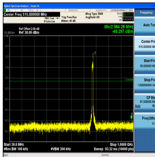
Band71-10MHz-QPSK-133297-50RB#0-Range1:30~1000MHz
