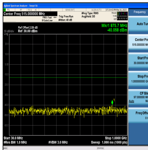
Band25-20MHz-16QAM-26590-100RB#0-Range1:30~1000MHz
