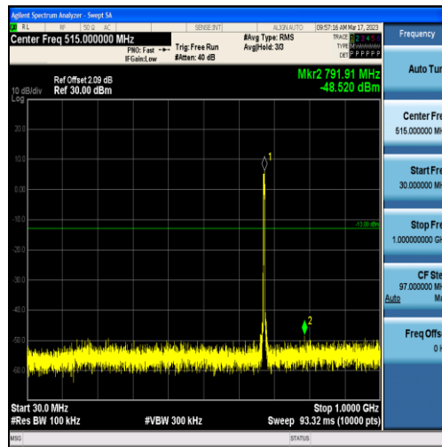
Band71-5MHz-16QAM-133297-25RB#0-Range1:30~1000MHz
