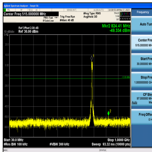
Band71-10MHz-16QAM-133422-50RB#0-Range1:30~1000MHz
