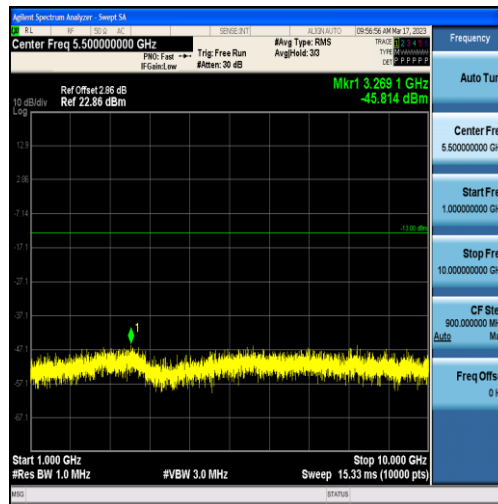
Band71-5MHz-16QAM-133147-25RB#0-Range2:1000~10000MHz
