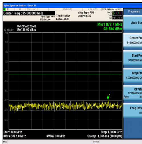
Band25-5MHz-16QAM-26365-25RB#0-Range1:30~1000MHz
