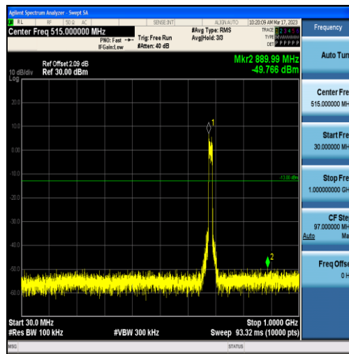
Band71-15MHz-QPSK-133397-75RB#0-Range1:30~1000MHz
