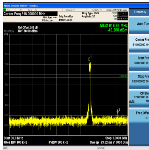
Band71-15MHz-16QAM-133397-75RB#0-Range1:30~1000MHz
