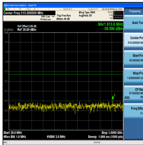
Band25-5MHz-QPSK-26665-25RB#0-Range1:30~1000MHz
