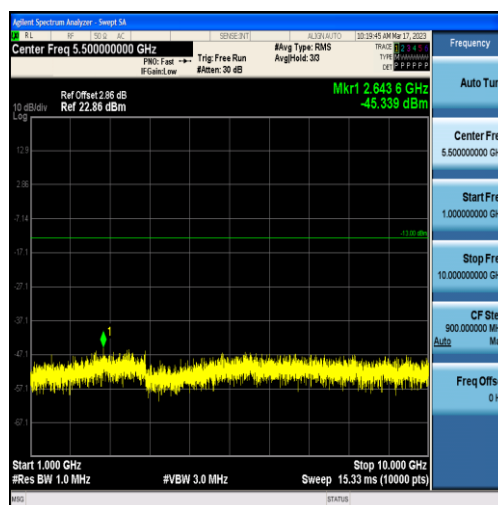
Band71-15MHz-16QAM-133297-75RB#0-Range2:1000~10000MHz
