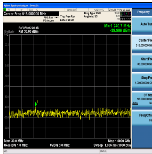
Band25-10MHz-QPSK-26640-50RB#0-Range1:30~1000MHz
