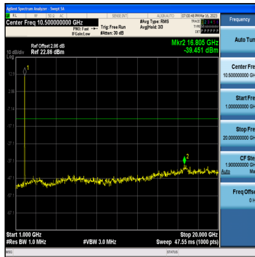
Band25-10MHz-16QAM-26090-50RB#0-Range2:1000~20000MHz
