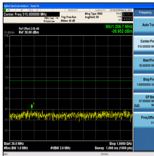
Band25-15MHz-QPSK-26615-75RB#0-Range1:30~1000MHz
