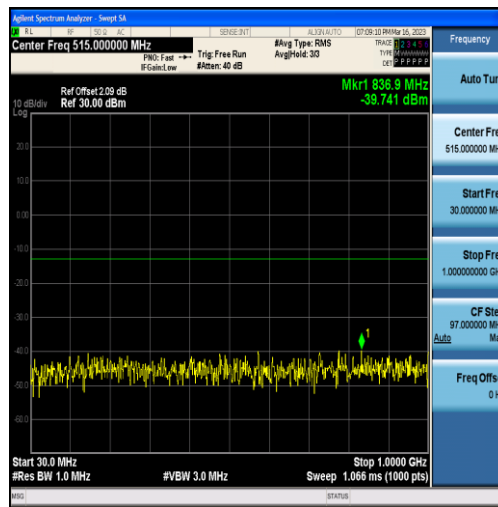
Band25-15MHz-16QAM-26365-75RB#0-Range1:30~1000MHz
