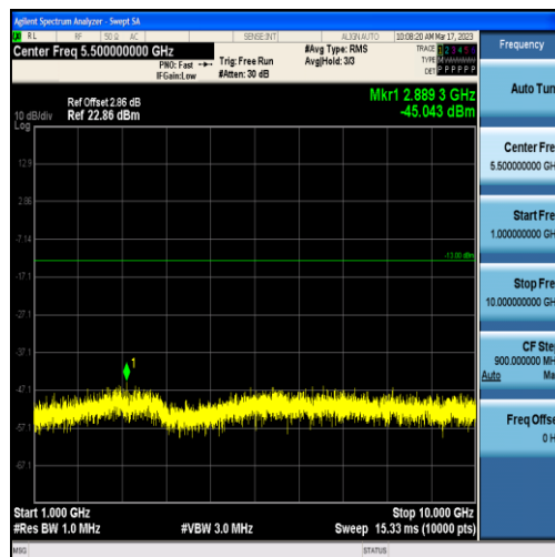
Band71-10MHz-16QAM-133297-50RB#0-Range2:1000~10000MHz
