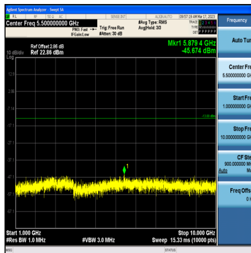
Band71-5MHz-16QAM-133297-25RB#0-Range2:1000~10000MHz
