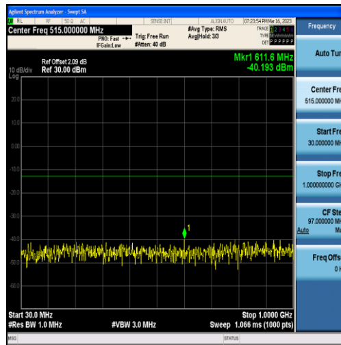
Band25-20MHz-16QAM-26365-100RB#0-Range1:30~1000MHz
