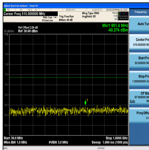
Band25-5MHz-QPSK-26365-25RB#0-Range1:30~1000MHz
