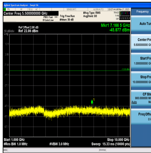
Band71-10MHz-16QAM-133172-50RB#0-Range2:1000~10000MHz
