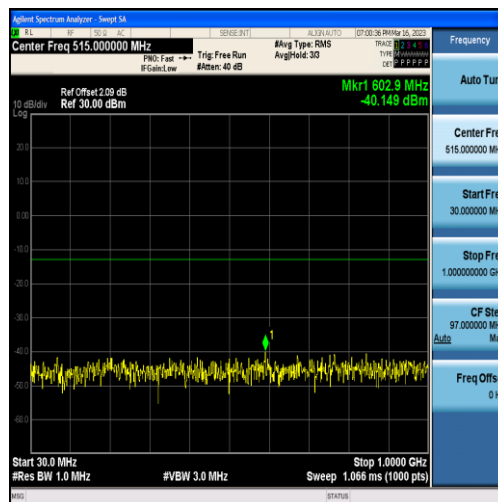
Band25-10MHz-QPSK-26090-50RB#0-Range1:30~1000MHz
