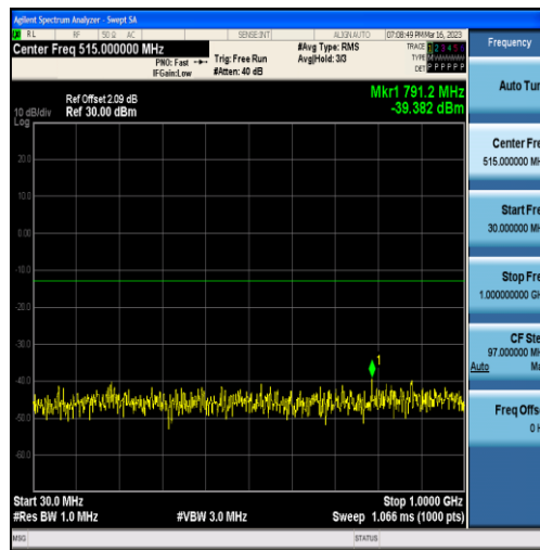
Band25-15MHz-16QAM-26115-75RB#0-Range1:30~1000MHz
