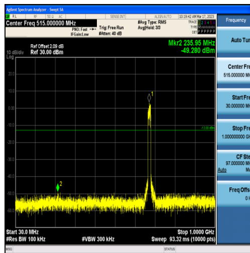
Band71-15MHz-16QAM-133297-75RB#0-Range1:30~1000MHz
