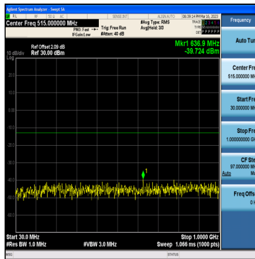
Band25-5MHz-16QAM-26065-25RB#0-Range1:30~1000MHz
