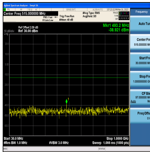
Band25-20MHz-16QAM-26140-100RB#0-Range1:30~1000MHz
