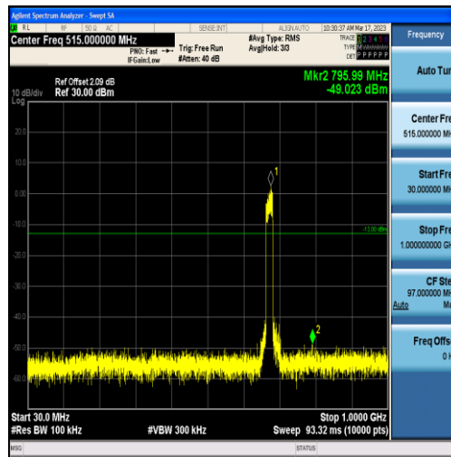
Band71-20MHz-16QAM-133297-100RB#0-Range1:30~1000MHz
