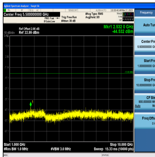
Band71-20MHz-16QAM-133297-100RB#0-Range2:1000~10000MHz
