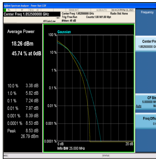
Band25-5MHz-16QAM-26065-25RB#0
