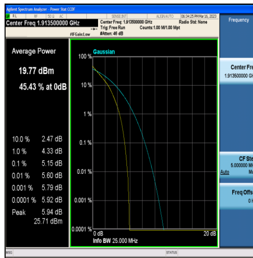
Band25-3MHz-QPSK-26675-15RB#0
