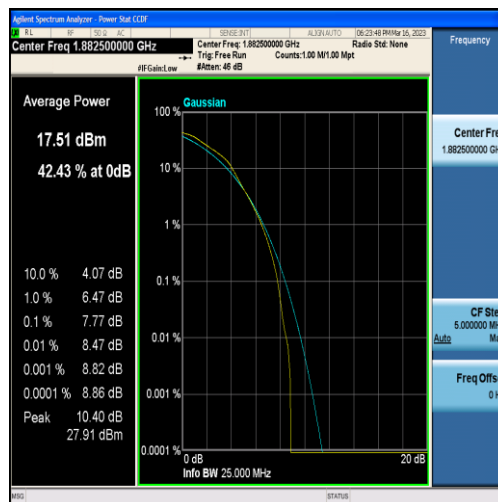
Band25-1.4MHz-16QAM-26365-6RB#0
