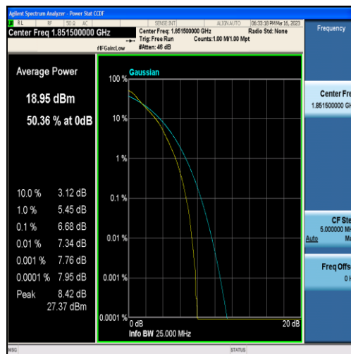
Band25-3MHz-QPSK-26055-15RB#0
