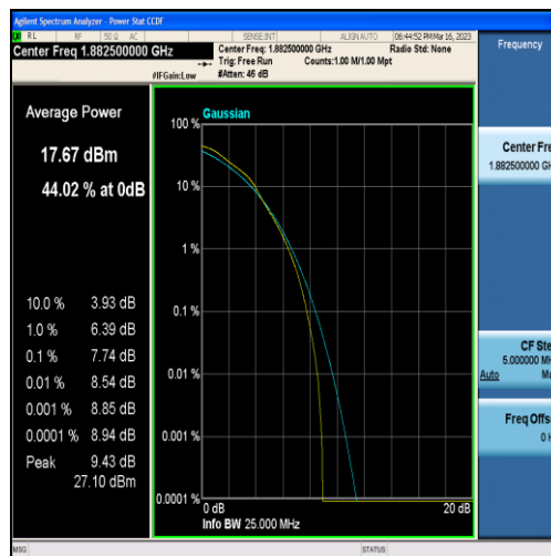
Band25-5MHz-16QAM-26365-25RB#0
