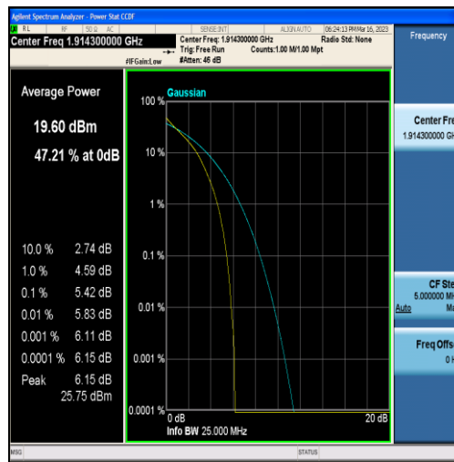
Band25-1.4MHz-QPSK-26683-6RB#0
