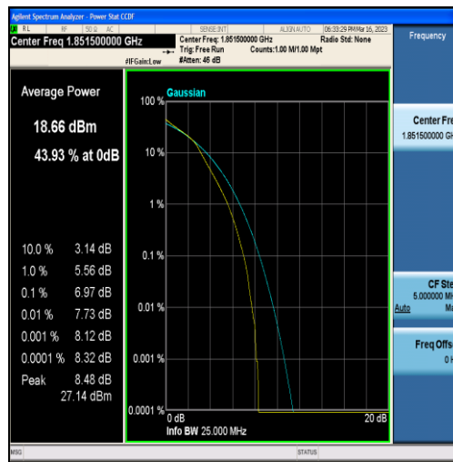
Band25-3MHz-16QAM-26055-15RB#0
