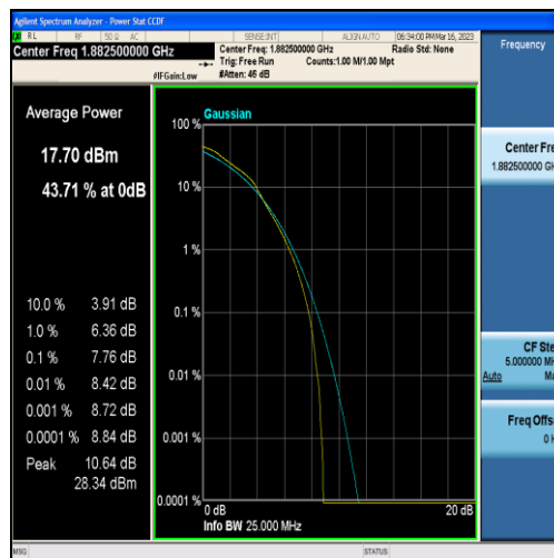
Band25-3MHz-16QAM-26365-15RB#0
