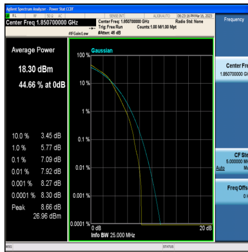
Band25-1.4MHz-16QAM-26047-6RB#0
