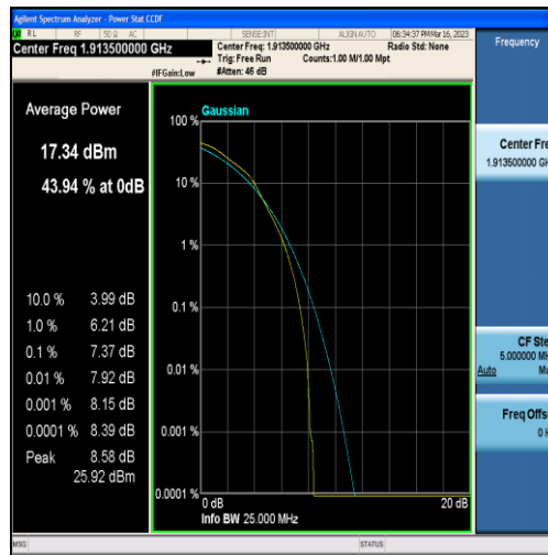
Band25-3MHz-16QAM-26675-15RB#0
