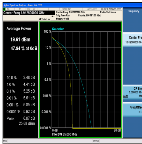
Band25-5MHz-QPSK-26665-25RB#0
