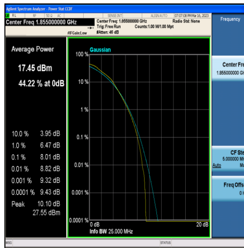
Band25-10MHz-16QAM-26090-50RB#0
