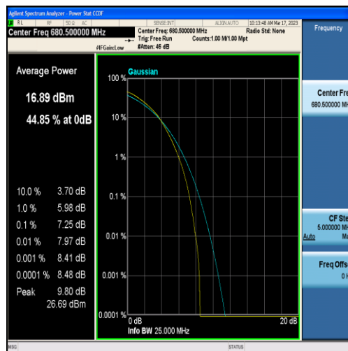
Band71-10MHz-16QAM-133297-50RB#0
