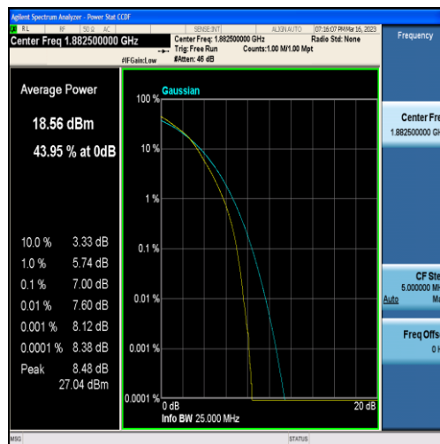
Band25-15MHz-16QAM-26365-75RB#0
