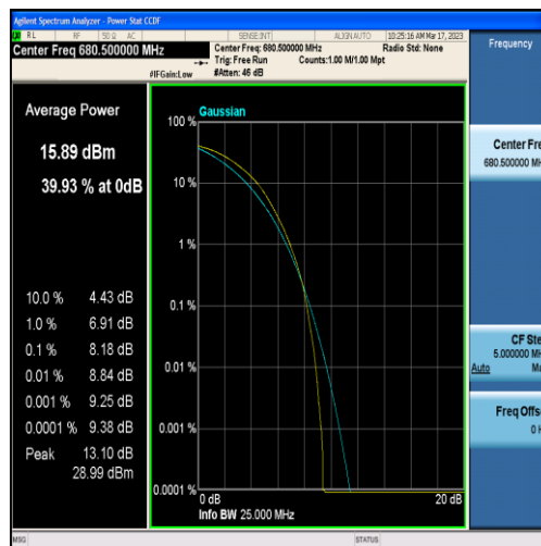
Band71-15MHz-16QAM-133297-75RB#0
