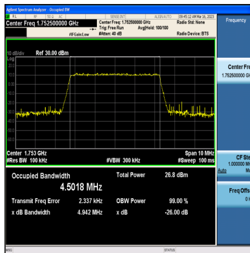
Band4-5MHz-16QAM-20375-25RB#0-4.5018
