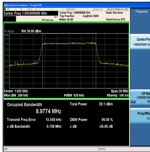
Band2-10MHz-16QAM-18650-50RB#0-8.9774
