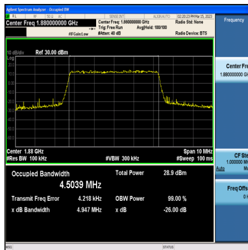
Band2-5MHz-QPSK-18900-25RB#0-4.5039
