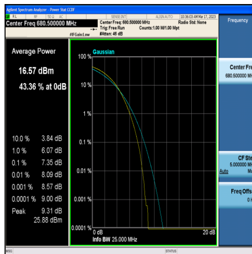
Band71-20MHz-16QAM-133297-100RB#0
