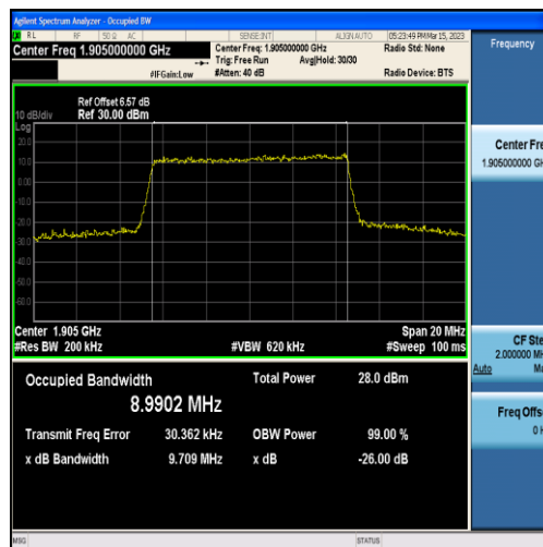
Band2-10MHz-16QAM-19150-50RB#0-8.9902
