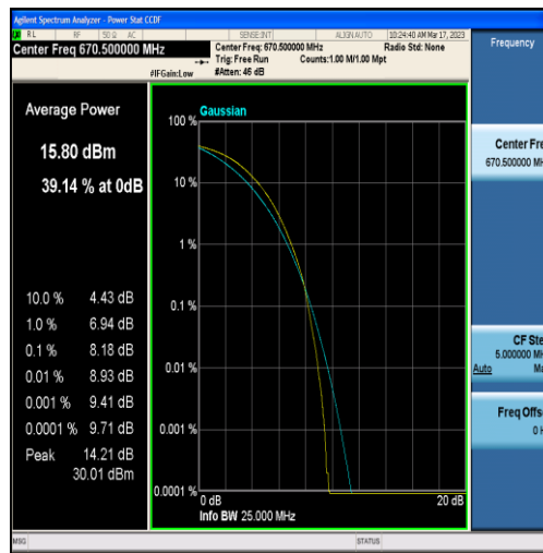
Band71-15MHz-16QAM-133197-75RB#0
