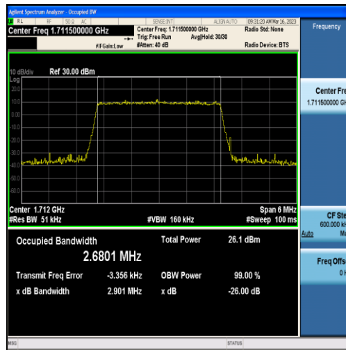
Band4-3MHz-16QAM-19965-15RB#0-2.6801
