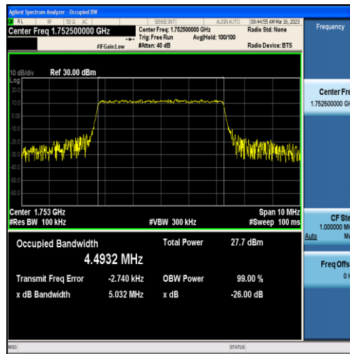
Band4-5MHz-QPSK-20375-25RB#0-4.4932
