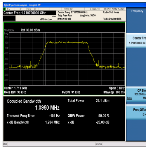
Band4-1.4MHz-16QAM-19957-6RB#0-1.0950
