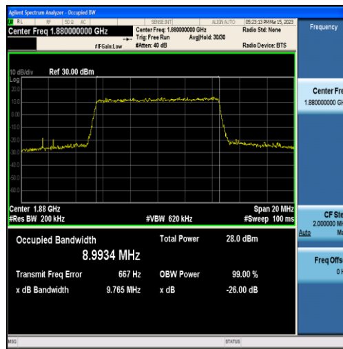
Band2-10MHz-16QAM-18900-50RB#0-8.9934
