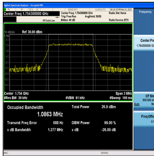
Band4-1.4MHz-QPSK-20393-6RB#0-1.0863
