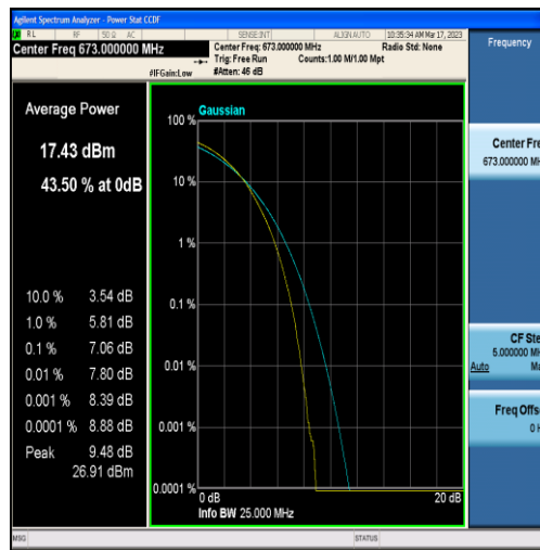
Band71-20MHz-16QAM-133222-100RB#0
