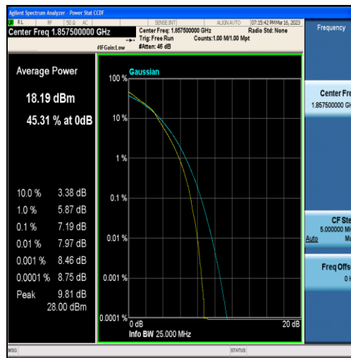
Band25-15MHz-16QAM-26115-75RB#0
