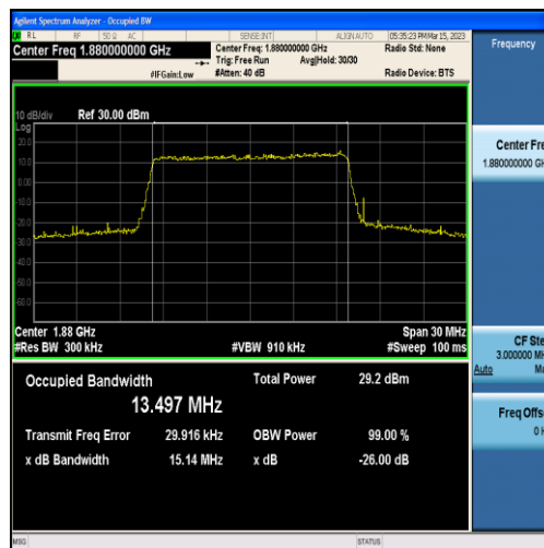
Band2-15MHz-QPSK-18900-75RB#0-13.497
