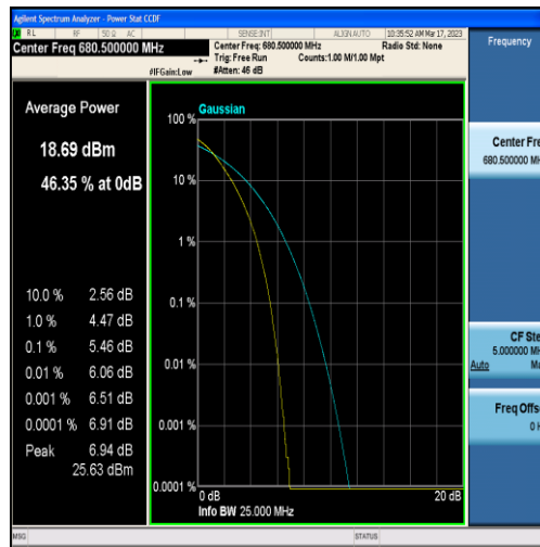
Band71-20MHz-QPSK-133297-100RB#0
