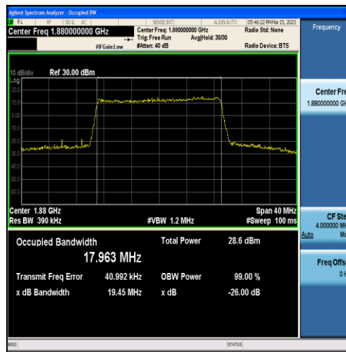
Band2-20MHz-16QAM-18900-100RB#0-17.963
