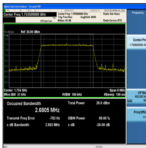
Band4-3MHz-16QAM-20385-15RB#0-2.6805
