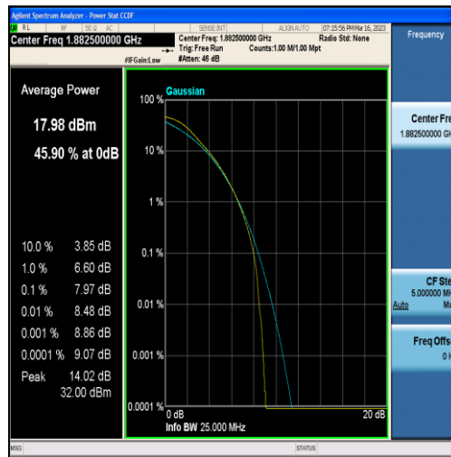
Band25-15MHz-QPSK-26365-75RB#0
