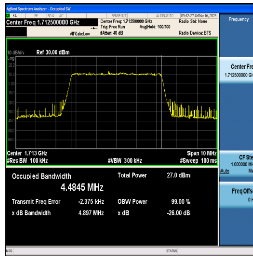
Band4-5MHz-16QAM-19975-25RB#0-4.4845
