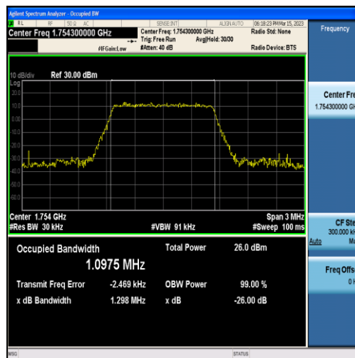
Band4-1.4MHz-16QAM-20393-6RB#0-1.0975
