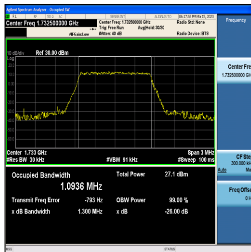
Band4-1.4MHz-QPSK-20175-6RB#0-1.0936
