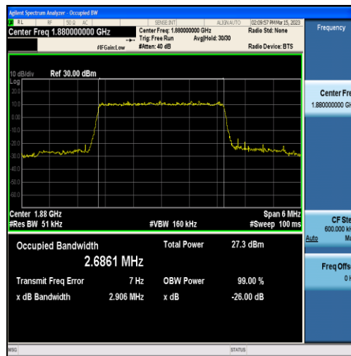
Band2-3MHz-16QAM-18900-15RB#0-2.6861
