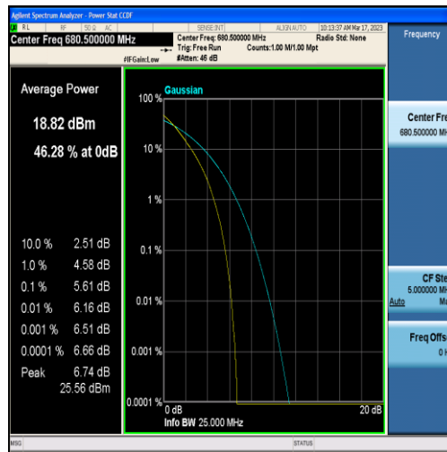
Band71-10MHz-QPSK-133297-50RB#0
