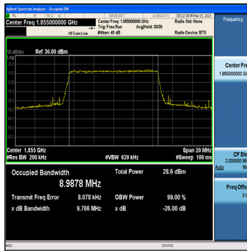
Band2-10MHz-QPSK-18650-50RB#0-8.9878
