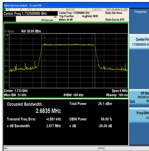
Band4-3MHz-16QAM-20175-15RB#0-2.6835
