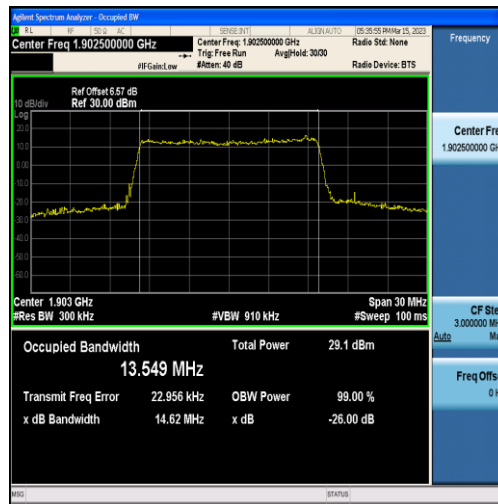
Band2-15MHz-QPSK-19125-75RB#0-13.549
