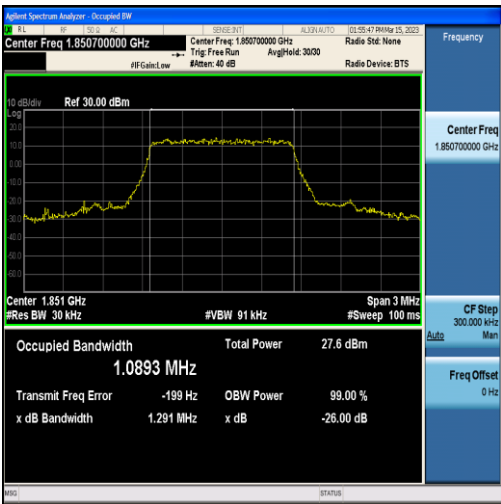
Band2-1.4MHz-QPSK-18607-6RB#0-1.0893
