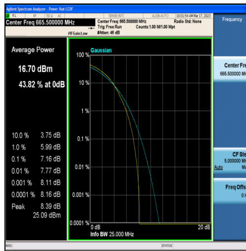
Band71-5MHz-16QAM-133147-25RB#0
