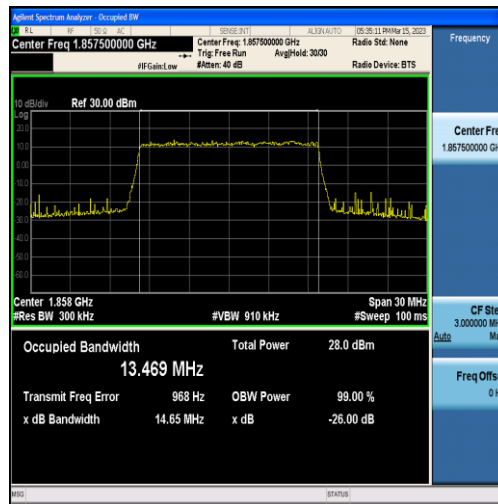
Band2-15MHz-16QAM-18675-75RB#0-13.469
