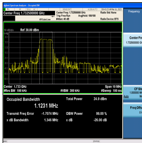
Band4-5MHz-QPSK-20175-25RB#0-1.1231
