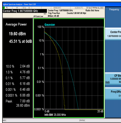
Band25-15MHz-QPSK-26615-75RB#0
