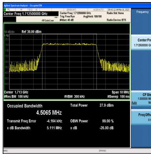
Band4-5MHz-QPSK-19975-25RB#0-4.5065
