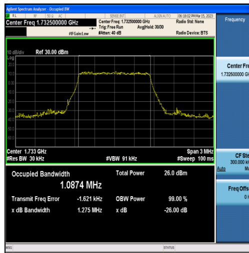
Band4-1.4MHz-16QAM-20175-6RB#0-1.0874
