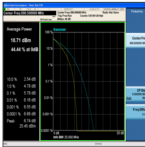
Band71-15MHz-QPSK-133397-75RB#0
