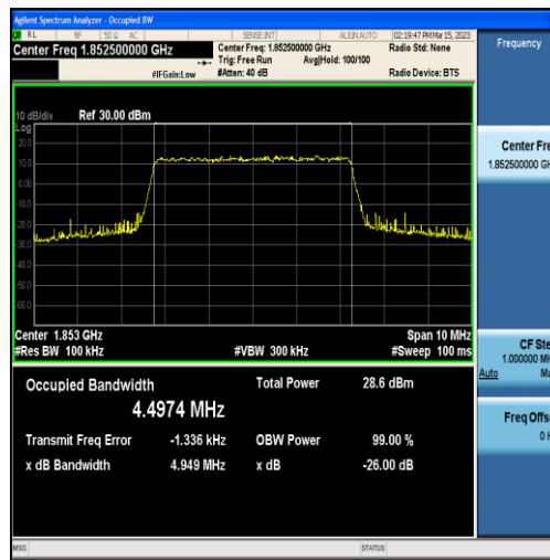
Band2-5MHz-QPSK-18625-25RB#0-4.4974
