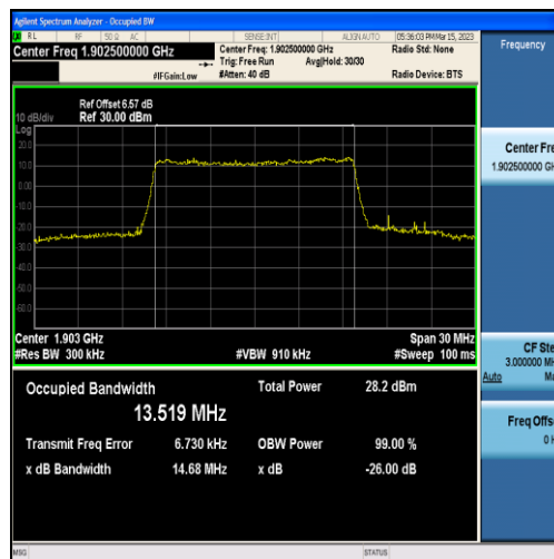
Band2-15MHz-16QAM-19125-75RB#0-13.519
