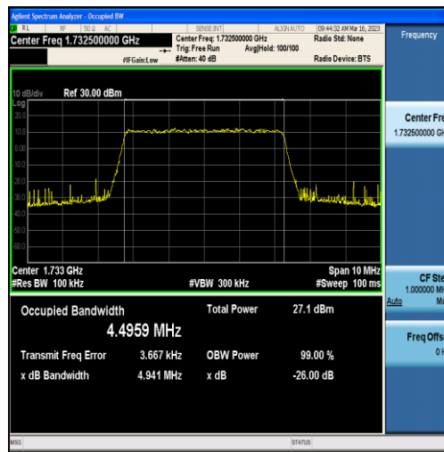
Band4-5MHz-16QAM-20175-25RB#0-4.4959
