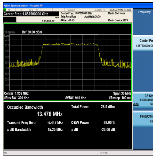
Band2-15MHz-QPSK-18675-75RB#0-13.478
