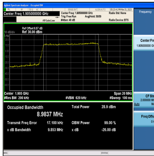
Band2-10MHz-QPSK-19150-50RB#0-8.9837
