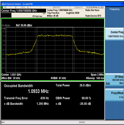
Band2-1.4MHz-16QAM-18607-6RB#0-1.0933
