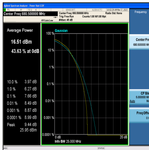
Band71-5MHz-16QAM-133297-25RB#0
