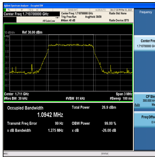
Band4-1.4MHz-QPSK-19957-6RB#0-1.0942
