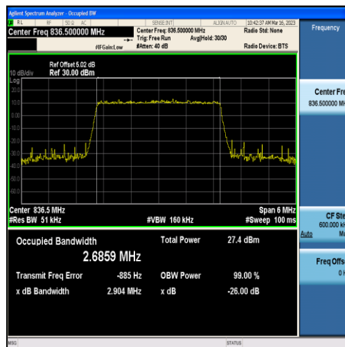
Band5-3MHz-QPSK-20525-15RB#0-2.6859
