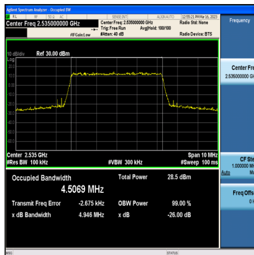
Band7-5MHz-QPSK-21100-25RB#0-4.5069
