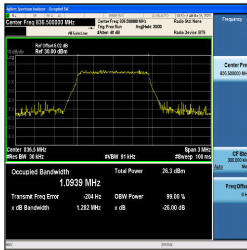
Band5-1.4MHz-16QAM-20525-6RB#0-1.0939
