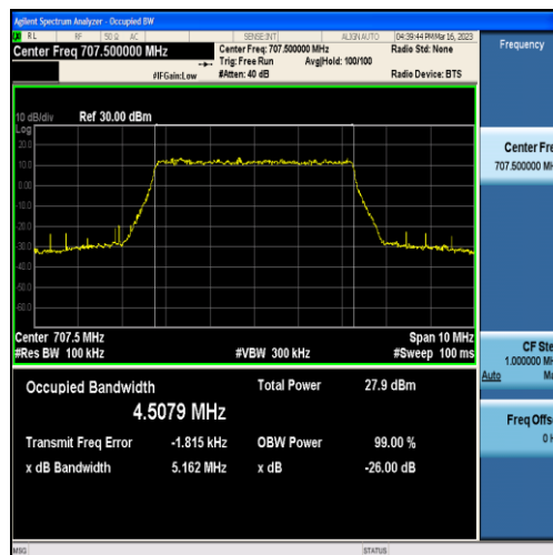
Band12-5MHz-QPSK-23095-25RB#0-4.5079
