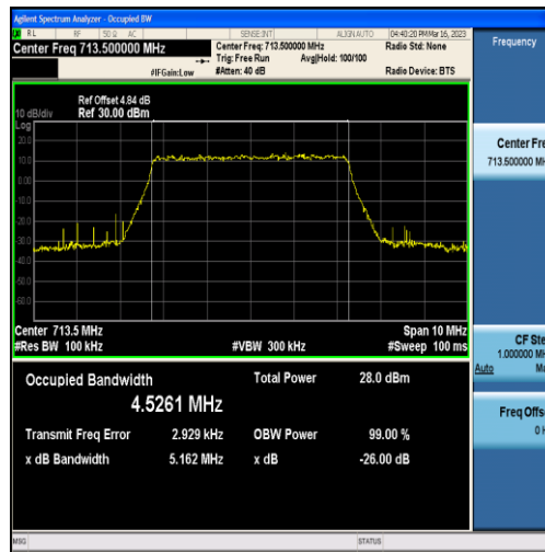
Band12-5MHz-QPSK-23155-25RB#0-4.5261
