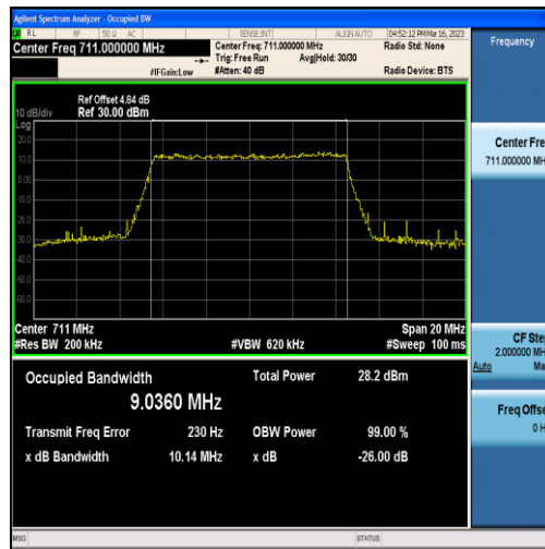
Band12-10MHz-QPSK-23130-50RB#0-9.0360
