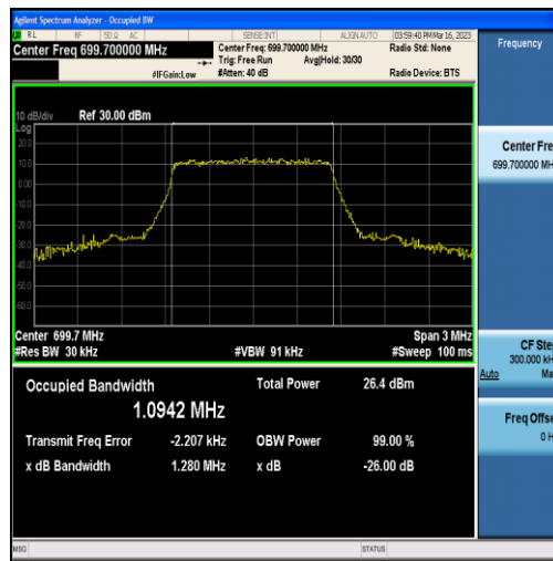
Band12-1.4MHz-QPSK-23017-6RB#0-1.0942
