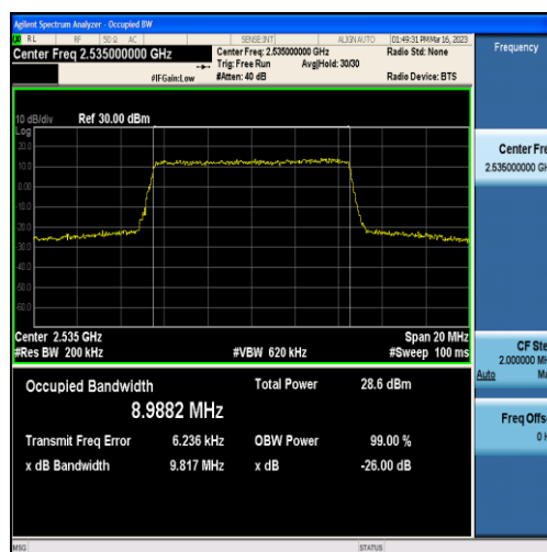
Band7-10MHz-QPSK-21100-50RB#0-8.9882
