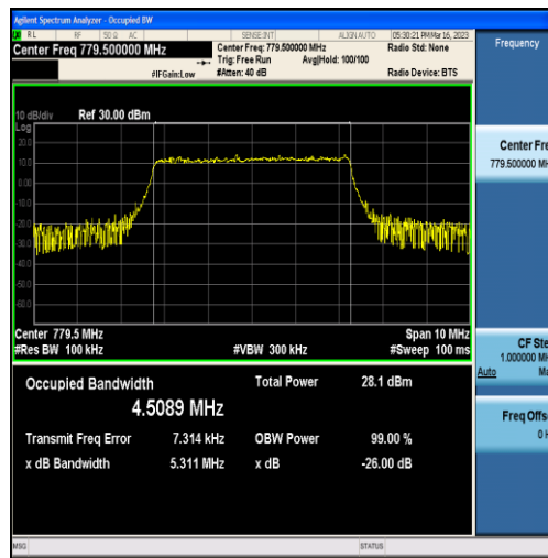
Band13-5MHz-QPSK-23205-25RB#0-4.5089
