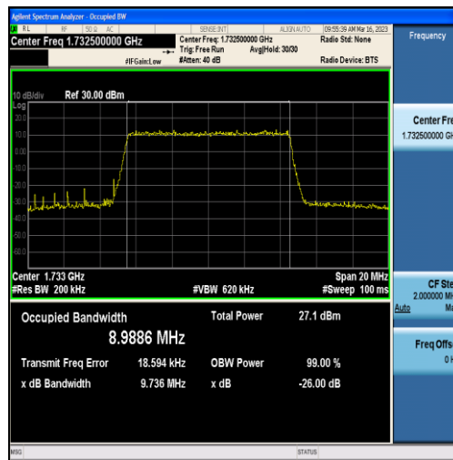
Band4-10MHz-16QAM-20175-50RB#0-8.9886
