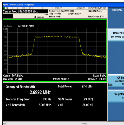
Band12-3MHz-QPSK-23095-15RB#0-2.6892
