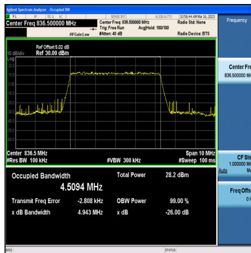
Band5-5MHz-QPSK-20525-25RB#0-4.5094
