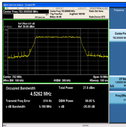
Band13-5MHz-QPSK-23230-25RB#0-4.5262
