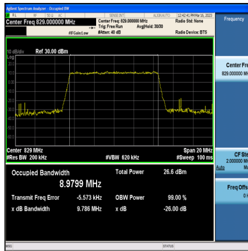
Band5-10MHz-16QAM-20450-50RB#0-8.9799
