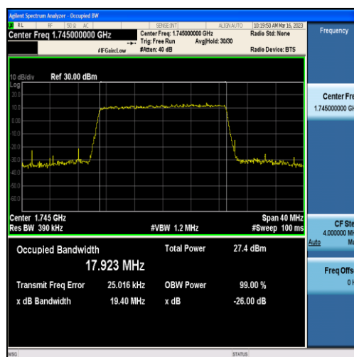
Band4-20MHz-16QAM-20300-100RB#0-17.923
