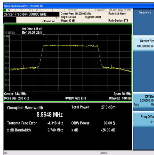
Band5-10MHz-16QAM-20600-50RB#0-8.9648
