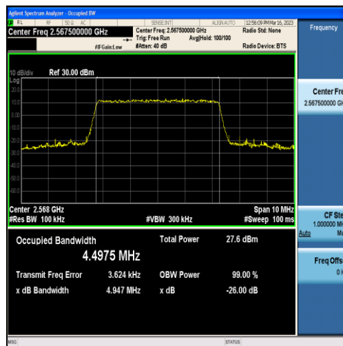
Band7-5MHz-16QAM-21425-25RB#0-4.4975
