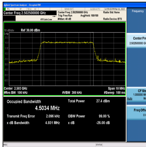
Band7-5MHz-16QAM-20775-25RB#0-4.5034
