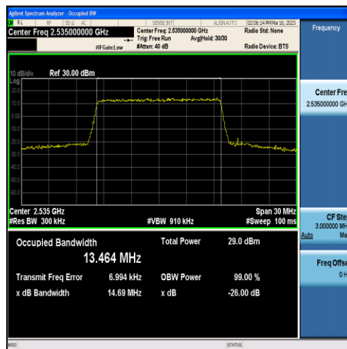
Band7-15MHz-QPSK-21100-75RB#0-13.464
