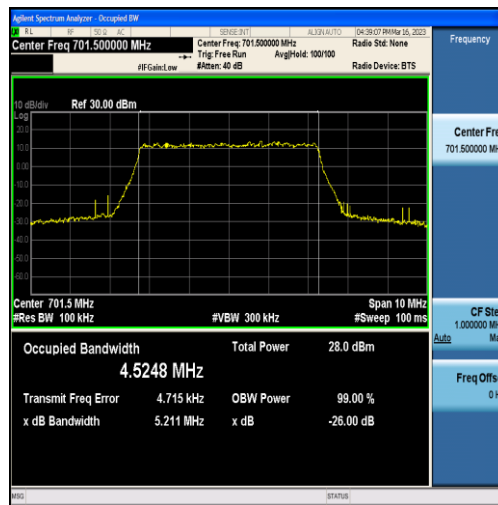
Band12-5MHz-QPSK-23035-25RB#0-4.5248
