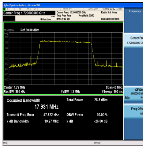
Band4-20MHz-QPSK-20050-100RB#0-17.931
