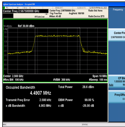
Band7-5MHz-QPSK-21425-25RB#0-4.4907
