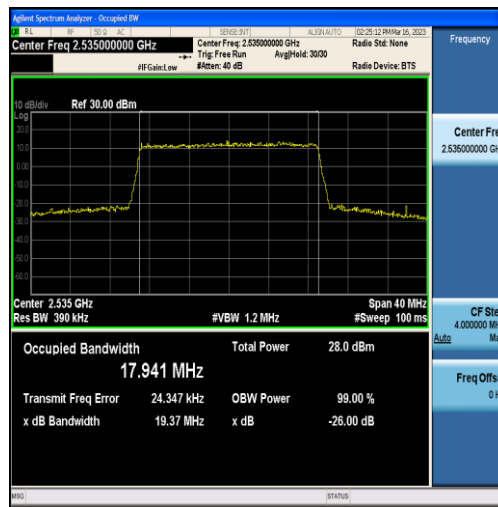
Band7-20MHz-16QAM-21100-100RB#0-17.941
