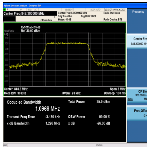
Band5-1.4MHz-16QAM-20643-6RB#0-1.0968
