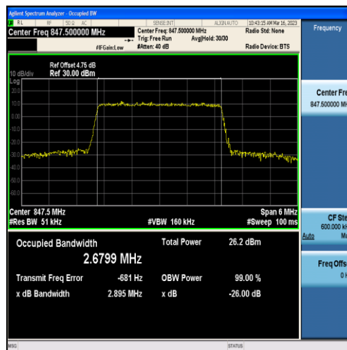
Band5-3MHz-16QAM-20635-15RB#0-2.6799
