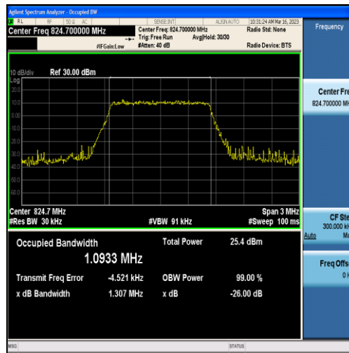
Band5-1.4MHz-16QAM-20407-6RB#0-1.0933
