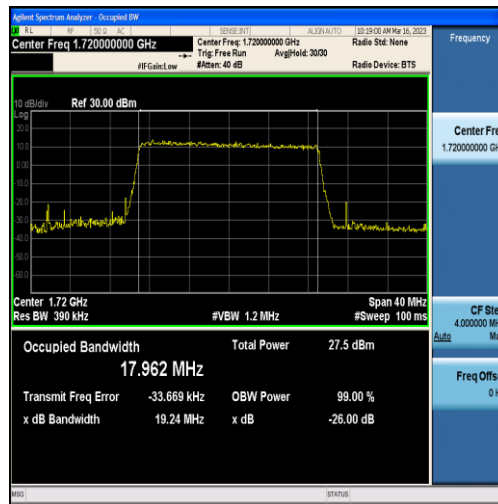
Band4-20MHz-16QAM-20050-100RB#0-17.962
