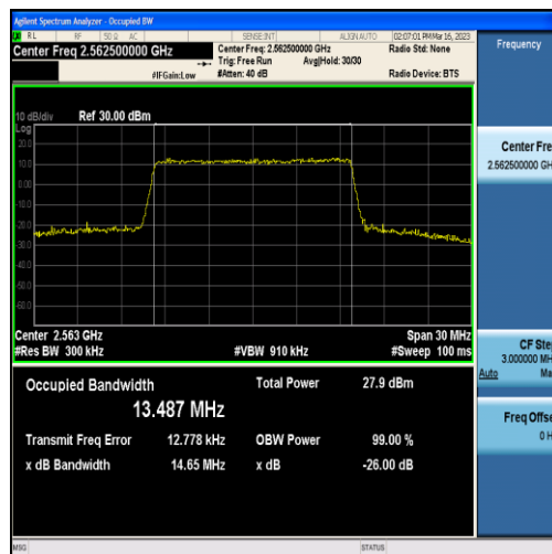
Band7-15MHz-16QAM-21375-75RB#0-13.487
