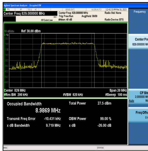
Band5-10MHz-QPSK-20450-50RB#0-8.9869
