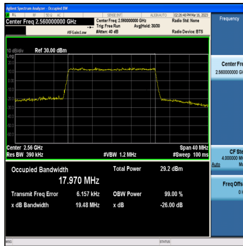
Band7-20MHz-QPSK-21350-100RB#0-17.970
