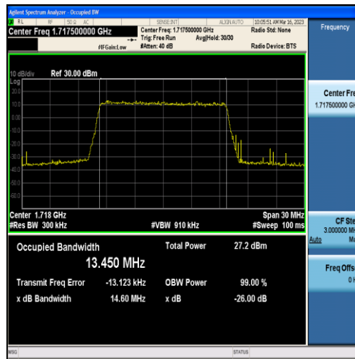
Band4-15MHz-16QAM-20025-75RB#0-13.450
