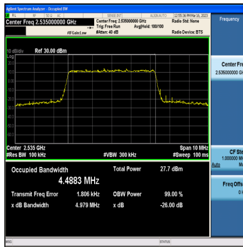
Band7-5MHz-16QAM-21100-25RB#0-4.4883
