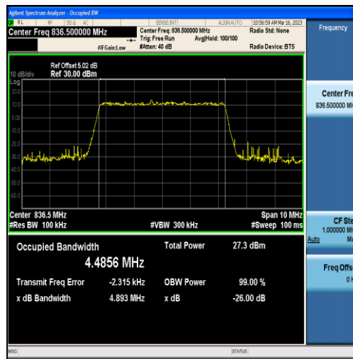
Band5-5MHz-16QAM-20525-25RB#0-4.4856
