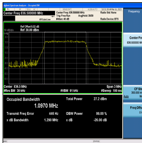
Band5-1.4MHz-QPSK-20525-6RB#0-1.0970
