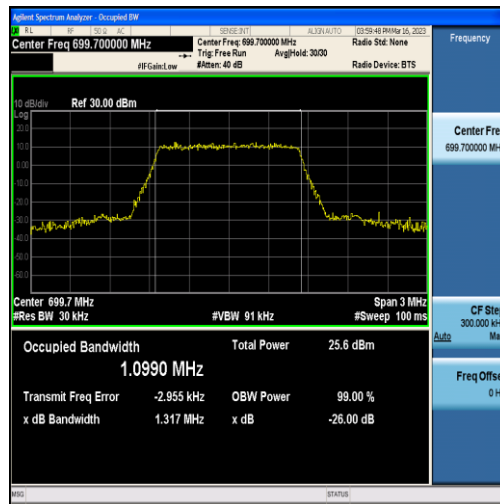
Band12-1.4MHz-16QAM-23017-6RB#0-1.0990
