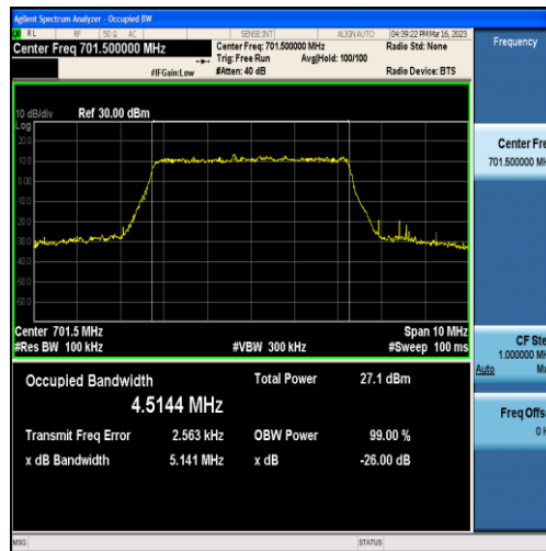
Band12-5MHz-16QAM-23035-25RB#0-4.5144
