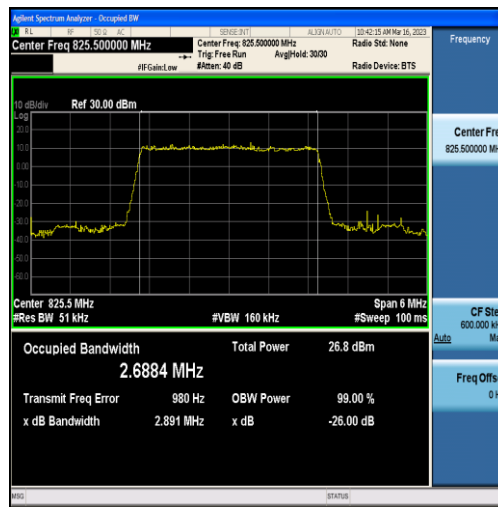
Band5-3MHz-QPSK-20415-15RB#0-2.6884
