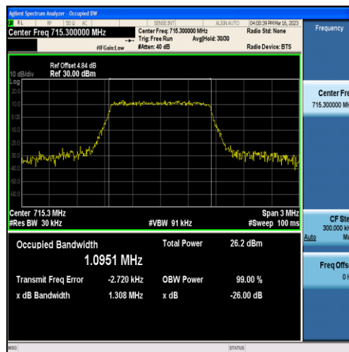
Band12-1.4MHz-16QAM-23173-6RB#0-1.0951
