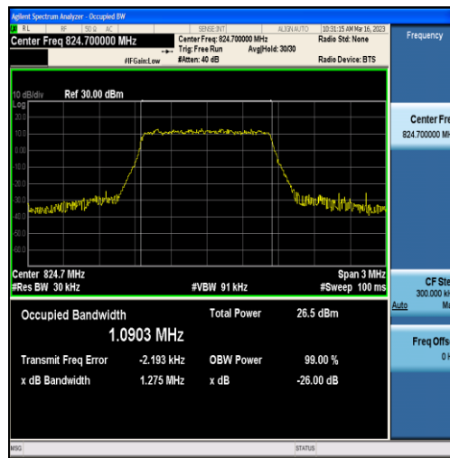
Band5-1.4MHz-QPSK-20407-6RB#0-1.0903
