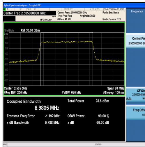
Band7-10MHz-QPSK-20800-50RB#0-8.9805
