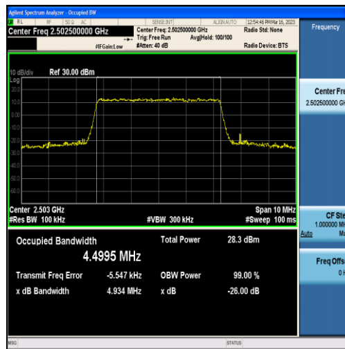
Band7-5MHz-QPSK-20775-25RB#0-4.4995
