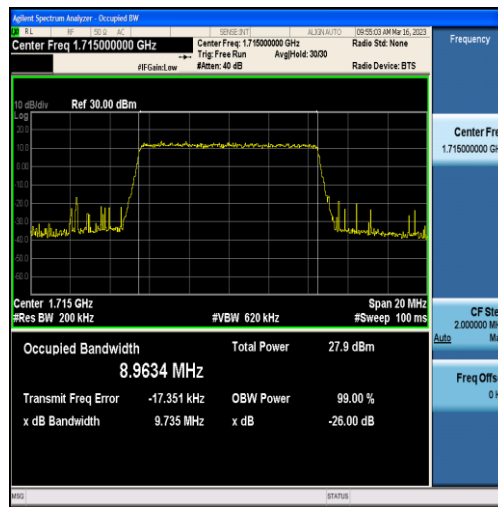
Band4-10MHz-QPSK-20000-50RB#0-8.9634
