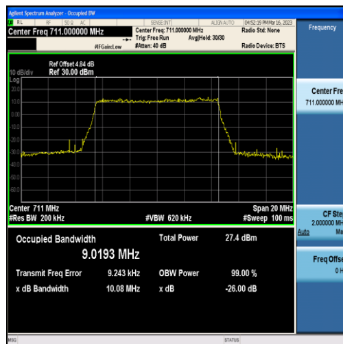
Band12-10MHz-16QAM-23130-50RB#0-9.0193
