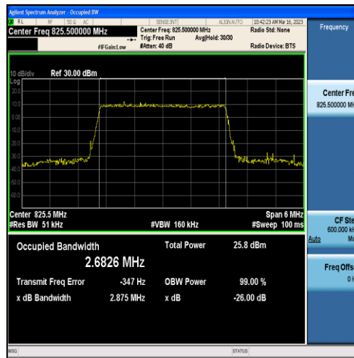
Band5-3MHz-16QAM-20415-15RB#0-2.6826
