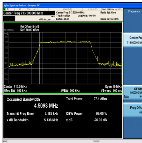
Band12-5MHz-16QAM-23155-25RB#0-4.5093
