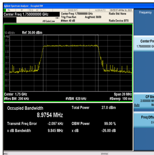
Band4-10MHz-16QAM-20350-50RB#0-8.9754
