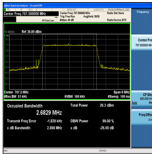
Band12-3MHz-16QAM-23095-15RB#0-2.6829
