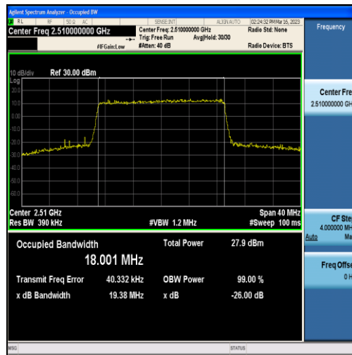
Band7-20MHz-16QAM-20850-100RB#0-18.001
