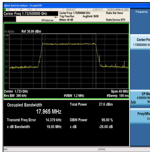
Band4-20MHz-16QAM-20175-100RB#0-17.965
