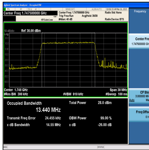
Band4-15MHz-QPSK-20325-75RB#0-13.440
