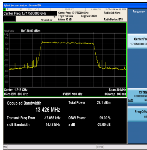
Band4-15MHz-QPSK-20025-75RB#0-13.426
