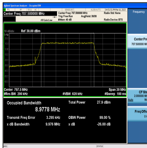
Band12-10MHz-QPSK-23095-50RB#0-8.9778
