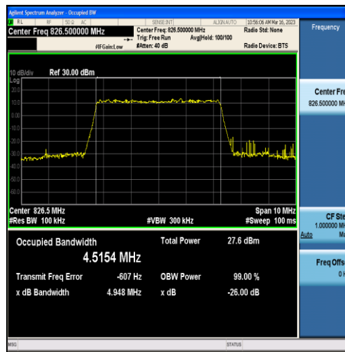
Band5-5MHz-QPSK-20425-25RB#0-4.5154
