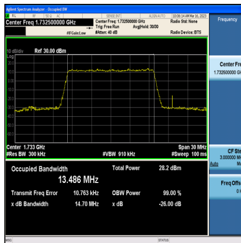
Band4-15MHz-QPSK-20175-75RB#0-13.486
