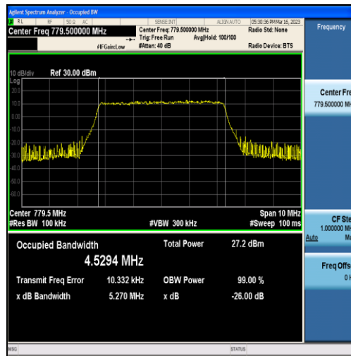
Band13-5MHz-16QAM-23205-25RB#0-4.5294
