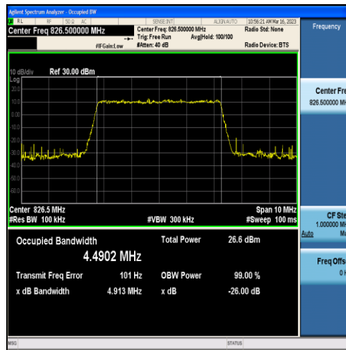
Band5-5MHz-16QAM-20425-25RB#0-4.4902
