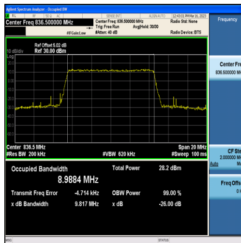
Band5-10MHz-QPSK-20525-50RB#0-8.9884
