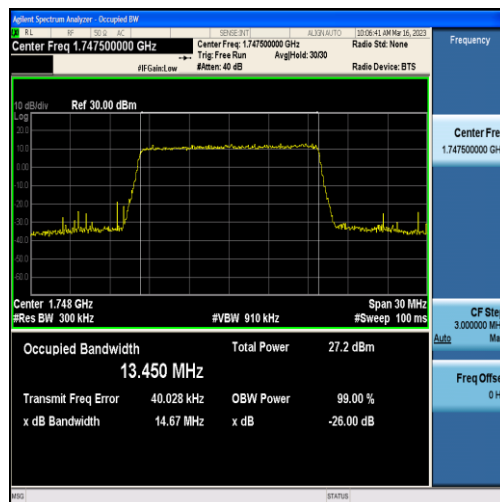
Band4-15MHz-16QAM-20325-75RB#0-13.450
