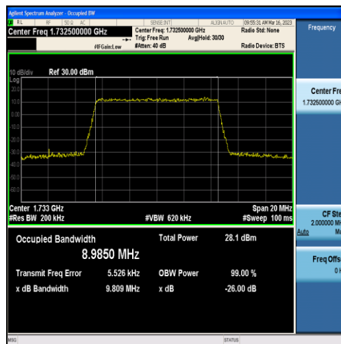
Band4-10MHz-QPSK-20175-50RB#0-8.9850
