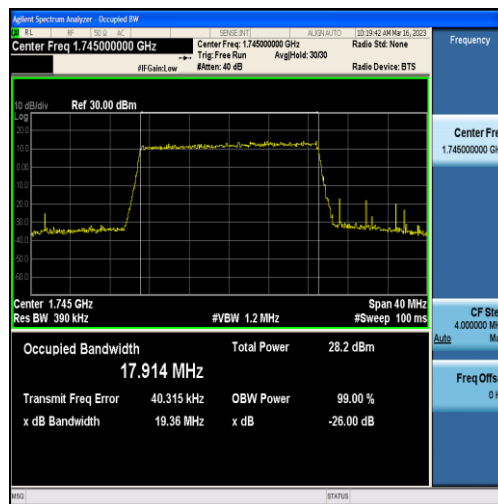
Band4-20MHz-QPSK-20300-100RB#0-17.914
