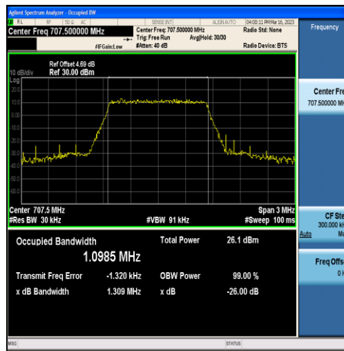
Band12-1.4MHz-16QAM-23095-6RB#0-1.0985
