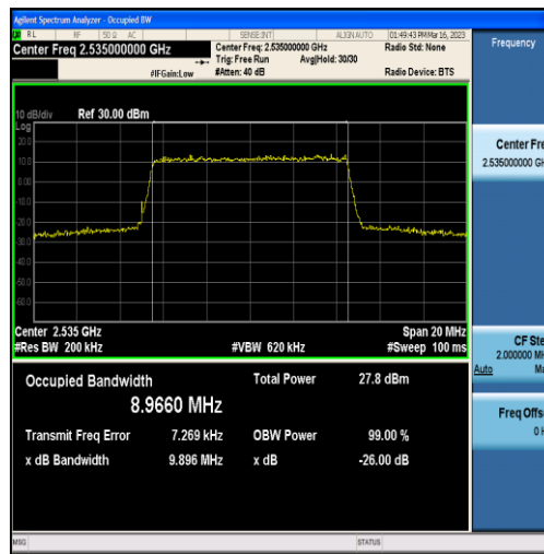
Band7-10MHz-16QAM-21100-50RB#0-8.9660
