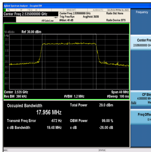
Band7-20MHz-QPSK-21100-100RB#0-17.956
