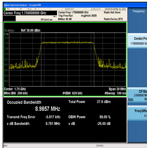
Band4-10MHz-QPSK-20350-50RB#0-8.9857
