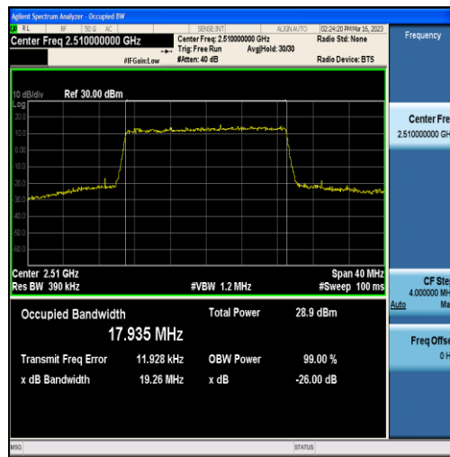
Band7-20MHz-QPSK-20850-100RB#0-17.935
