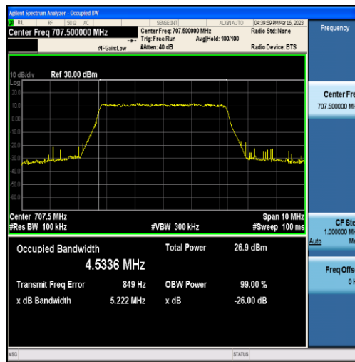
Band12-5MHz-16QAM-23095-25RB#0-4.5336
