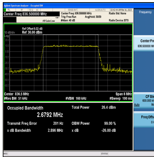
Band5-3MHz-16QAM-20525-15RB#0-2.6792
