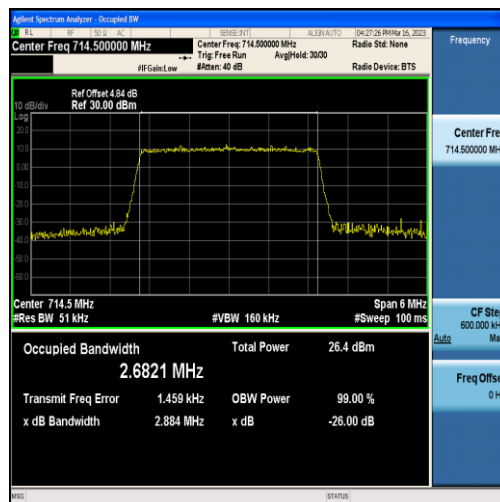
Band12-3MHz-16QAM-23165-15RB#0-2.6821
