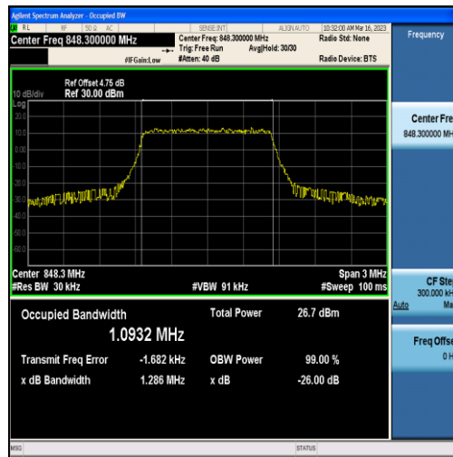
Band5-1.4MHz-QPSK-20643-6RB#0-1.0932
