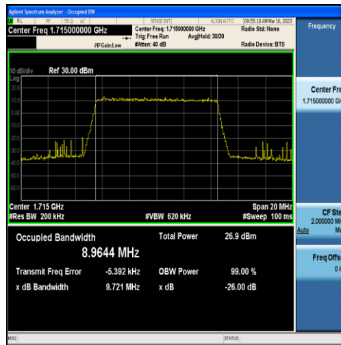
Band4-10MHz-16QAM-20000-50RB#0-8.9644
