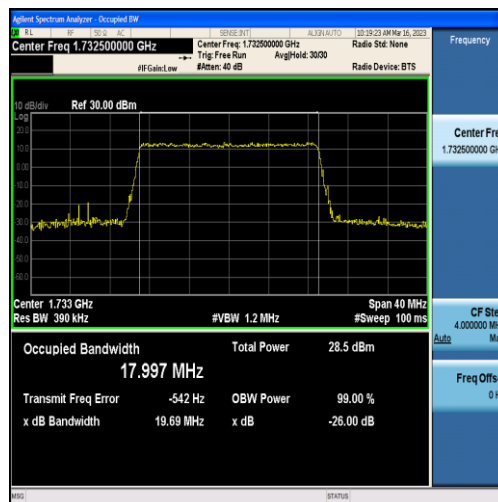
Band4-20MHz-QPSK-20175-100RB#0-17.997
