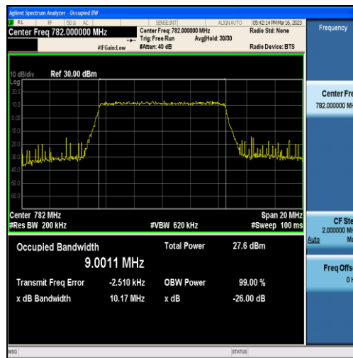
Band13-10MHz-QPSK-23230-50RB#0-9.0011
