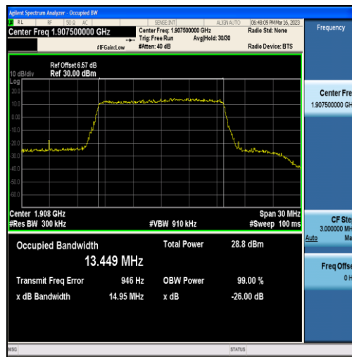
Band25-15MHz-QPSK-26615-75RB#0-13.449
