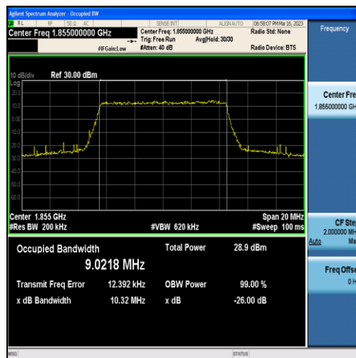
Band25-10MHz-QPSK-26090-50RB#0-9.0218
