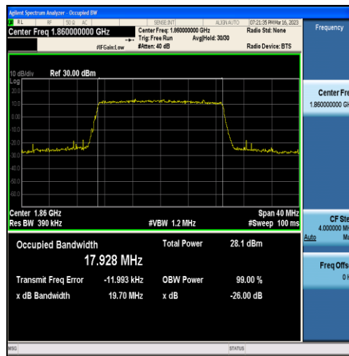
Band25-20MHz-16QAM-26140-100RB#0-17.928
