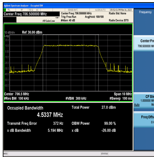
Band17-5MHz-16QAM-23755-25RB#0-4.5337
