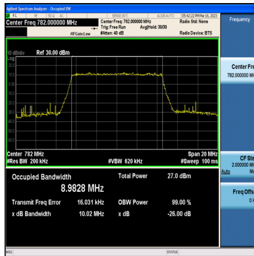
Band13-10MHz-16QAM-23230-50RB#0-8.9828
