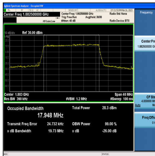
Band25-20MHz-16QAM-26365-100RB#0-17.948
