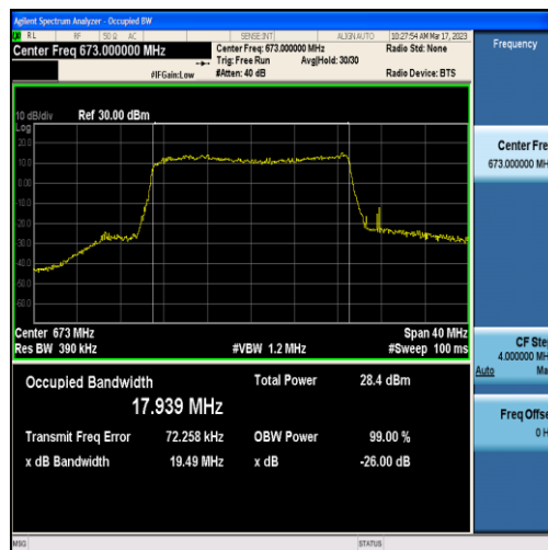
Band71-20MHz-QPSK-133222-100RB#0-17.939
