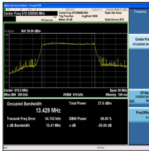
Band71-15MHz-16QAM-133197-75RB#0-13.429
