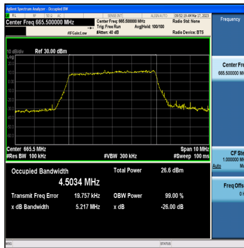
Band71-5MHz-16QAM-133147-25RB#0-4.5034
