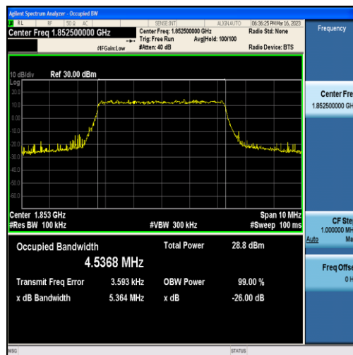
Band25-5MHz-QPSK-26065-25RB#0-4.5368
