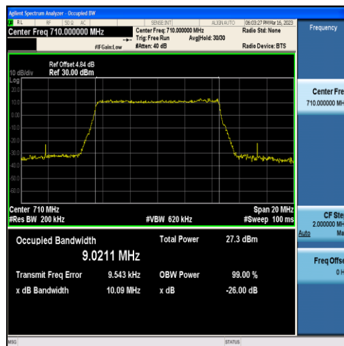
Band17-10MHz-16QAM-23790-50RB#0-9.0211
