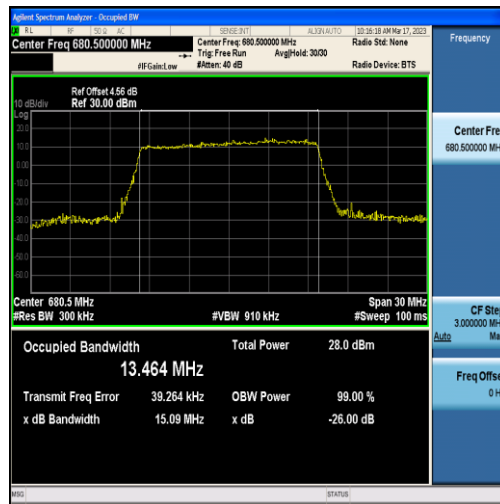
Band71-15MHz-QPSK-133297-75RB#0-13.464
