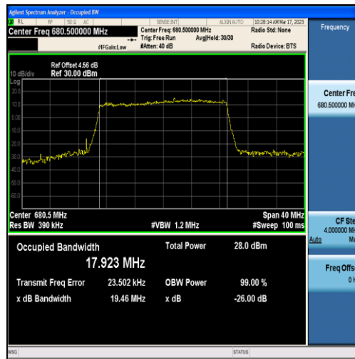
Band71-20MHz-QPSK-133297-100RB#0-17.923
