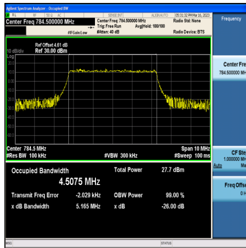
Band13-5MHz-QPSK-23255-25RB#0-4.5075
