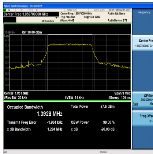
Band25-1.4MHz-QPSK-26047-6RB#0-1.0928
