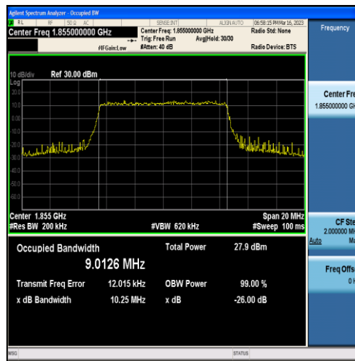
Band25-10MHz-16QAM-26090-50RB#0-9.0126
