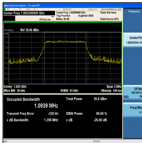
Band25-1.4MHz-16QAM-26365-6RB#0-1.0939
