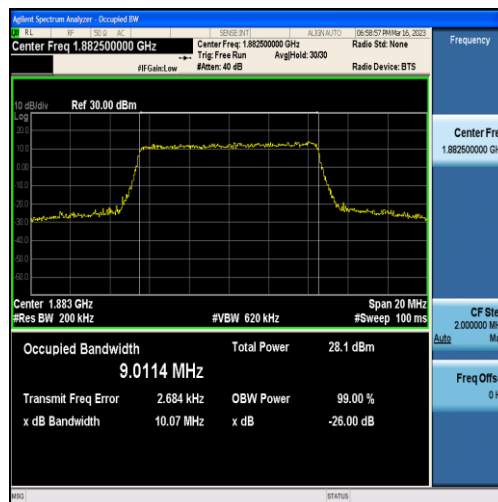
Band25-10MHz-16QAM-26365-50RB#0-9.0114
