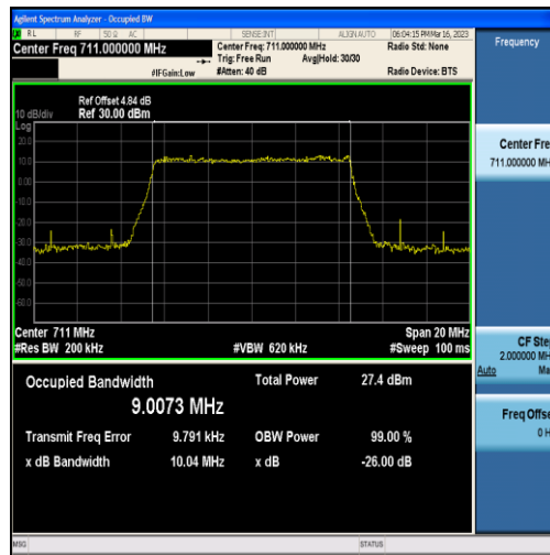
Band17-10MHz-16QAM-23800-50RB#0-9.0073
