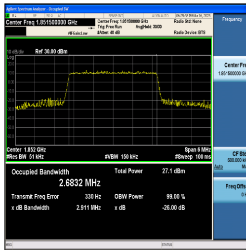
Band25-3MHz-16QAM-26055-15RB#0-2.6832
