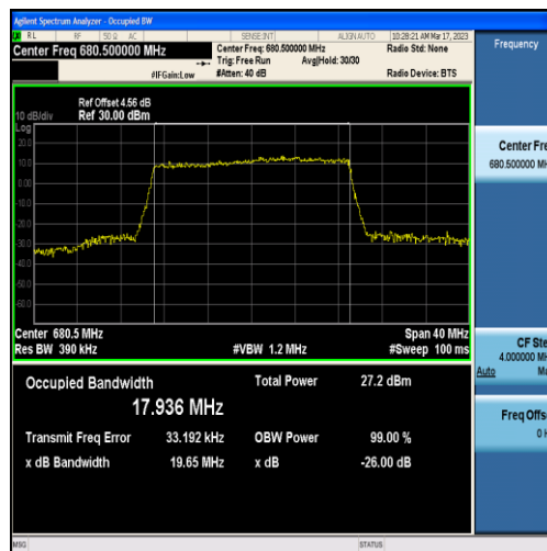
Band71-20MHz-16QAM-133297-100RB#0-17.936
