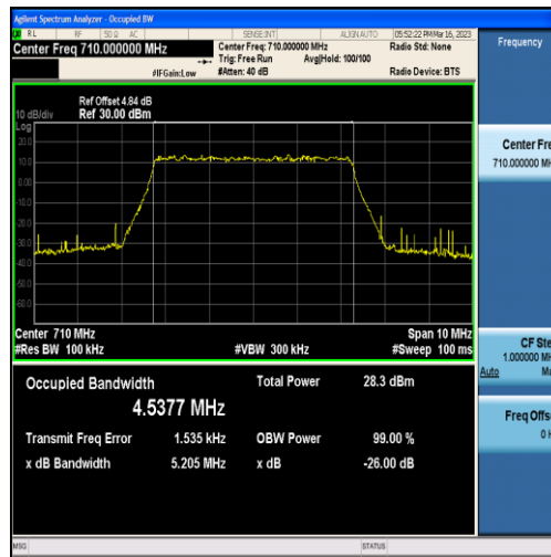
Band17-5MHz-QPSK-23790-25RB#0-4.5377
