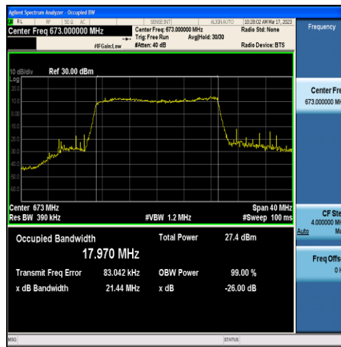
Band71-20MHz-16QAM-133222-100RB#0-17.970
