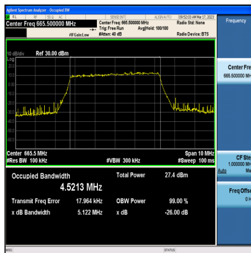
Band71-5MHz-QPSK-133147-25RB#0-4.5213
