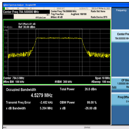
Band13-5MHz-16QAM-23255-25RB#0-4.5279
