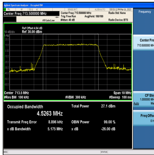
Band17-5MHz-16QAM-23825-25RB#0-4.5263
