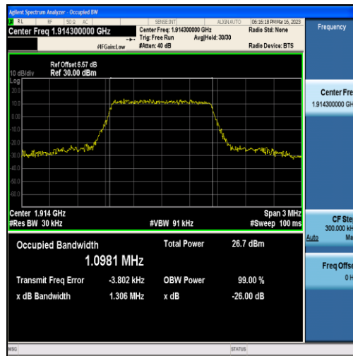
Band25-1.4MHz-16QAM-26683-6RB#0-1.0981
