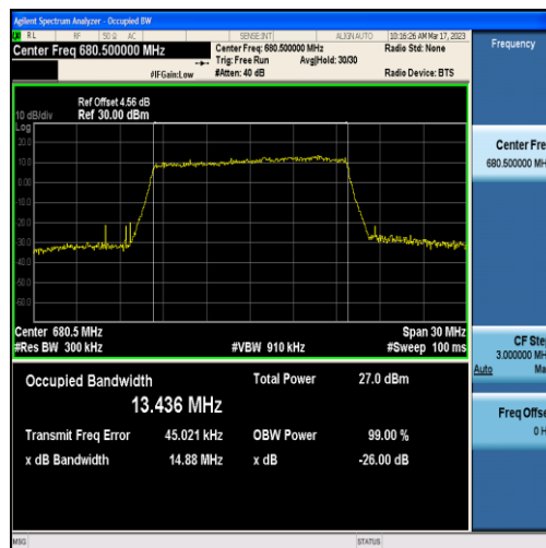
Band71-15MHz-16QAM-133297-75RB#0-13.436
