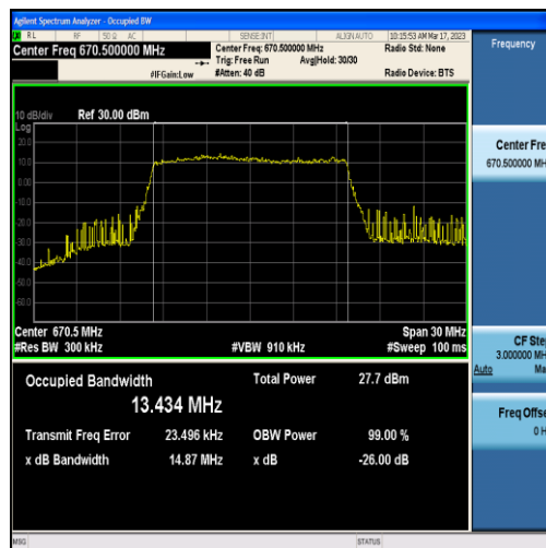
Band71-15MHz-QPSK-133197-75RB#0-13.434
