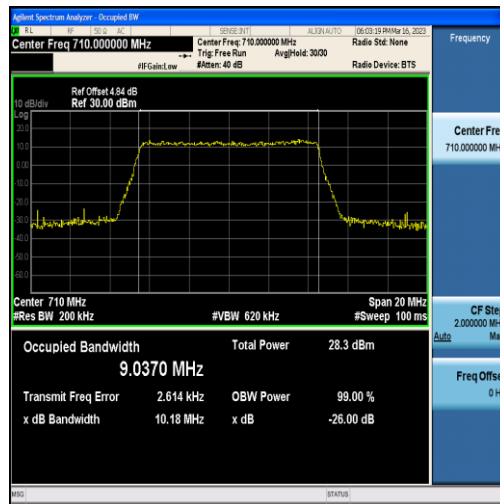
Band17-10MHz-QPSK-23790-50RB#0-9.0370
