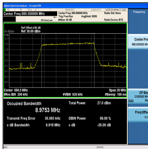
Band71-10MHz-16QAM-133297-50RB#0-8.9753
