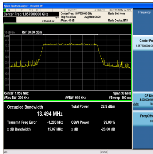
Band25-15MHz-QPSK-26115-75RB#0-13.494
