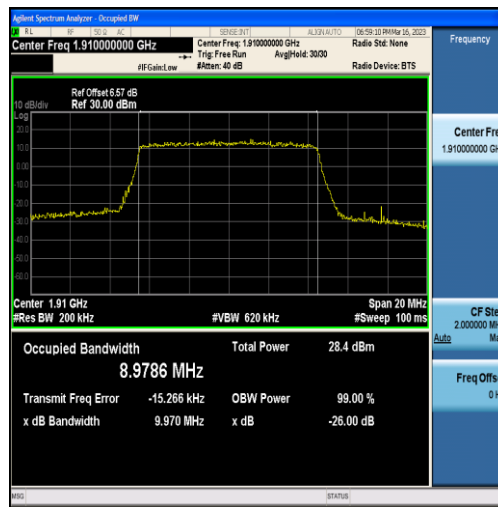
Band25-10MHz-QPSK-26640-50RB#0-8.9786
