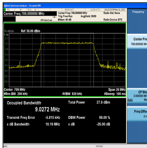
Band17-10MHz-QPSK-23780-50RB#0-9.0272
