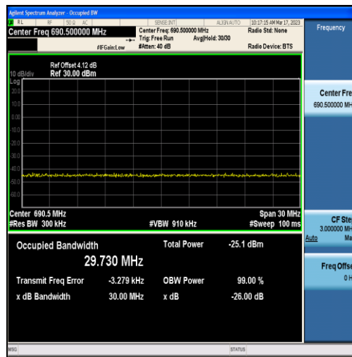
Band71-15MHz-QPSK-133397-75RB#0-29.730
