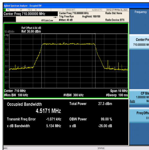
Band17-5MHz-16QAM-23790-25RB#0-4.5171
