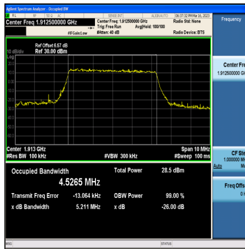
Band25-5MHz-QPSK-26665-25RB#0-4.5265
