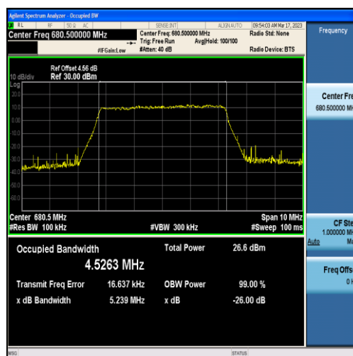
Band71-5MHz-16QAM-133297-25RB#0-4.5263
