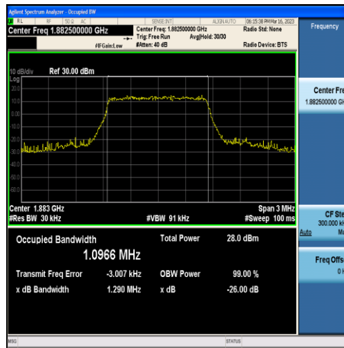
Band25-1.4MHz-QPSK-26365-6RB#0-1.0966
