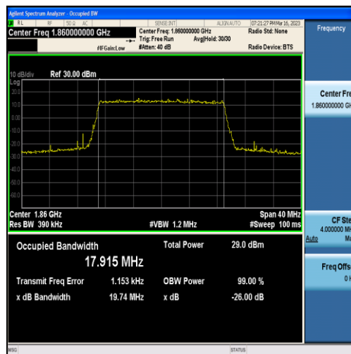
Band25-20MHz-QPSK-26140-100RB#0-17.915
