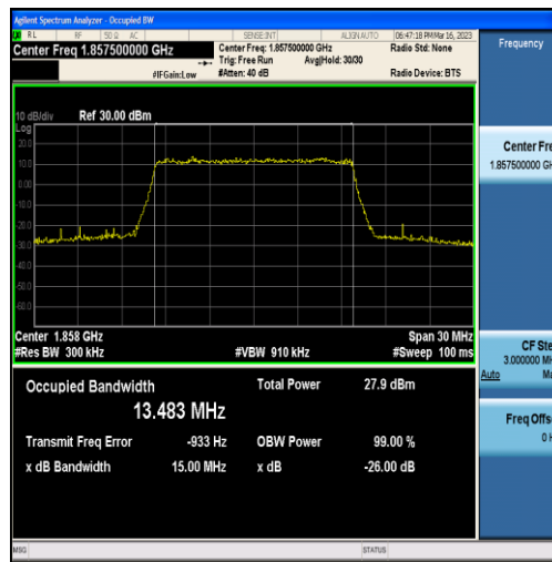
Band25-15MHz-16QAM-26115-75RB#0-13.483
