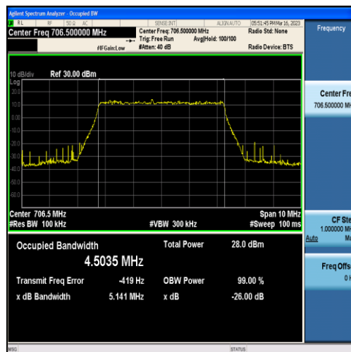
Band17-5MHz-QPSK-23755-25RB#0-4.5035
