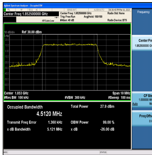
Band25-5MHz-16QAM-26065-25RB#0-4.5120
