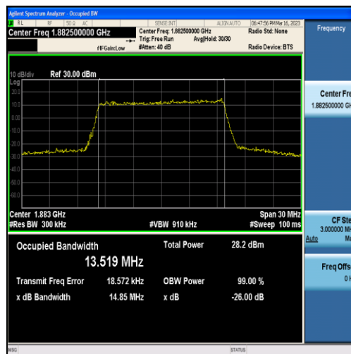
Band25-15MHz-16QAM-26365-75RB#0-13.519
