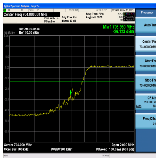
Band17-5MHz-16QAM-23755-25RB#0
