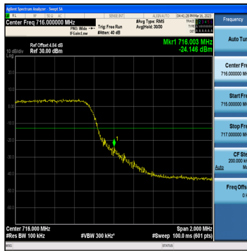
Band12-5MHz-QPSK-23155-25RB#0
