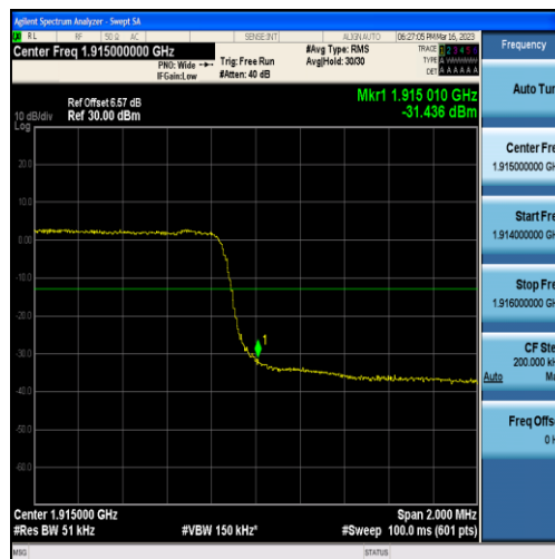
Band25-3MHz-QPSK-26675-15RB#0
