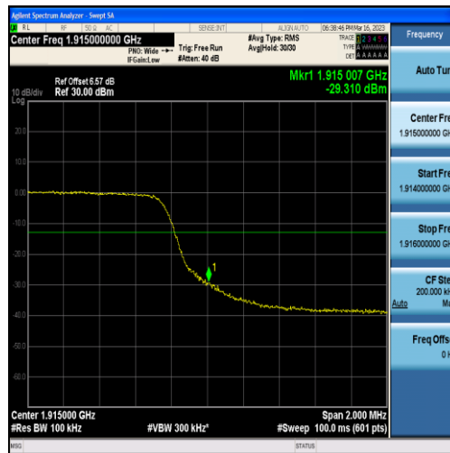
Band25-5MHz-16QAM-26665-25RB#0
