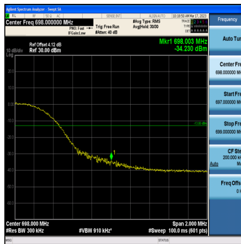
Band71-15MHz-16QAM-133397-75RB#0
