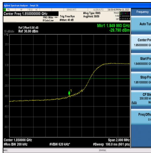
Band25-10MHz-QPSK-26090-50RB#0
