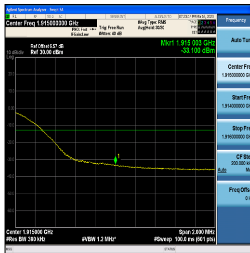
Band25-20MHz-16QAM-26590-100RB#0
