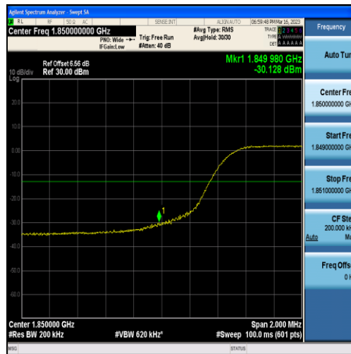
Band25-10MHz-16QAM-26090-50RB#0
