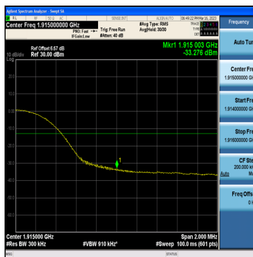
Band25-15MHz-16QAM-26615-75RB#0
