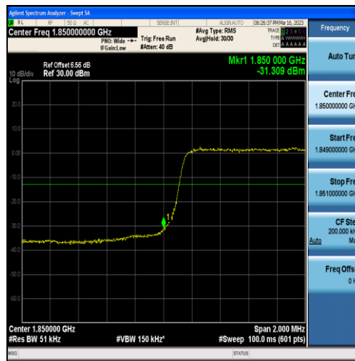
Band25-3MHz-QPSK-26055-15RB#0
