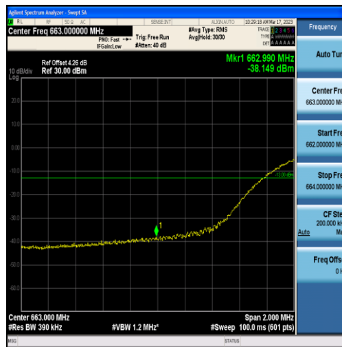
Band71-20MHz-16QAM-133222-100RB#0
