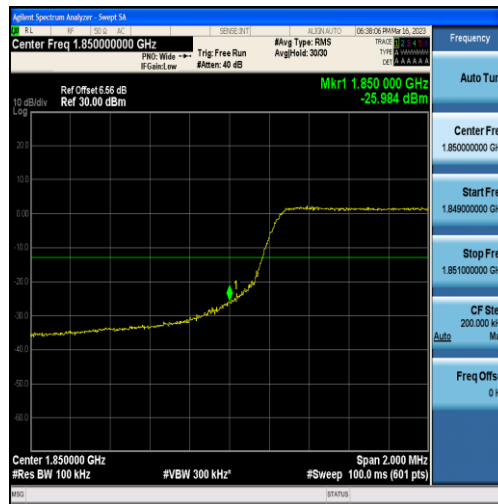
Band25-5MHz-QPSK-26065-25RB#0
