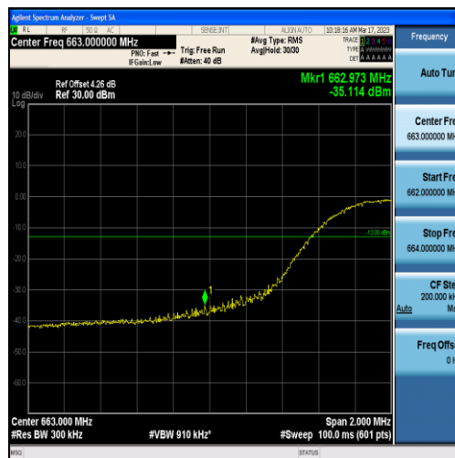
Band71-15MHz-16QAM-133197-75RB#0
