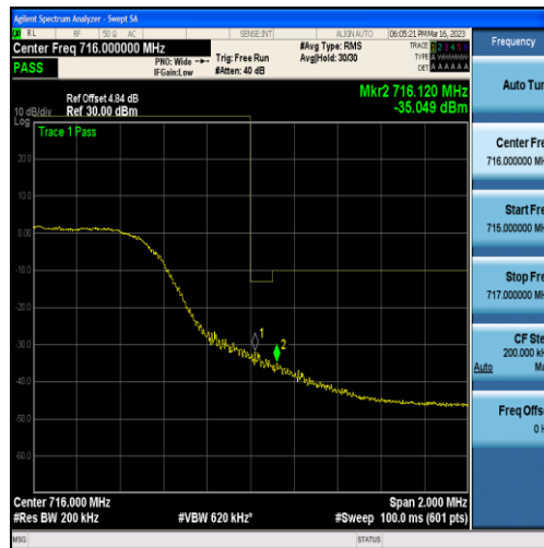
Band17-10MHz-16QAM-23800-50RB#0
