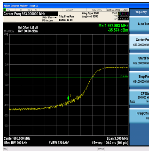
Band71-10MHz-16QAM-133172-50RB#0
