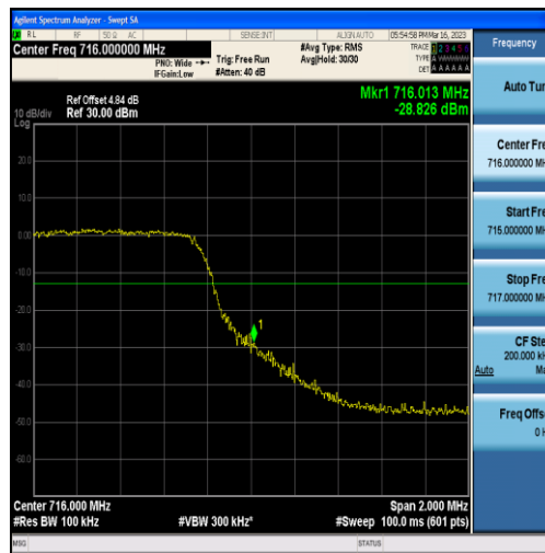
Band17-5MHz-16QAM-23825-25RB#0
