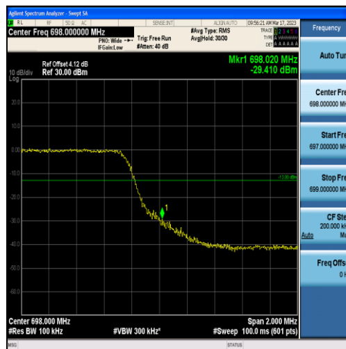
Band71-5MHz-16QAM-133447-25RB#0
