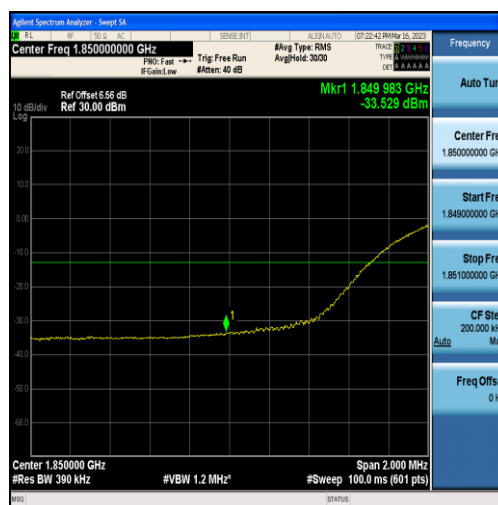
Band25-20MHz-16QAM-26140-100RB#0
