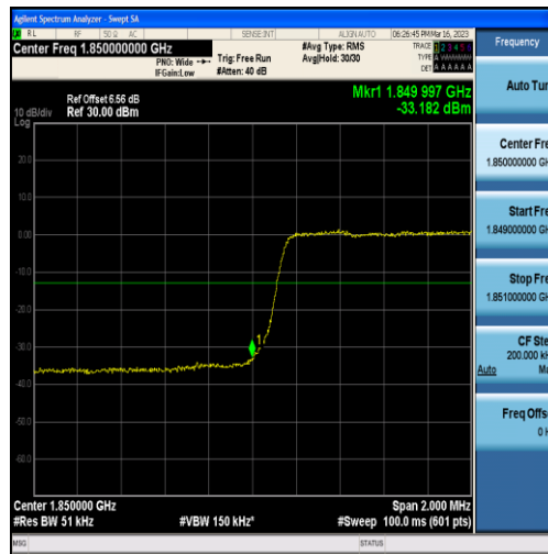
Band25-3MHz-16QAM-26055-15RB#0
