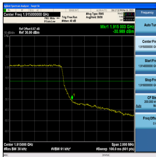
Band25-1.4MHz-16QAM-26683-6RB#0
