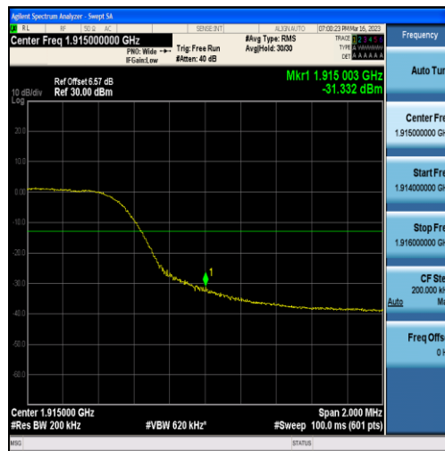
Band25-10MHz-16QAM-26640-50RB#0
