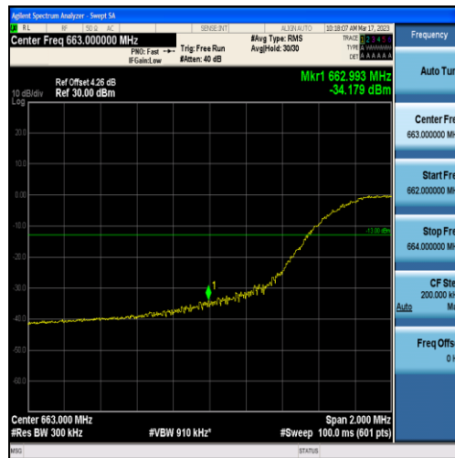
Band71-15MHz-QPSK-133197-75RB#0
