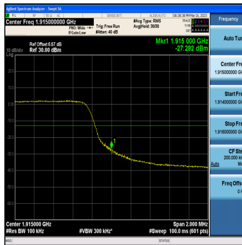
Band25-5MHz-QPSK-26665-25RB#0
