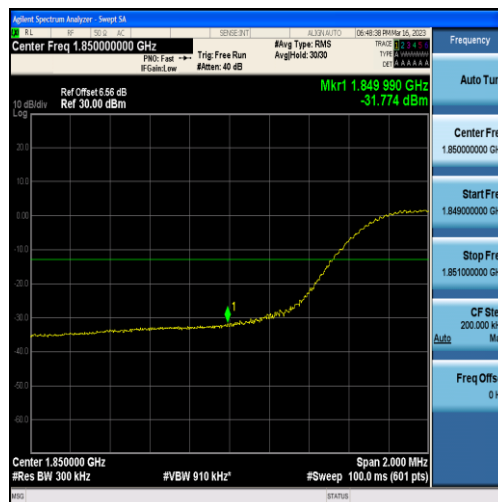
Band25-15MHz-QPSK-26115-75RB#0
