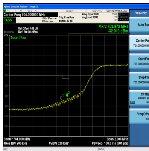
Band17-10MHz-16QAM-23780-50RB#0
