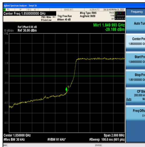
Band25-1.4MHz-QPSK-26047-6RB#0
