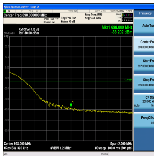
Band71-20MHz-16QAM-133372-100RB#0
