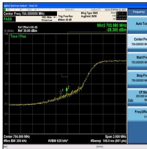
Band17-10MHz-QPSK-23780-50RB#0
