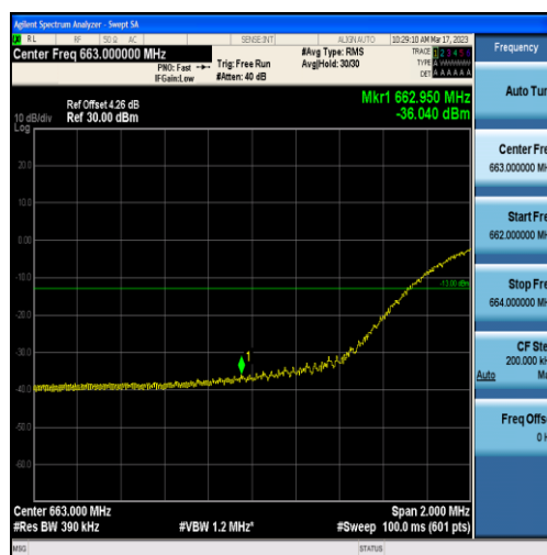
Band71-20MHz-QPSK-133222-100RB#0
