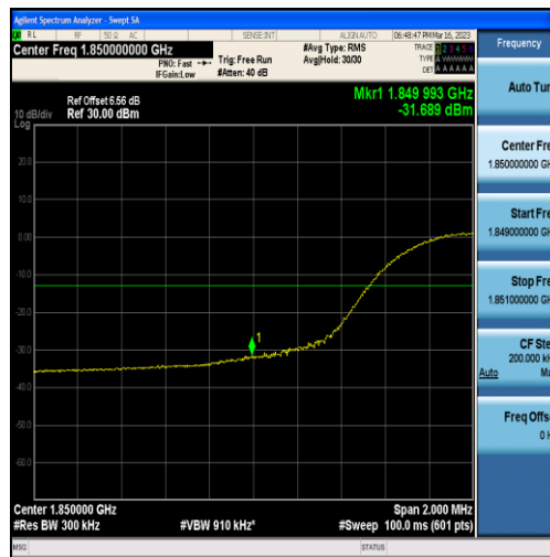
Band25-15MHz-16QAM-26115-75RB#0
