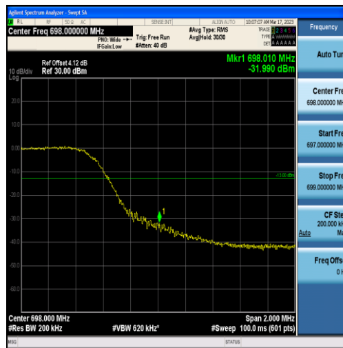
Band71-10MHz-16QAM-133422-50RB#0
