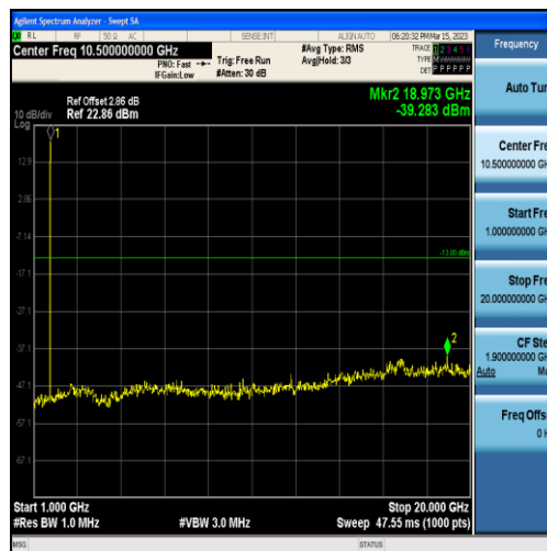
Band4-1.4MHz-16QAM-20175-6RB#0-Range2:1000~20000MHz
