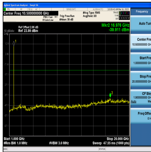
Band4-15MHz-16QAM-20025-75RB#0-Range2:1000~20000MHz
