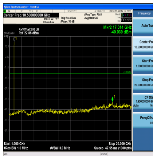
Band4-3MHz-16QAM-20175-15RB#0-Range2:1000~20000MHz
