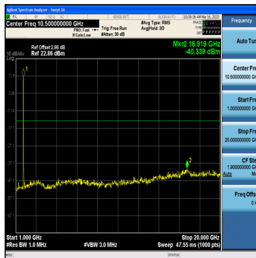
Band4-15MHz-QPSK-20025-75RB#0-Range2:1000~20000MHz
