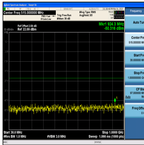
Band7-5MHz-16QAM-21425-25RB#0-Range1:30~1000MHz
