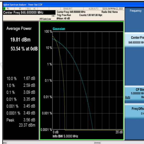
Band5-4233
