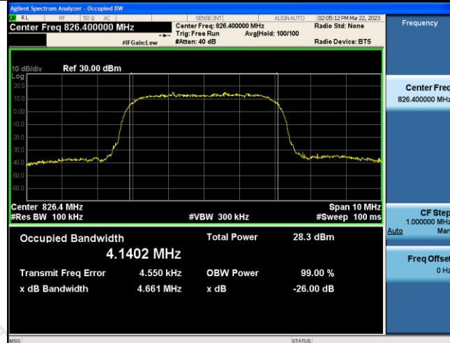
Channel 4132
