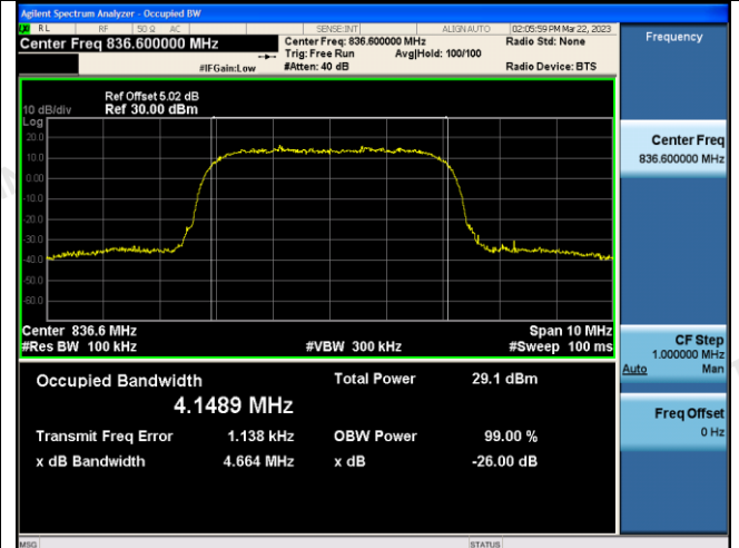
Channel 4183
