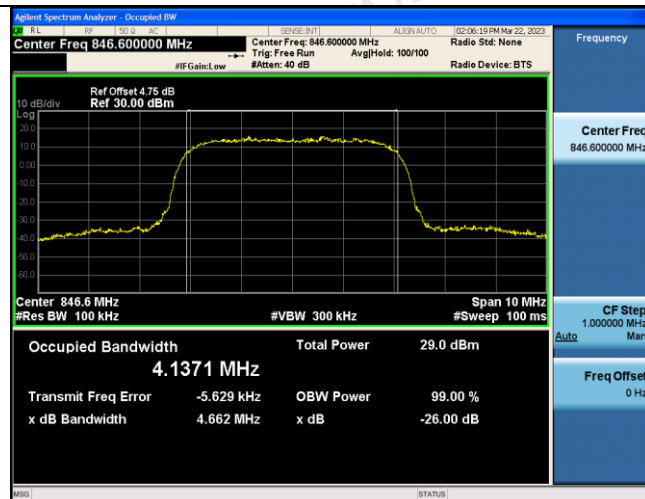
Channel 4233
