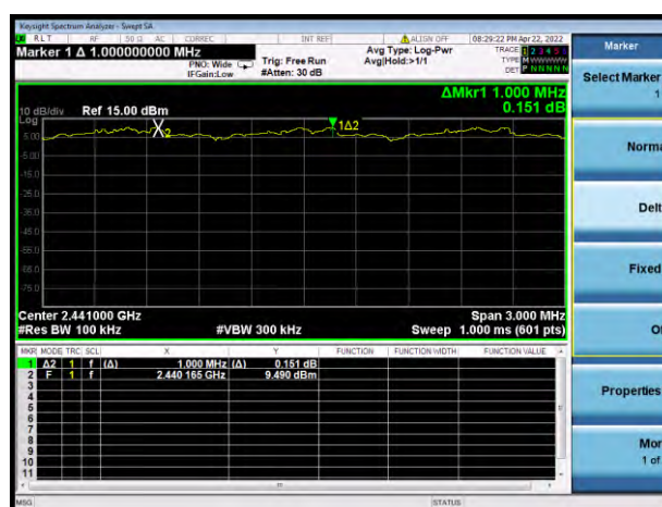
8-DPSK
