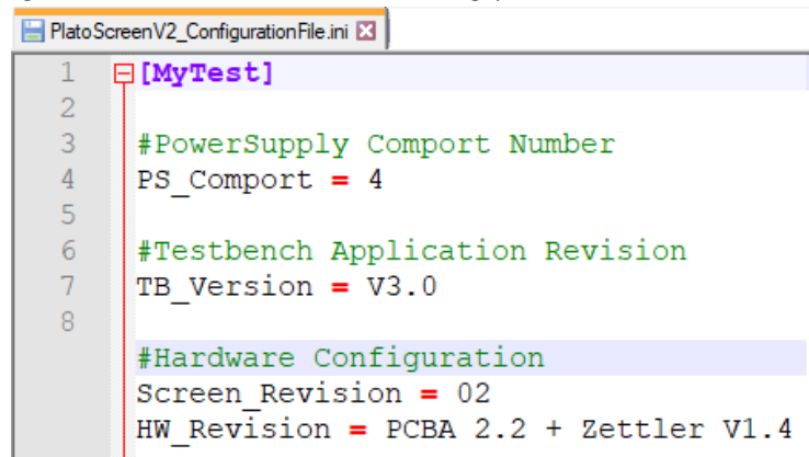
Figure 27 : Configuration File
