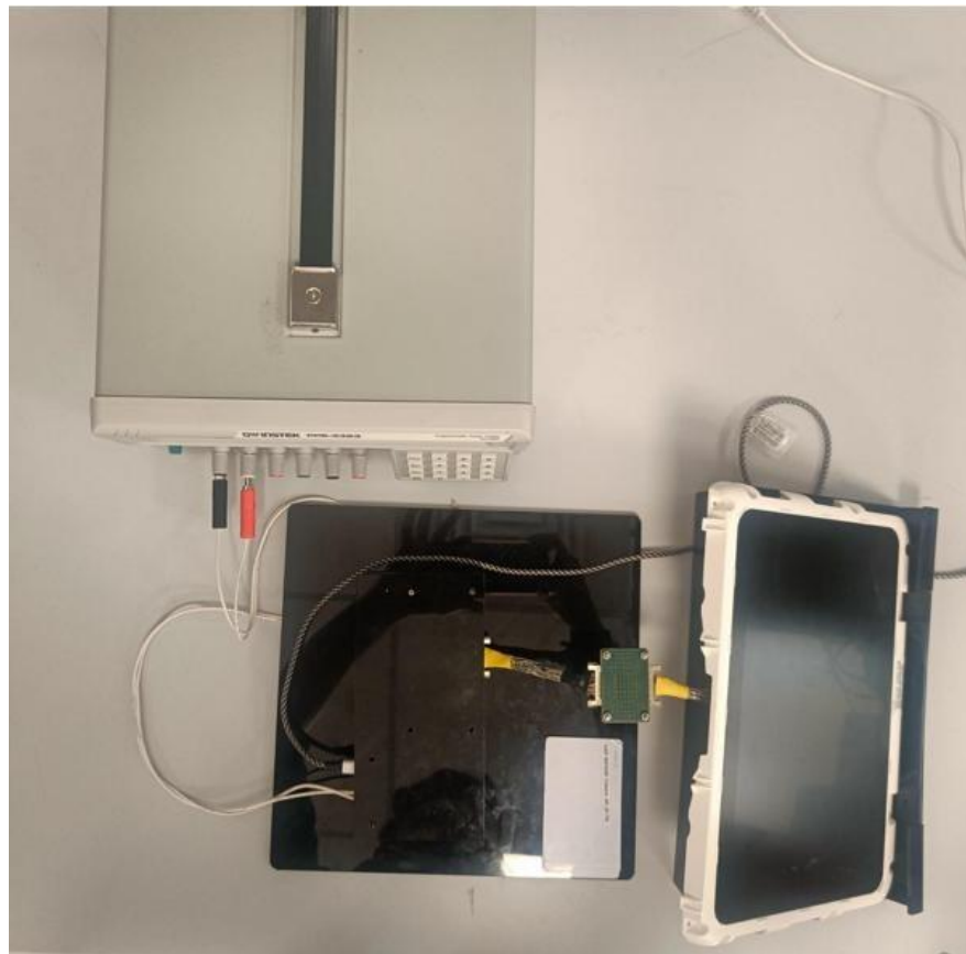
Figure 14 : Top View
