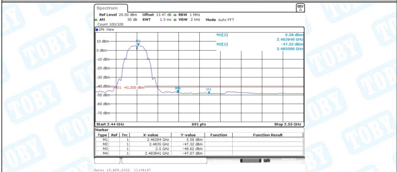
11B_Ant1_High_2462_AV
