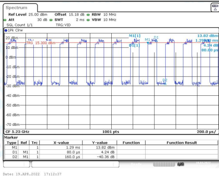
11AC40SISO_Ant1_5230
