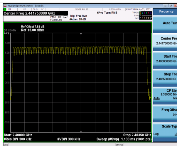
GFSK Modulation
