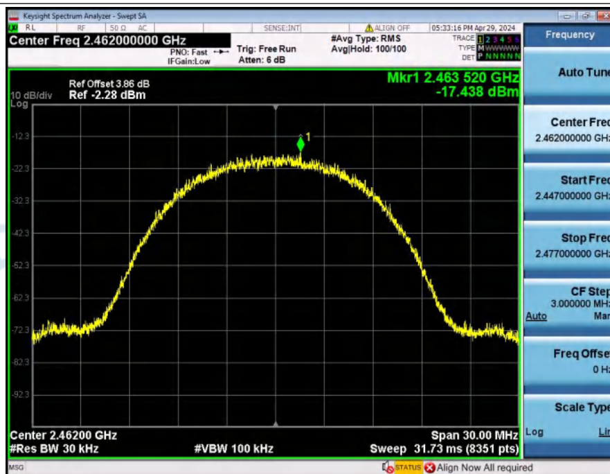
Power_Spectral_Density_NVNT_ANT1_802_11b_2462
