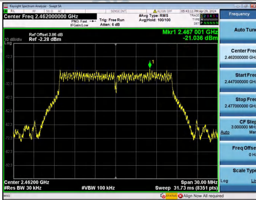
Power_Spectral_Density_NVNT_ANT1_802_11g_2462
