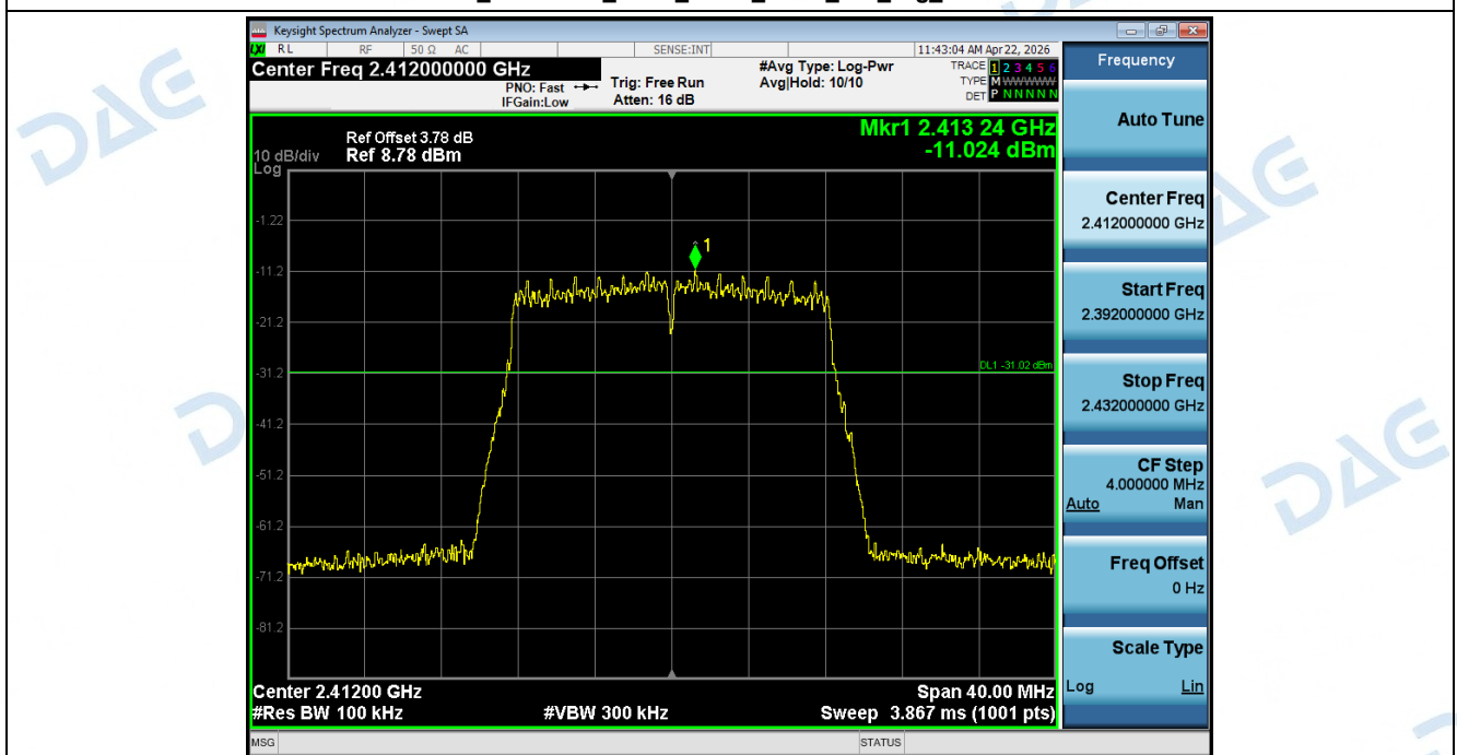
2_Spurious_Emission_NVNT_ANT1_802_11g_2412
