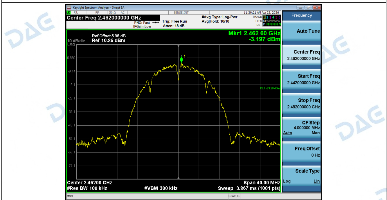
2_Spurious_Emission_NVNT_ANT1_802_11b_2462
