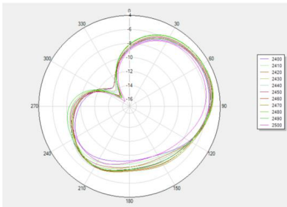
Theta 90 2D
