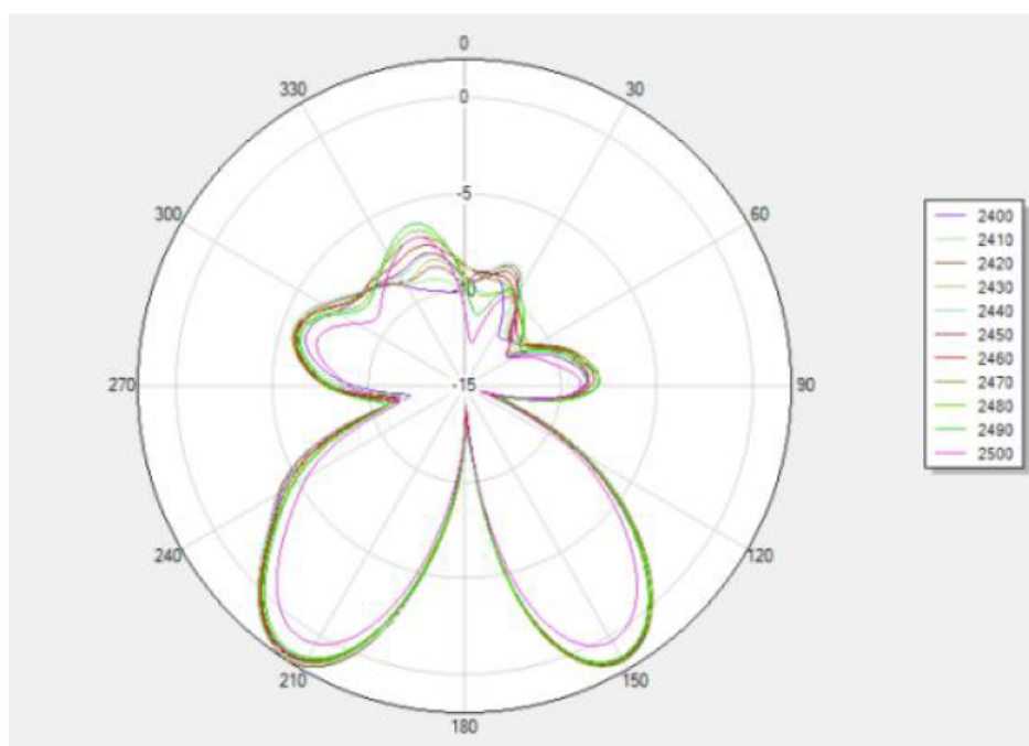
Phi 0 2D
