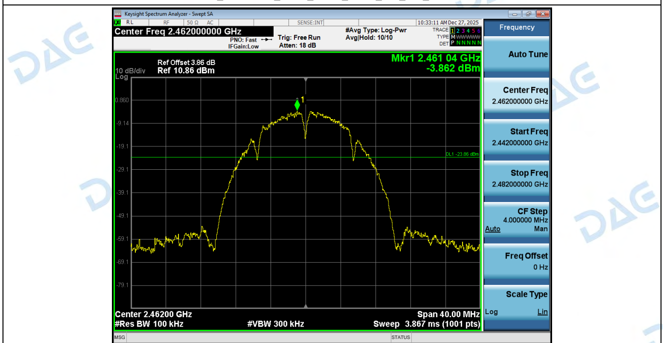
2 Bandedge_NVNT_ANT1_802_11b_2462
