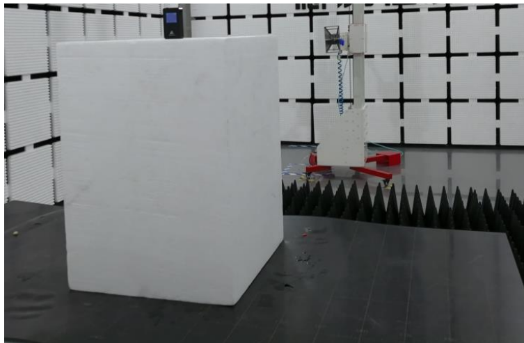
Radiated emission above 1GHz
