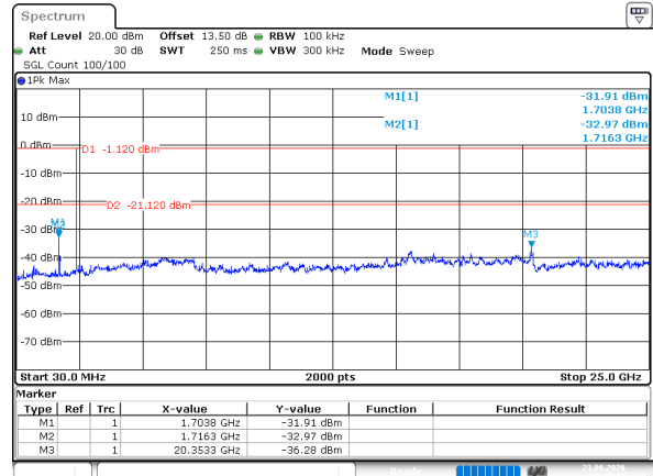
BLE_2M_Low_Channel
