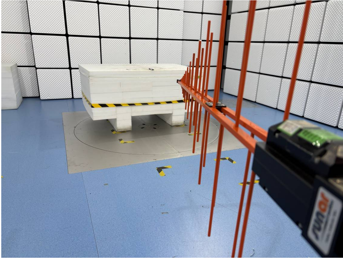
RE – Front View (1 GHz~5 GHz)
