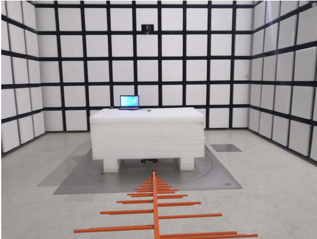
Radiated Emissions Below 1G front View
