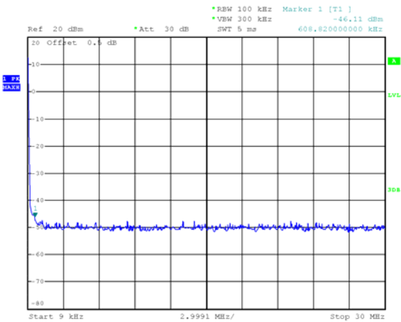
Mode: channel 39
