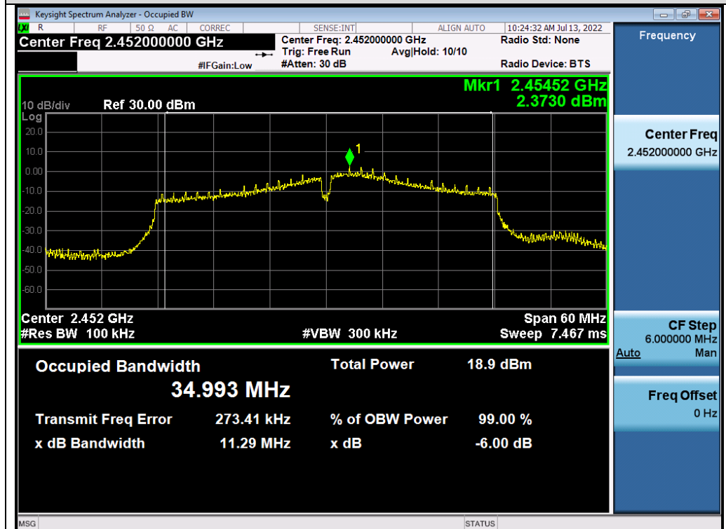
Test_Graph_802.11n40_ANT1_2452_MCS0_DTSBW
