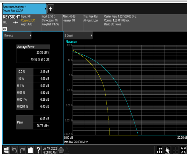
Band2-15MHz-QPSK-18675-5RB#0
