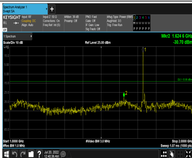
Band4-10MHz-16QAM-20175-1RB#0-Range2:1000~2000MHz
