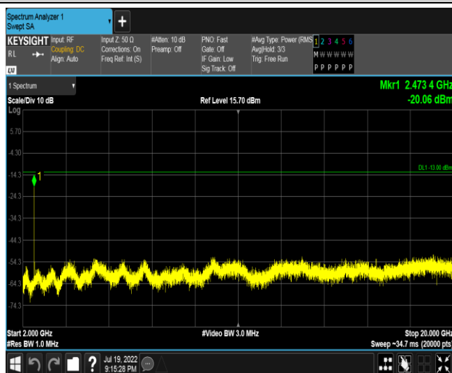
Band5-5MHz-QPSK-20425-1RB#0-Range3:2000~20000MHz
