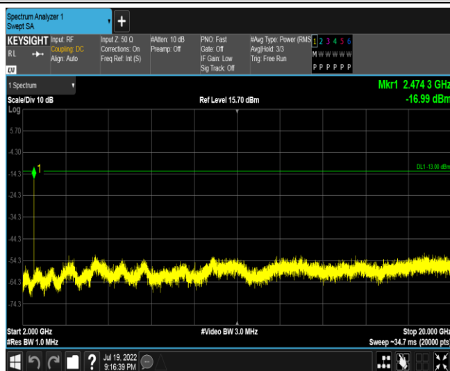
Band5-5MHz-16QAM-20425-1RB#0-Range3:2000~20000MHz
