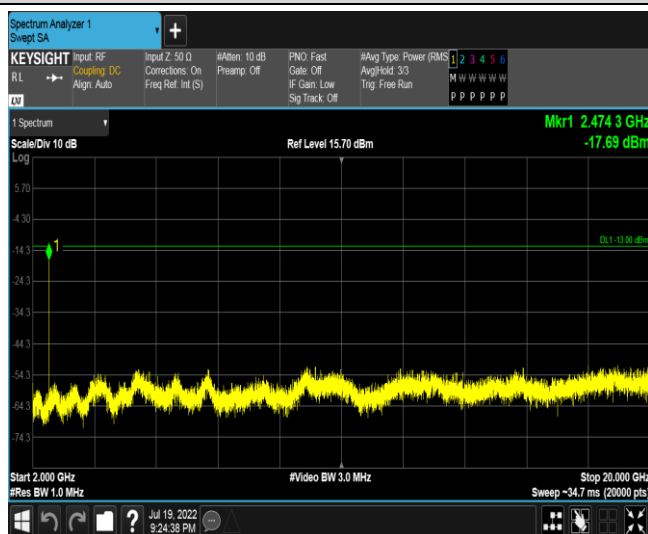
Band5-10MHz-16QAM-20450-1RB#0-Range3:2000~20000MHz
