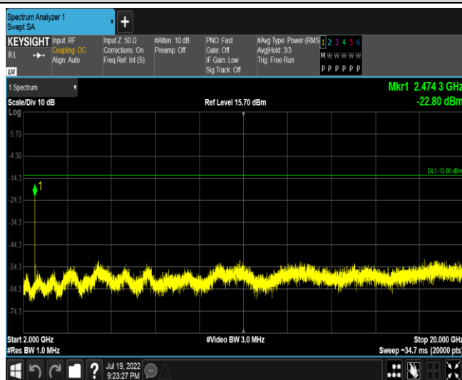
Band5-10MHz-QPSK-20450-1RB#0-Range3:2000~20000MHz
