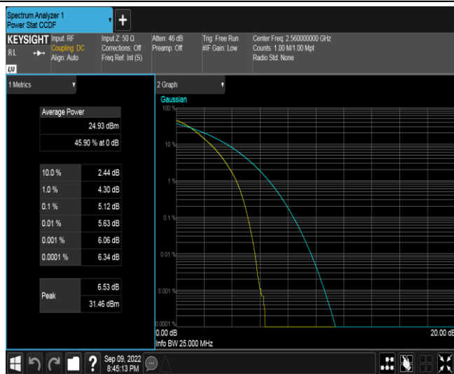
Band7-20MHz-QPSK-21350-100RB#0
