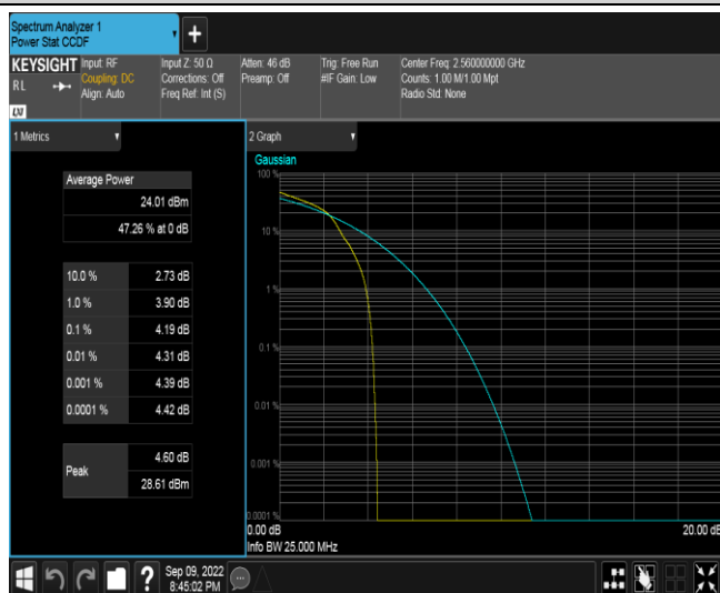
Band7-20MHz-16QAM-21350-1RB#0
