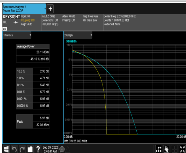
Band7-10MHz-16QAM-21100-50RB#0
