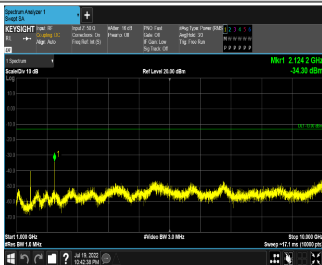
Band17-5MHz-QPSK-23790-1RB#0-Range5:1000~10000MHz
