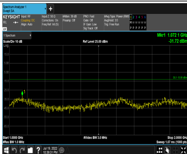
Band17-5MHz-QPSK-23755-1RB#0-Range2:1000~2000MHz
