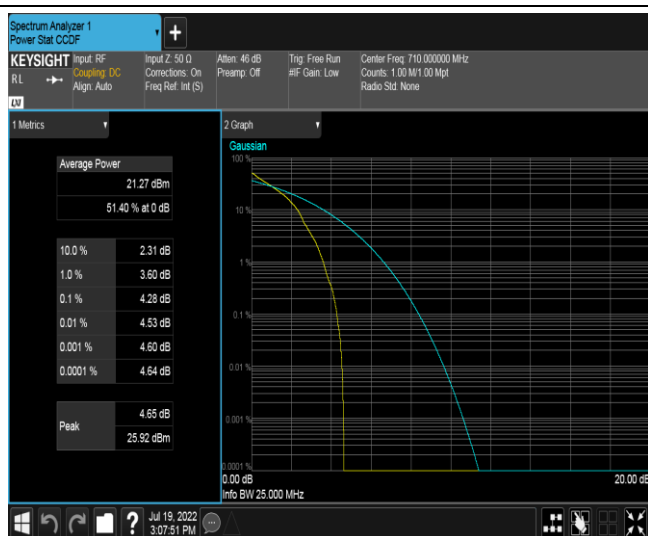
Band17-5MHz-QPSK-23790-25RB#0
