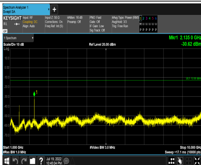
Band17-5MHz-QPSK-23825-1RB#0-Range5:1000~10000MHz
