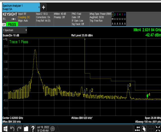
Band38-10MHz-16QAM-38200-1RB#49
