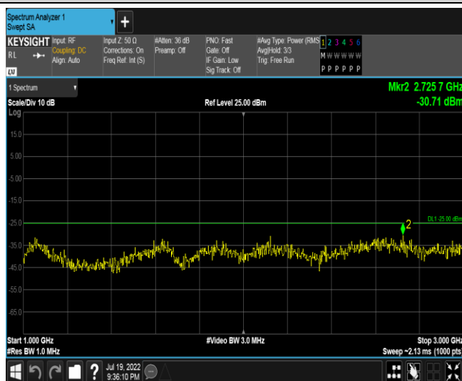
Band38-10MHz-QPSK-37800-1RB#0-Range2:1000~3000MHz
