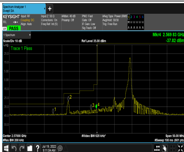
Band38-10MHz-QPSK-37800-1RB#49
