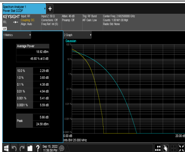
Band41-15MHz-QPSK-41515-75RB#0
