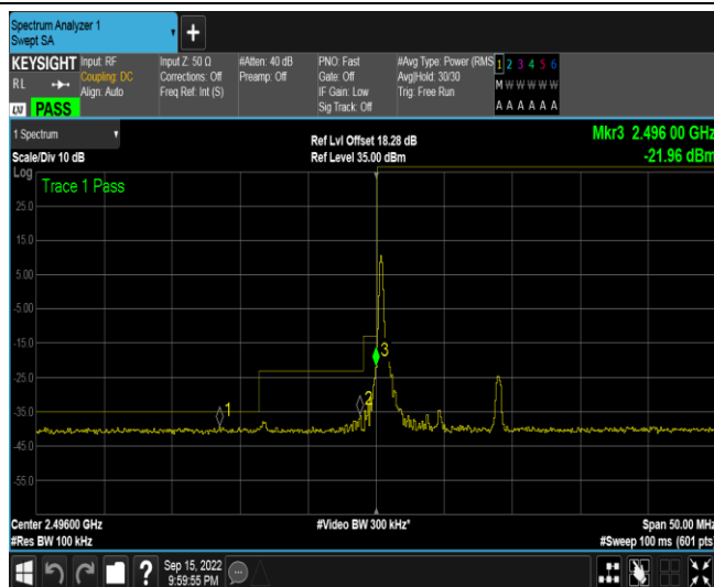
Band41-5MHz-16QAM-39675-1RB#24
