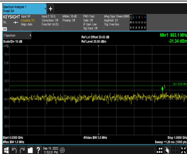
Band41-15MHz-QPSK-41515-1RB#0-Range1:30~1000MHz
