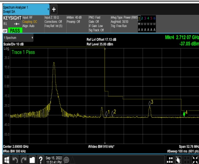
Band41-15MHz-16QAM-41515-1RB#0
