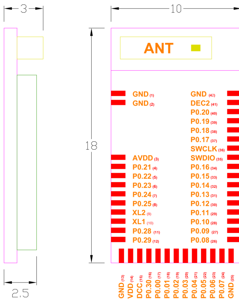
Top (Unit: mm)
