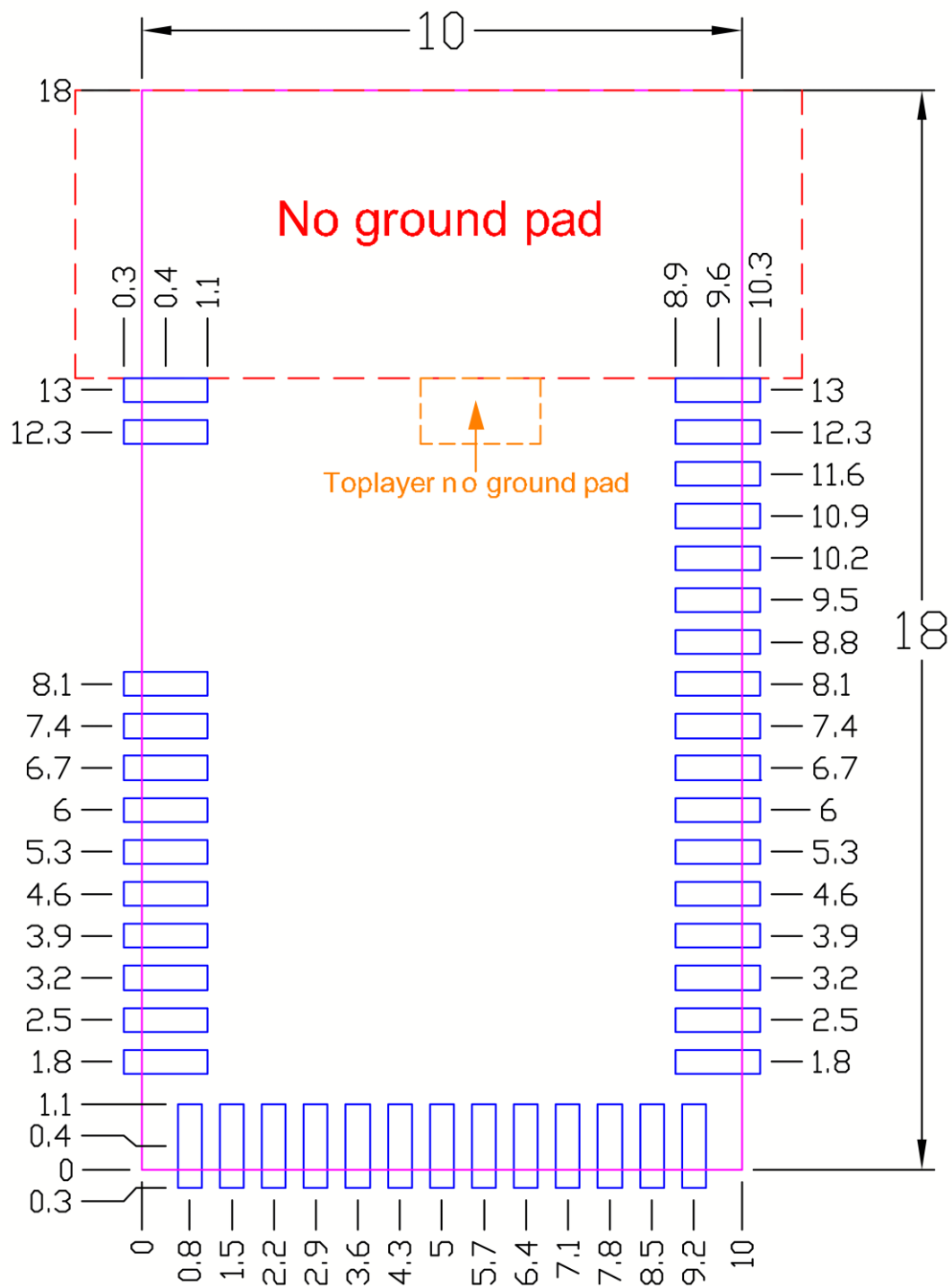
Top View (Unit : mm) recommended solder pad layout
