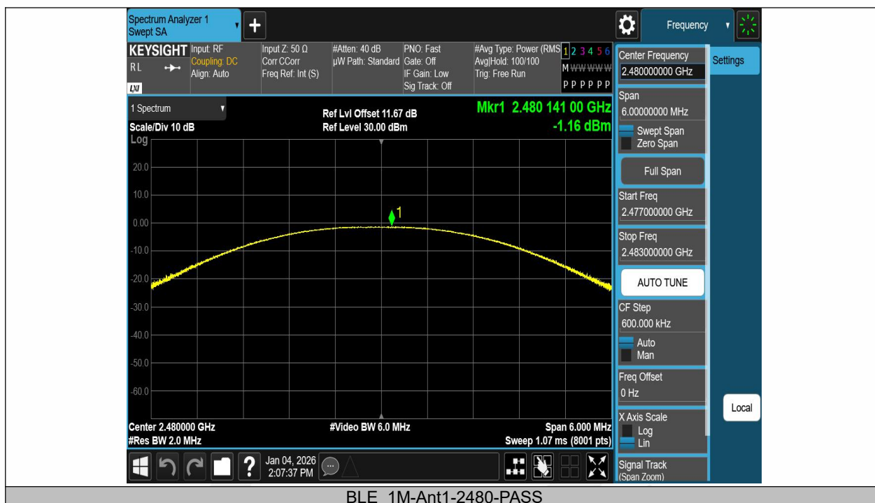
BLE_1M-Ant1-2480-PASS
