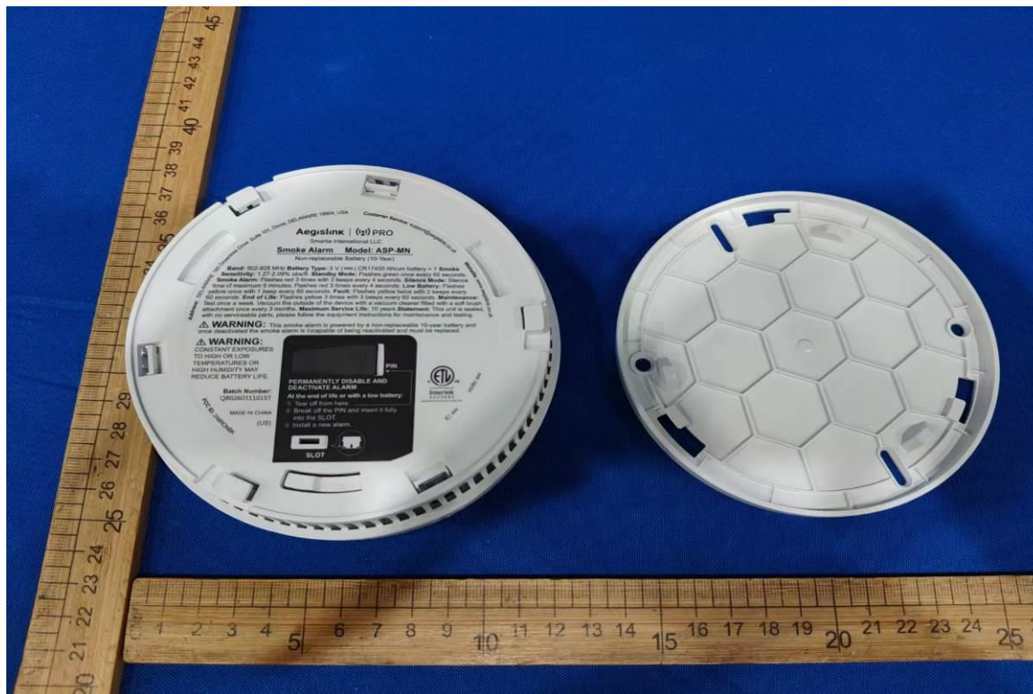
EUT Photo (28)
