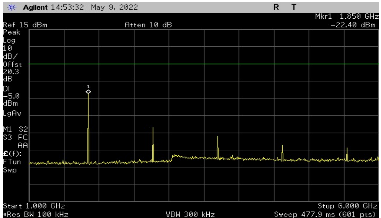
Plot 18 – High Band – 1GHz to 6GHz
