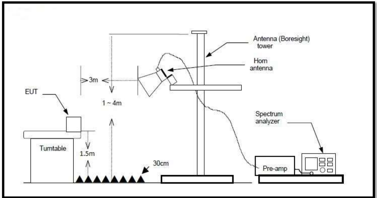
Figure 6. Radiated Emission Above 1GHz Test Setup
