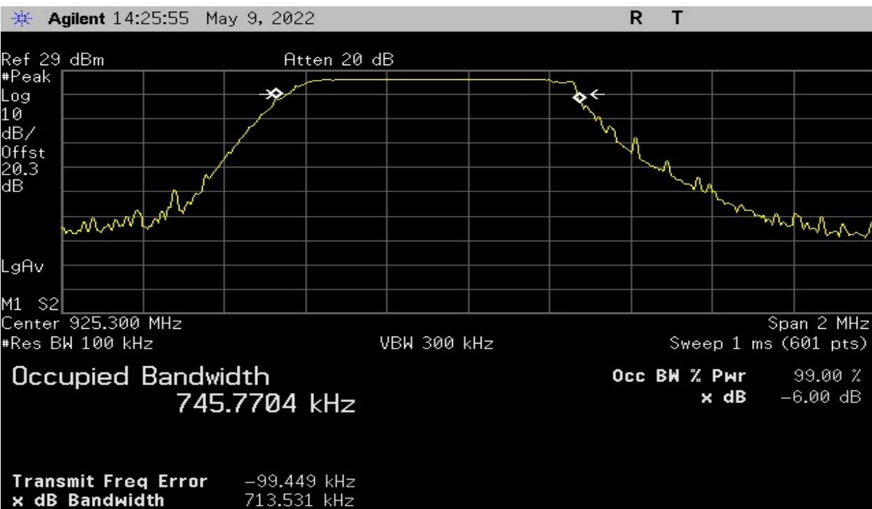
Plot 6 – Highest Channel – 6dB BW
