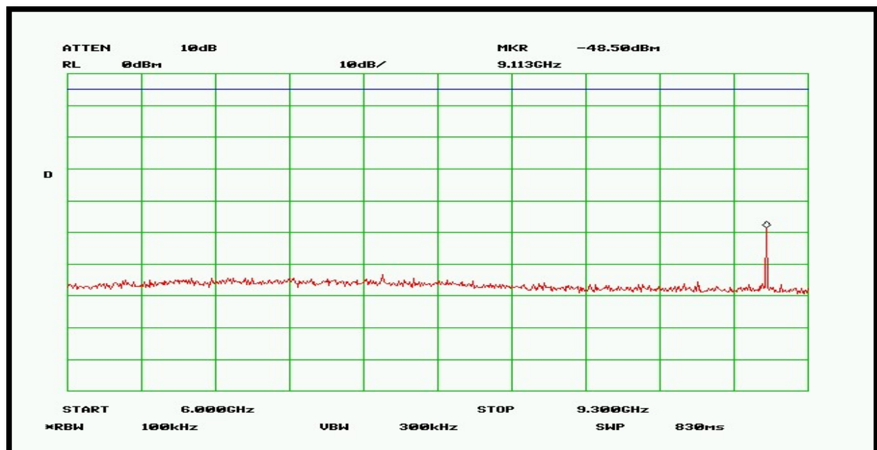
Plot 19 – High Band – 6GHz to 9.3GHz
