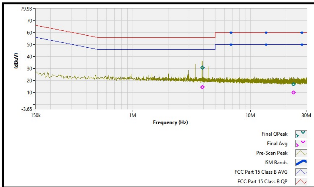
Plot 3 – Conducted Emissions – Neutral Side
