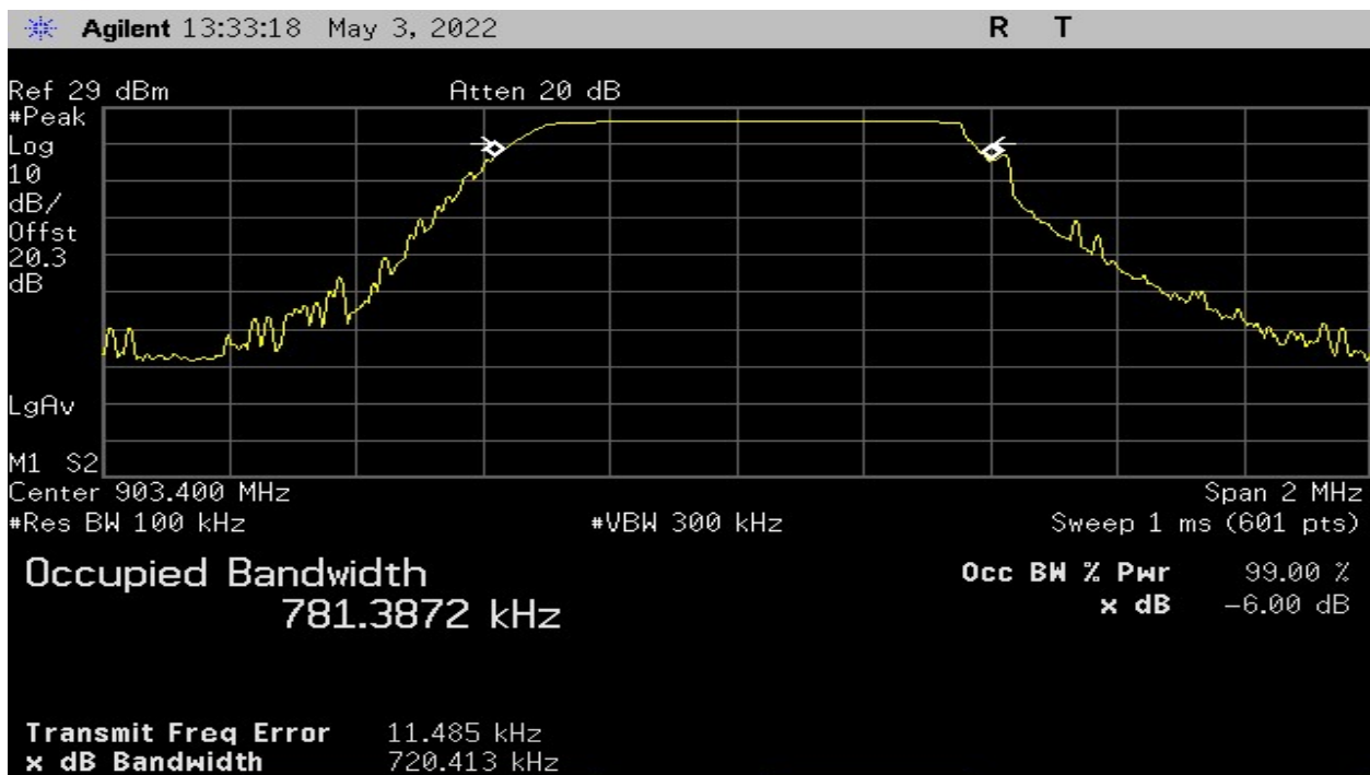
Plot 4 – Lowest Channel – 6dB BW
