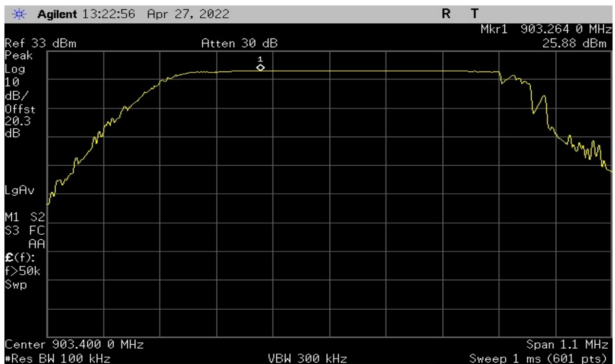
Plot 10 – Maximum in-band peak PSD in 100kHz
