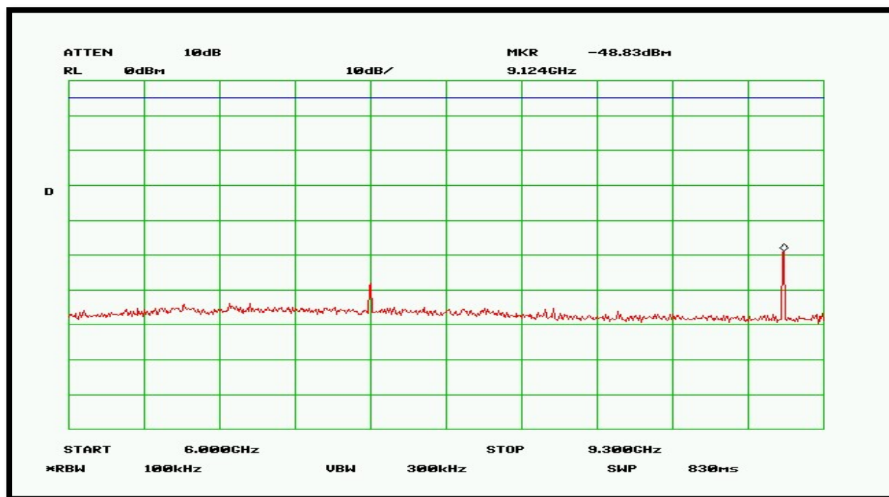
Plot 16 – Mid Band – 6GHz to 9.3GHz
