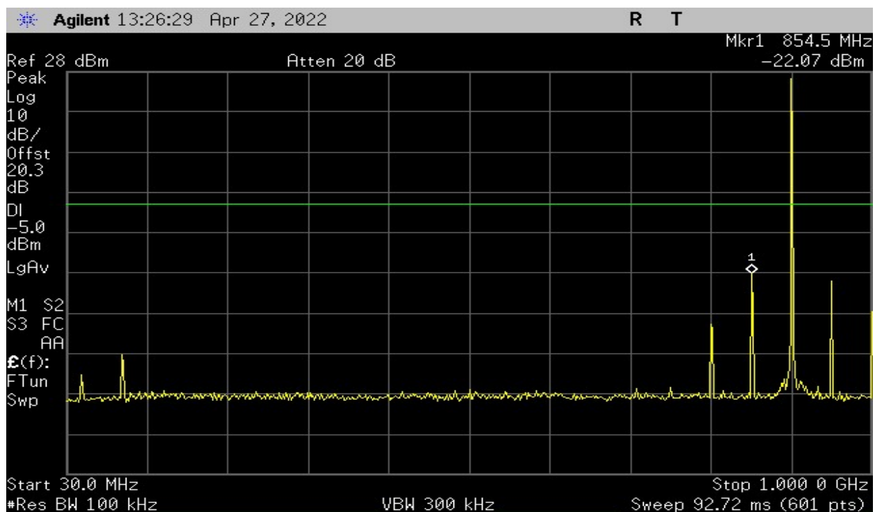
Plot 11 – Low Band – 30MHz to 1000MHz
