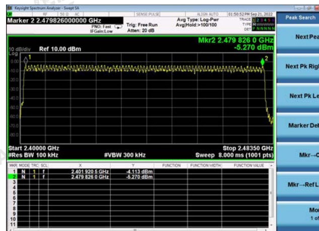
8-DPSK Modulation
