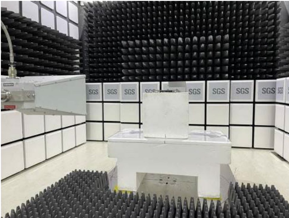
Radiated Emissions (Above 1GHz) Test Setup
