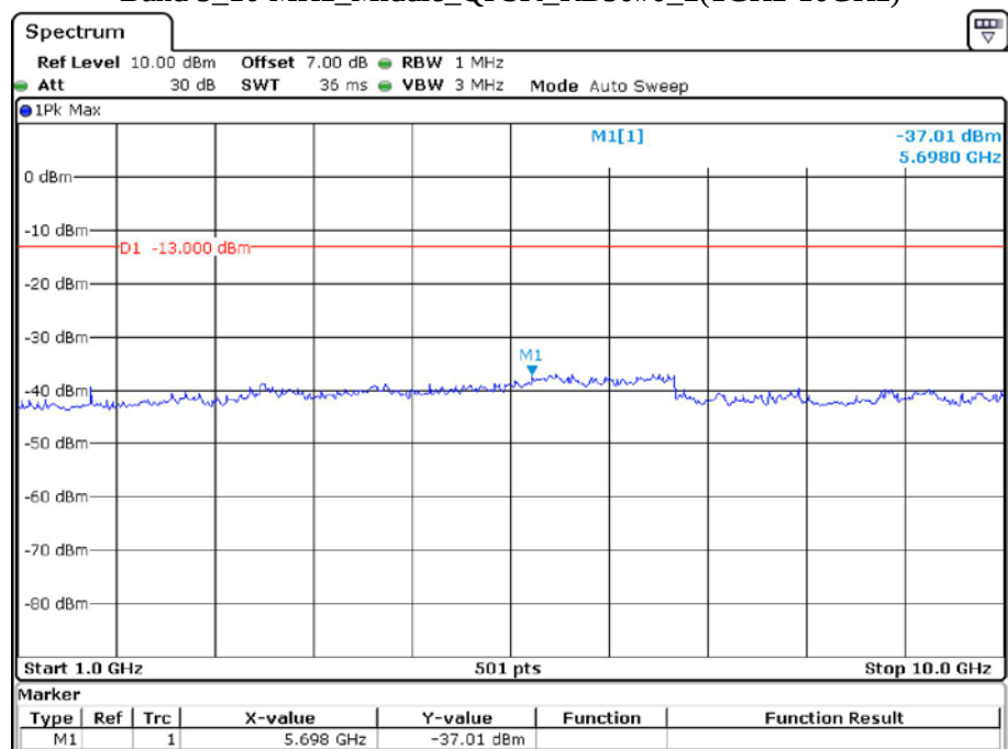
Band 5_10 MHz_Middle_QPSK_RB50#0_2(1GHz-10GHz)
