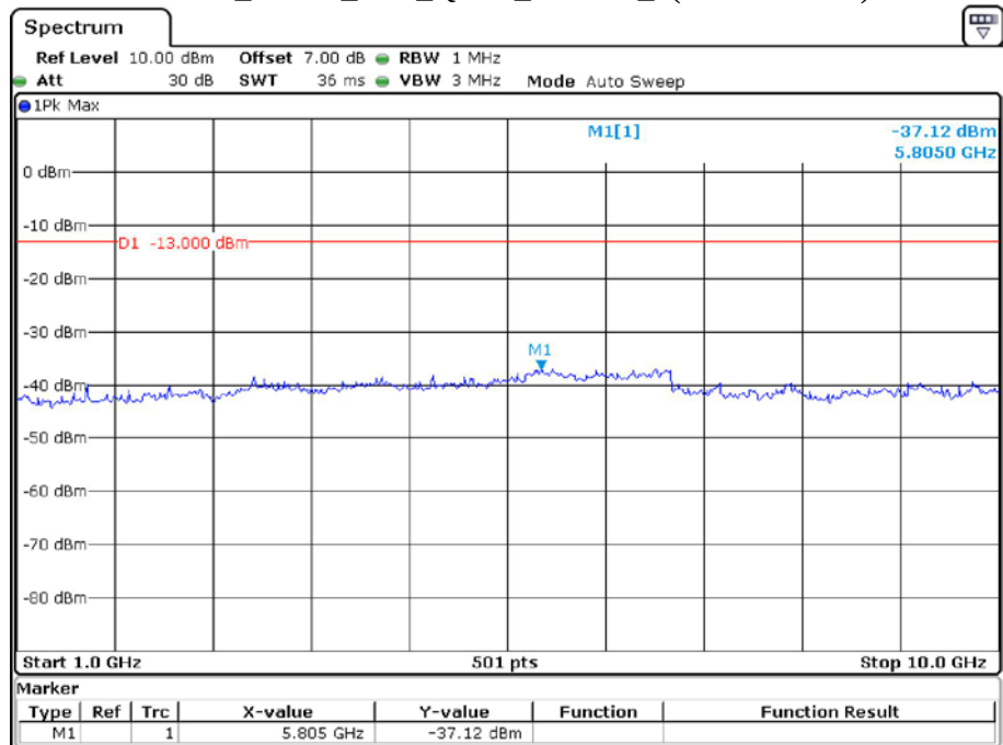
Band 5_5 MHz_Low_QPSK_RB25#0_2(1GHz-10GHz)
