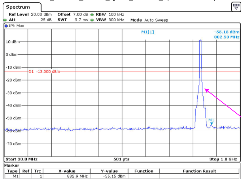
Band 5_10 MHz_Middle_QPSK_RB50#0_1(30MHz-1GHz)
