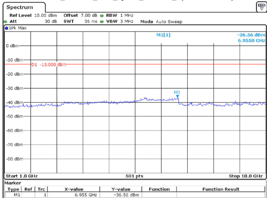
Band 5_10 MHz_Low_QPSK_RB50#0_2(1GHz-10GHz)
