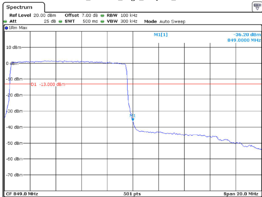
Band 5_10 MHz_High_16QAM_RB50#0
