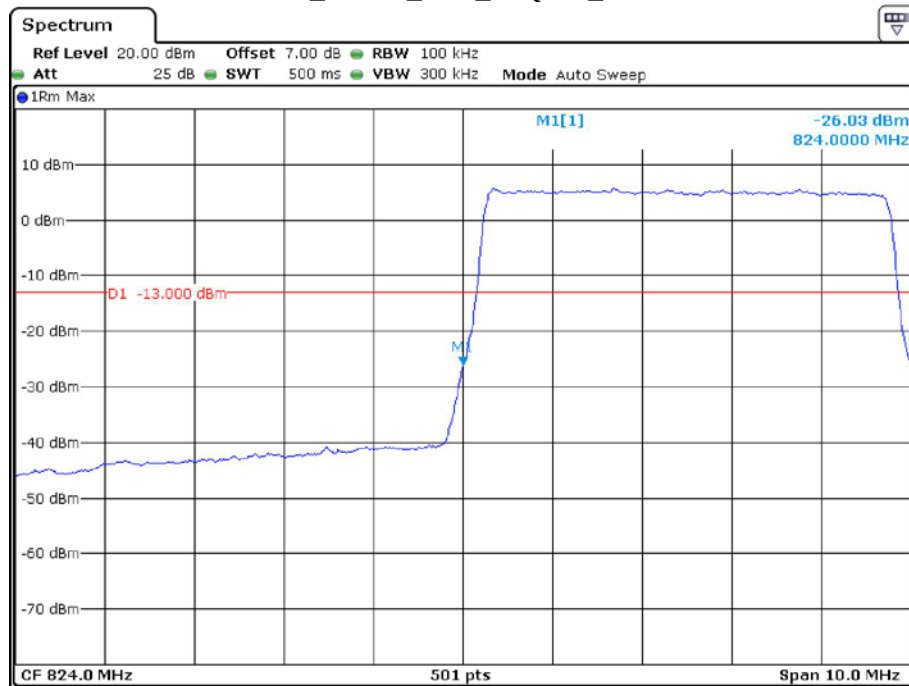
Band 5_5 MHz_Low_16QAM_RB25#0
