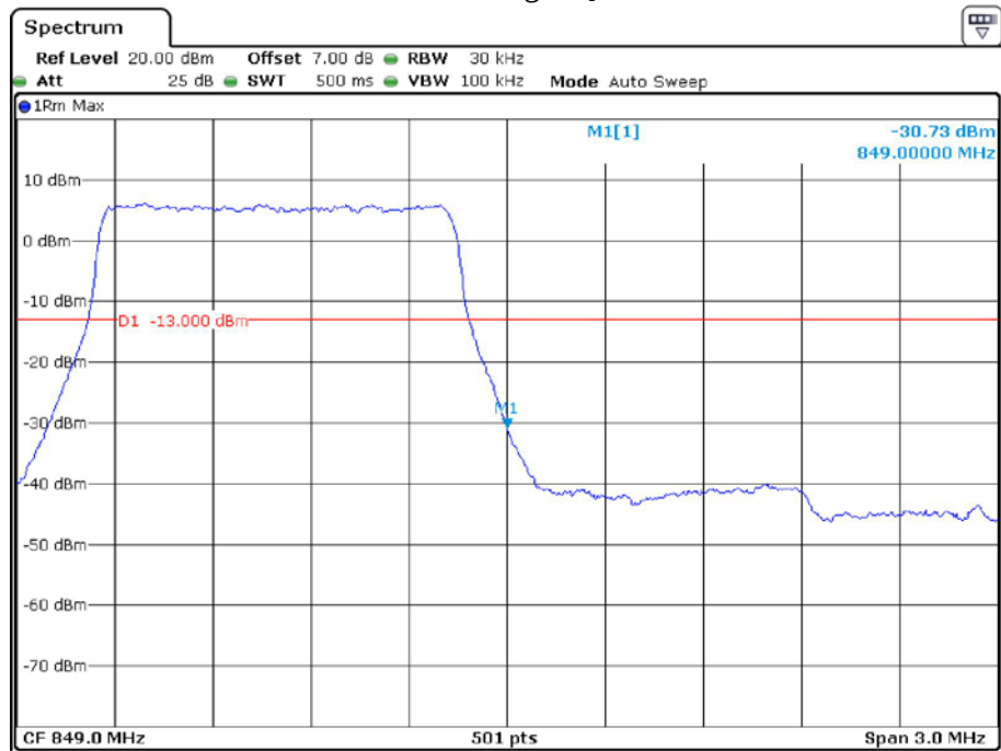
Band 5_1.4 MHz_High_QPSK_RB6#0
