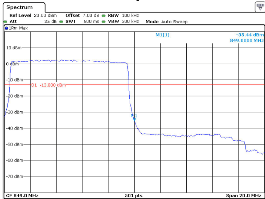
Band 5_10 MHz_High_QPSK_RB50#0
