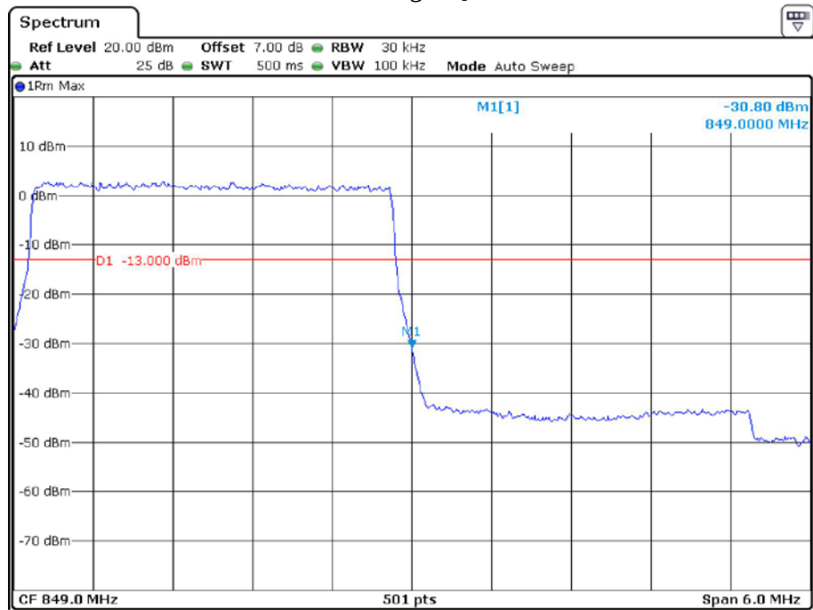
Band 5_3 MHz_High_QPSK_RB15#0
