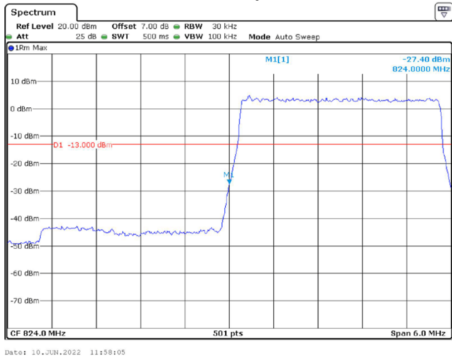
Band 5_3 MHz_Low_QPSK_RB15#0
