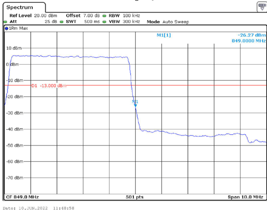
Band 5_5 MHz_High_QPSK_RB25#0
