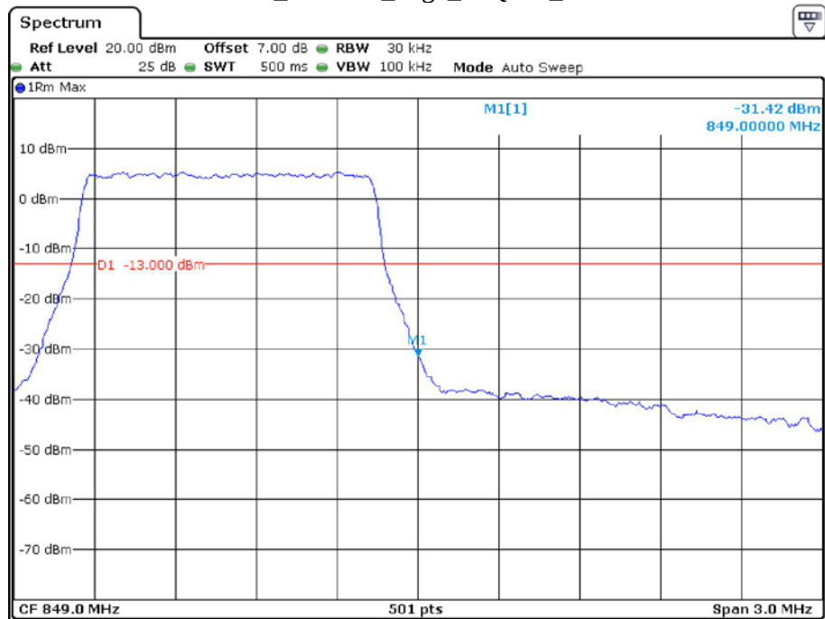
Band 5_1.4 MHz_High_16QAM_RB6#0
