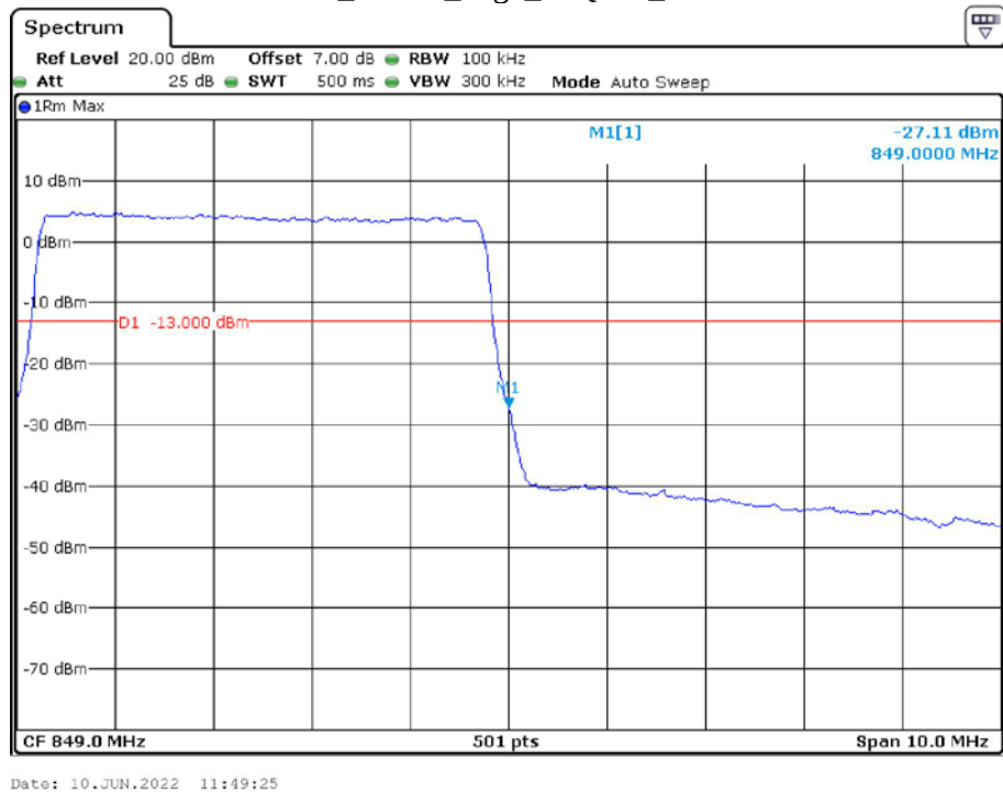
Band 5_5 MHz_High_16QAM_RB25#0
