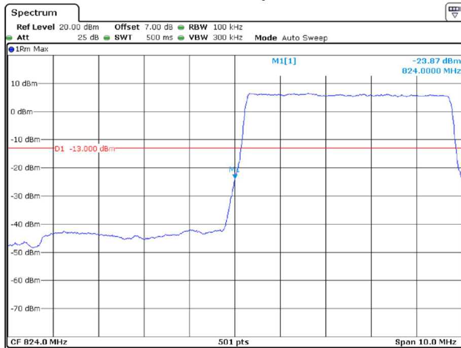
Band 5_5 MHz_Low_QPSK_RB25#0
