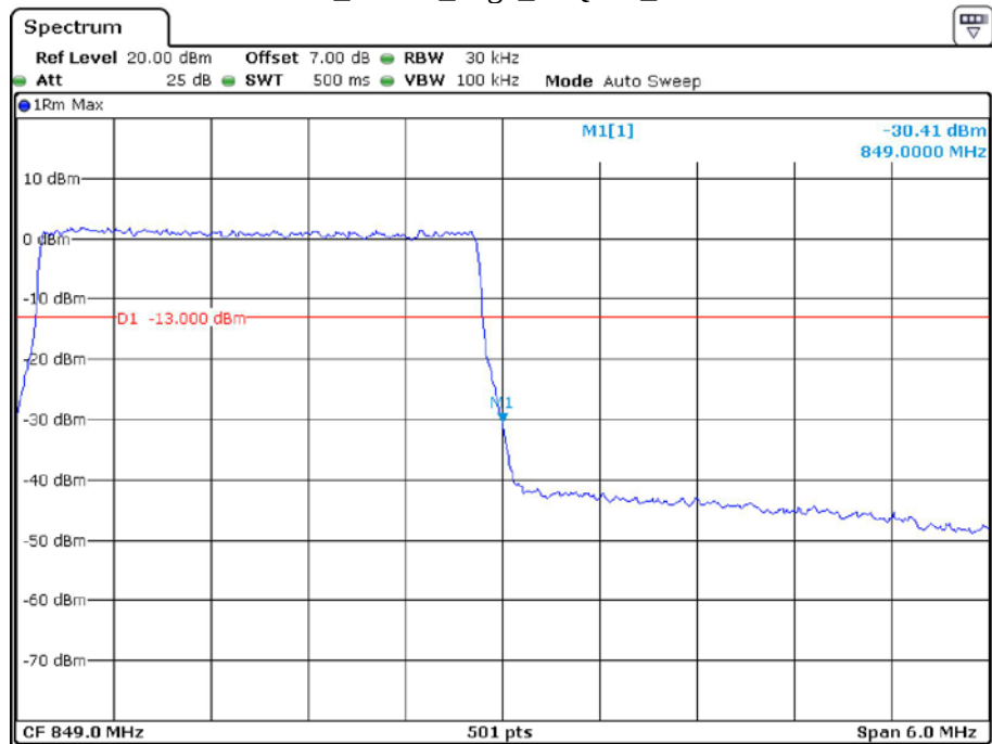
Band 5_3 MHz_High_16QAM_RB15#0
