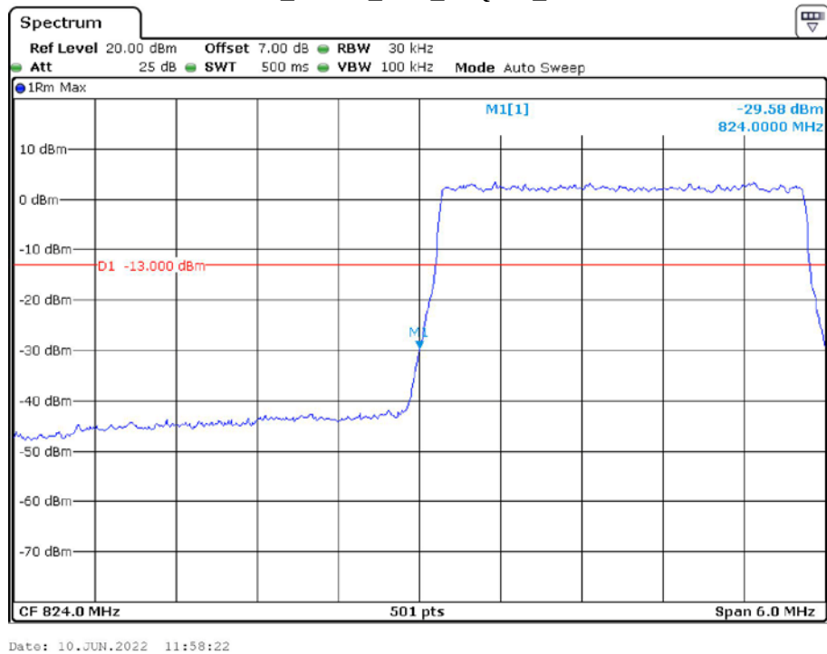
Band 5_3 MHz_Low_16QAM_RB15#0
