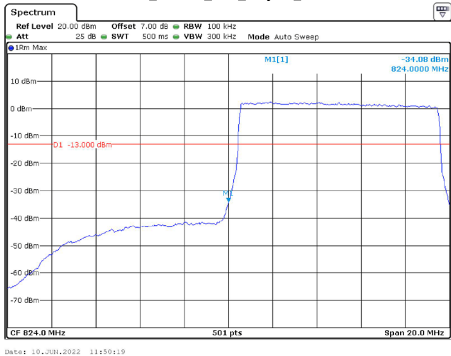
Band 5_10 MHz_Low_16QAM_RB50#0
