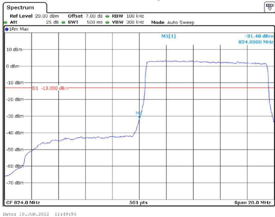
Band 5_10 MHz_Low_QPSK_RB50#0
