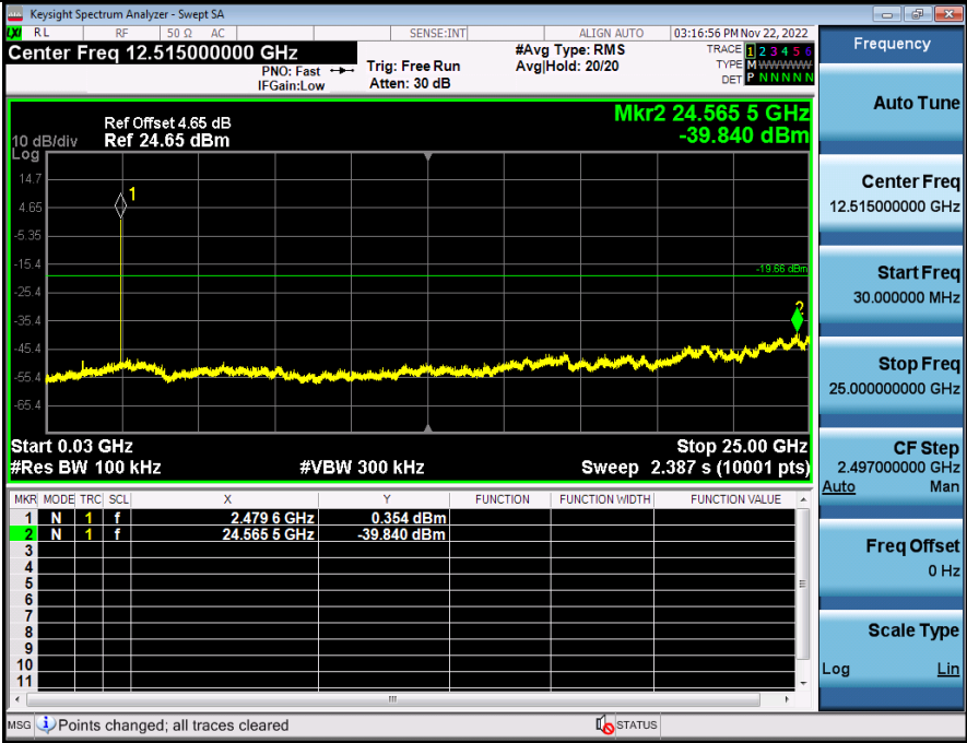
2_Spurious_Emissions_BT_2-DH5_2480
