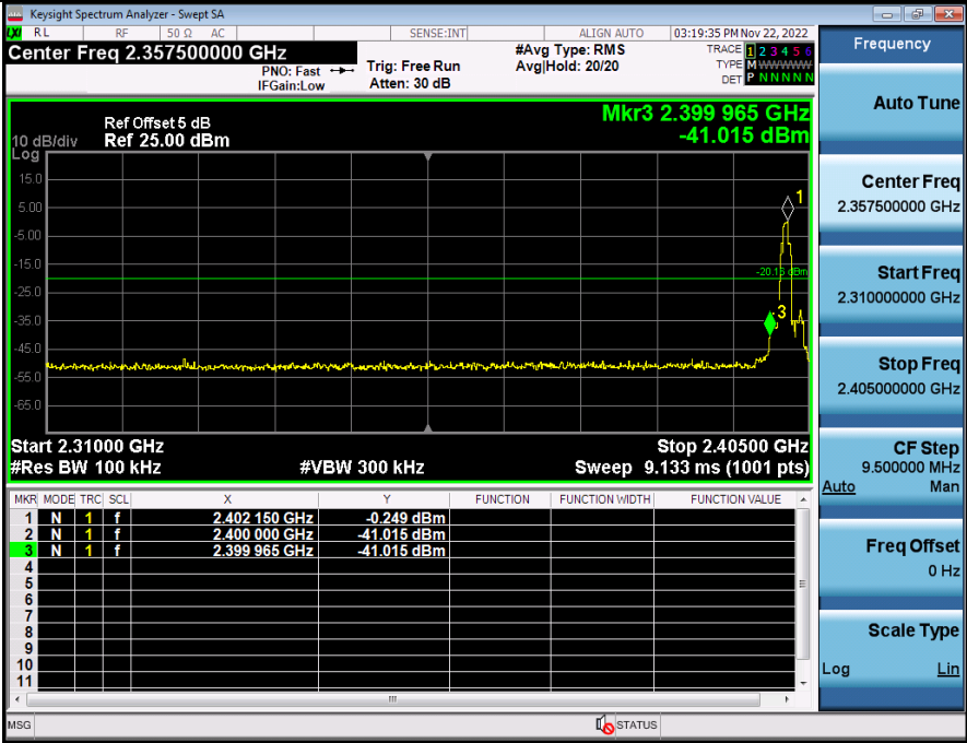
2_Bandedge_BT_3-DH5_2402
