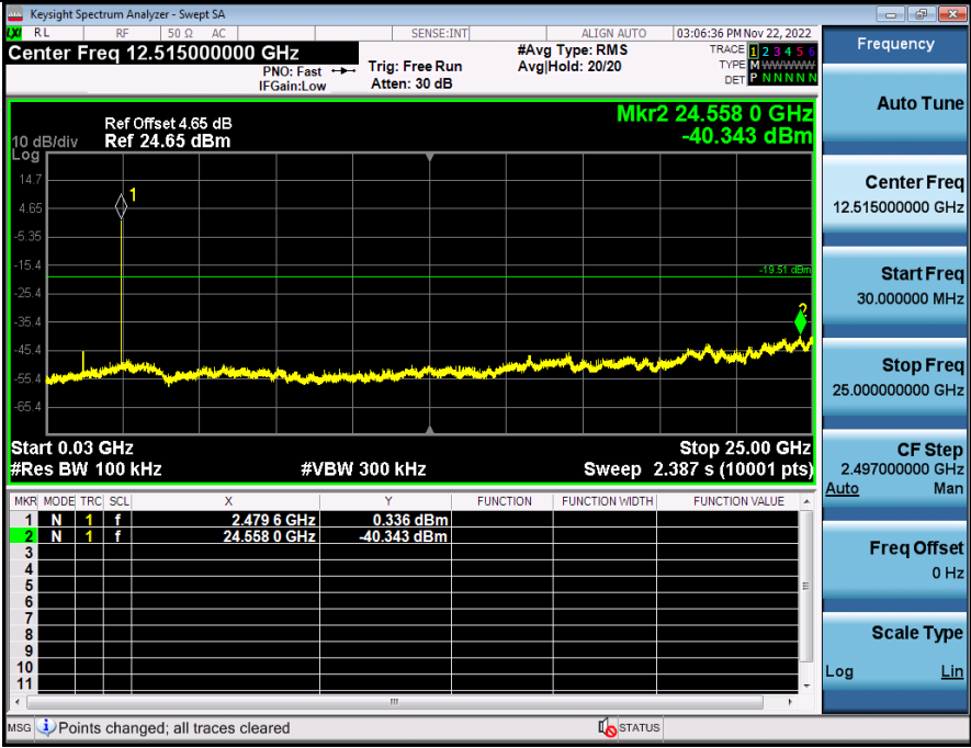
2_Spurious_Emissions_BT_1-DH5_2480
