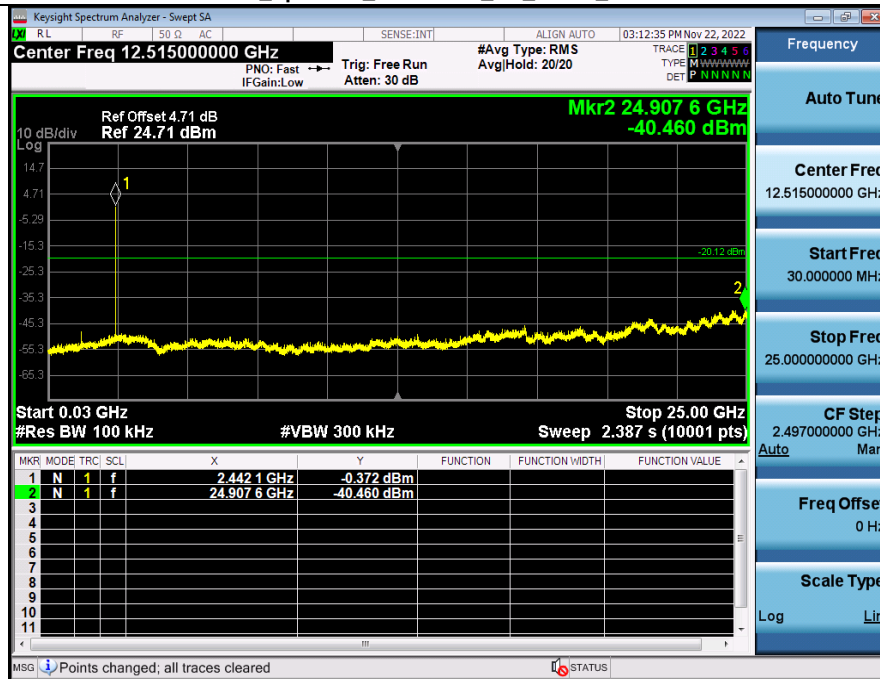
2_Spurious_Emissions_BT_2-DH5_2441
