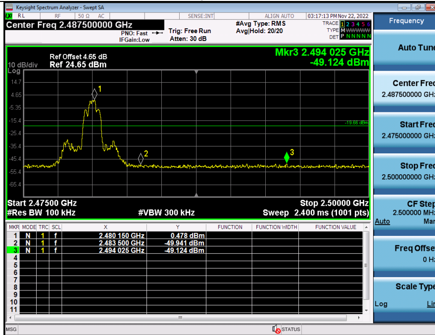
2_Bandedge_BT_2-DH5_2480
